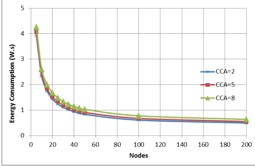
Figure 5-4: Impact of increasing the value of the contention window on the average energy consumption
