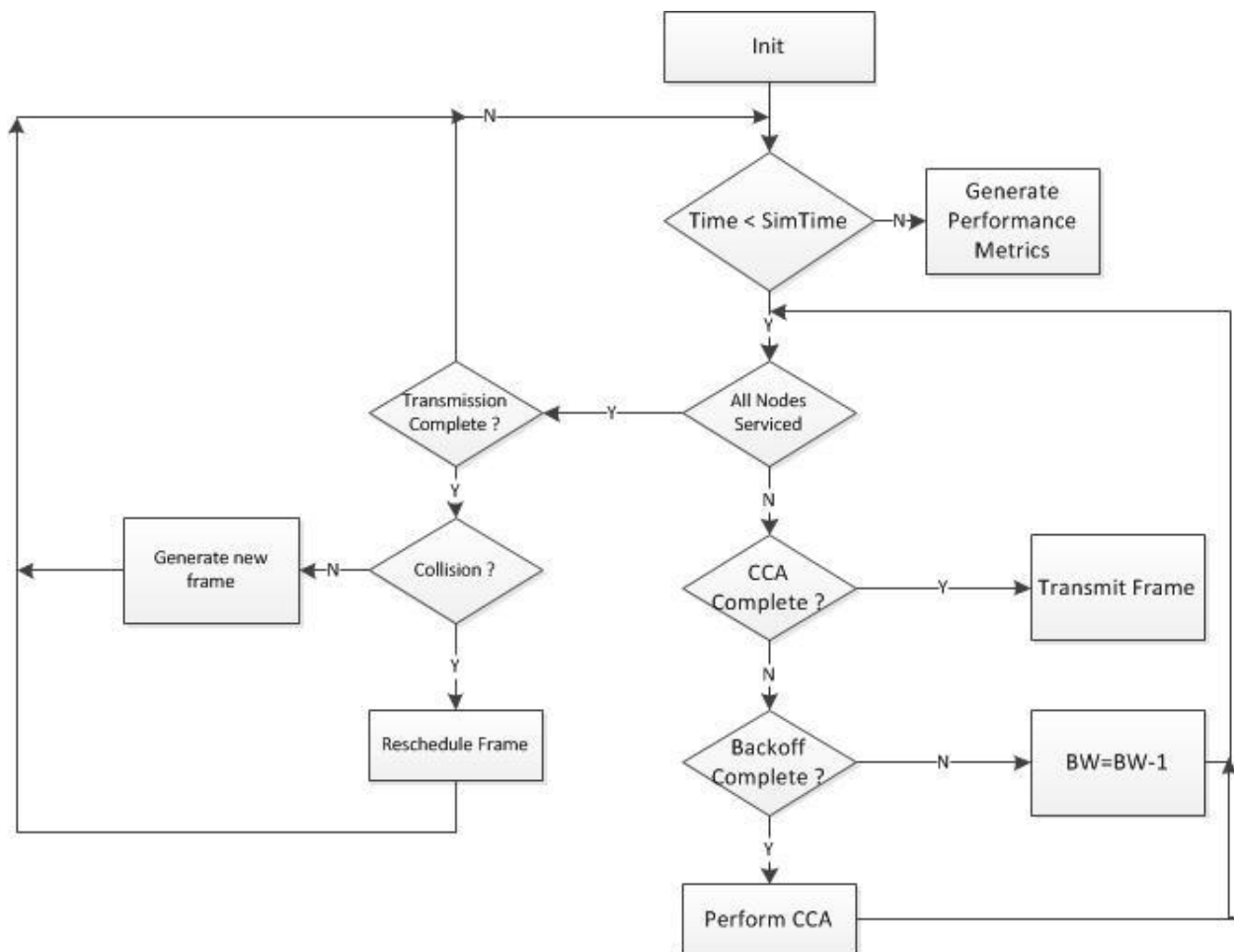
Figure 4-1: Flowchart of the MAC Simulator.
