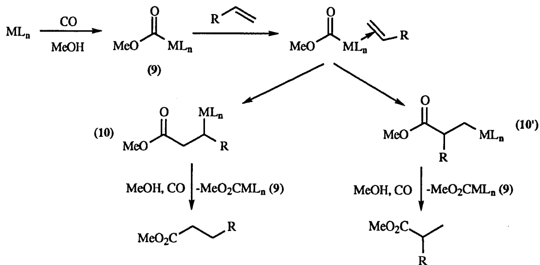
Scheme 5: Metal Carboxylate Mechanism for the Hydrocarboxylation Reaction.
