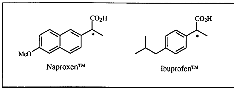
Chart 1: Aryl Propionic Acids with Analgesic Properties
