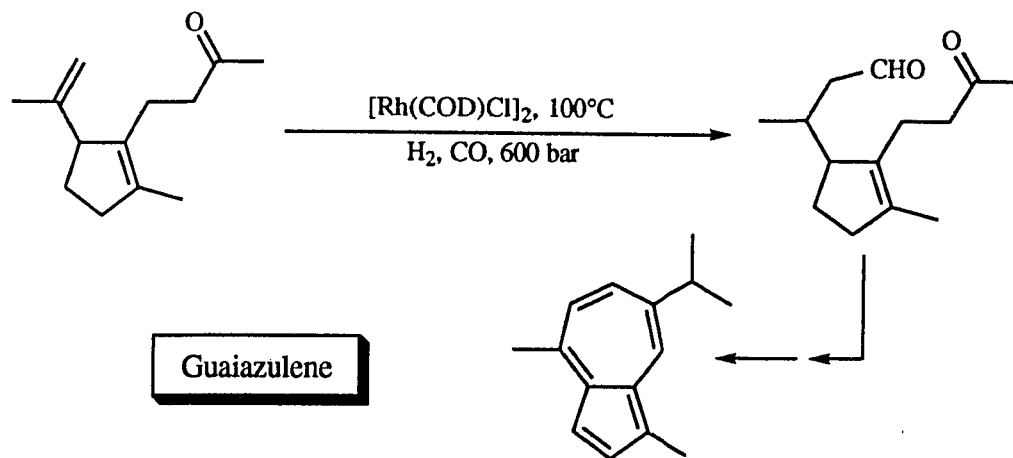
Scheme 12: Hydroformylation in the Preparation of Guaiazulene
