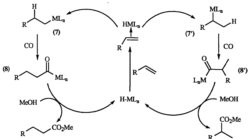
Scheme 4: Metal Hydride Mechanism for the Hydrocarboxylation Reaction.
