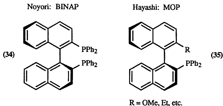
Figure 6: Binap and MOP: Effective Axially Dissymmetric Ligands.
