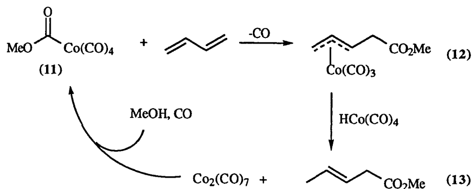
Scheme 6: Cobalt Methoxylate Catalyzed Hydroesterification of Butadiene.
