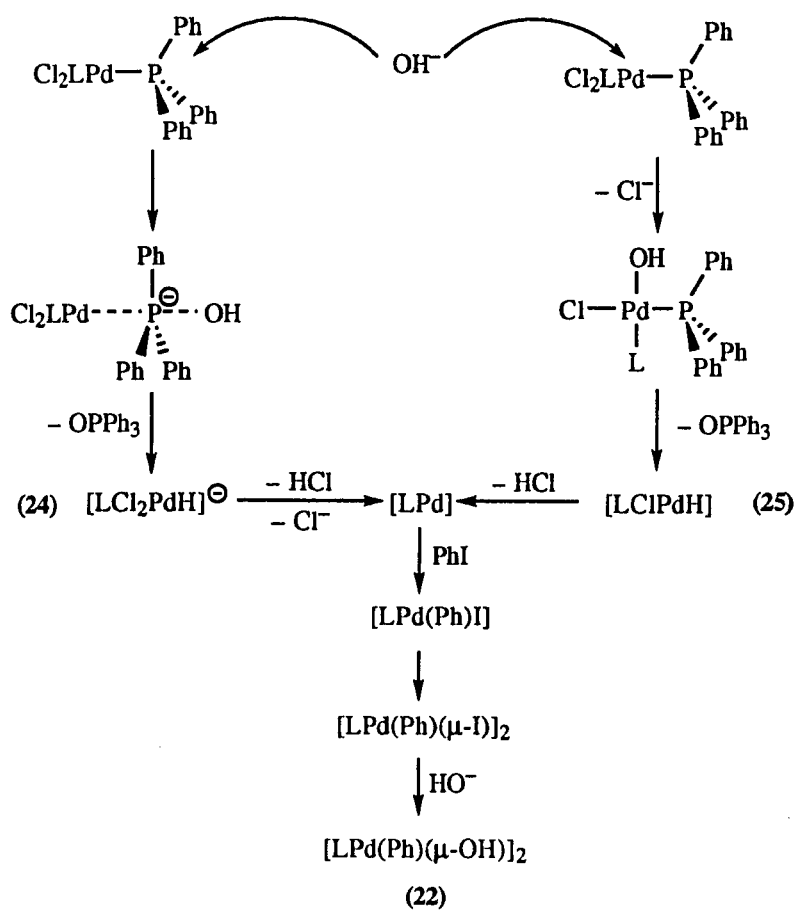
Scheme 10: The Hydroxide-Promoted Reduction of Pd(II) Phosphine Complexes
