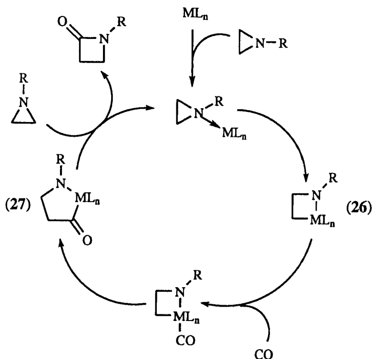
Scheme 11: \beta -Lactams From Aziridines: Carbonylative Ring Expansion.
