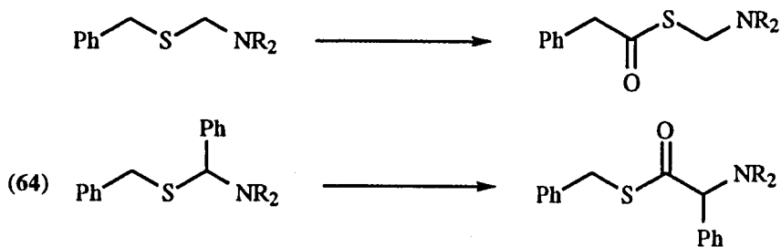
Scheme 17: Regioselectivity of Carbonylation of Acyclic N,S-Acetals
