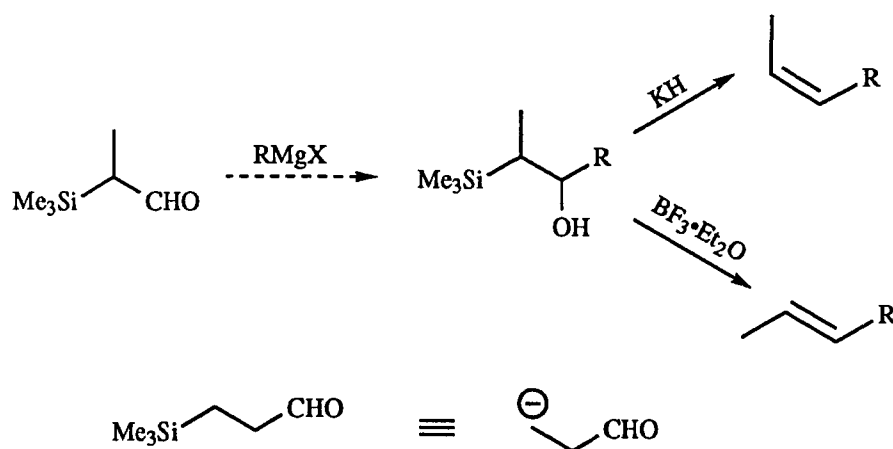
Scheme 14: The Utility of \alpha - and \beta -Silylaldehydes.
