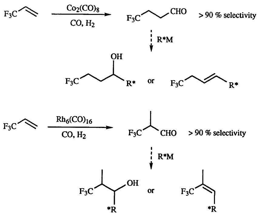
Scheme 13: Hydroformylation of Fluorinated Alkenes.
