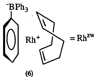
Figure 1: Structure of the Zwitterionic Complex Rh^{zw} .
