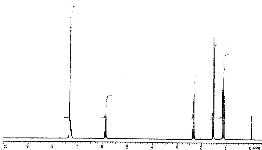
Figure 9: Ethyl Ester of (S)-(-)-1-Phenylethanol (42).
