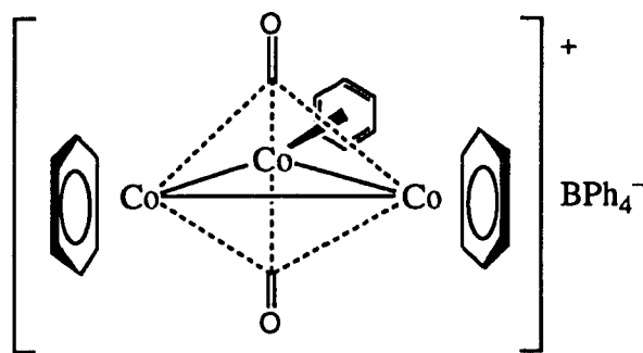
Figure 5: [\text{Co}_3(\eta^6\text{-C}_6\text{H}_6)_3(\mu_3\text{-CO})_2]\text{BPh}_4^- , (34).
