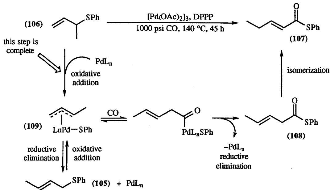
Scheme 22: Palladium Catalyzed Carbonylation of 3-(1-Butenyl) Phenyl Sulfide.
