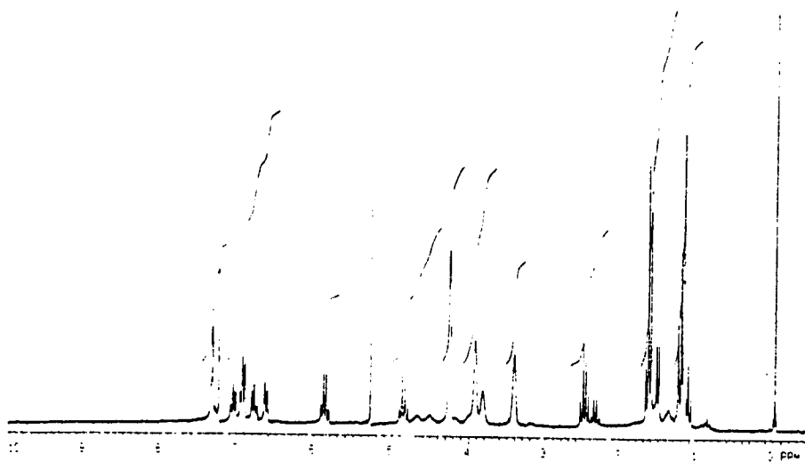
Figure 10: Preparation of Chiral-Non Racemic Rhodium-Arene Ester Complex (43).
