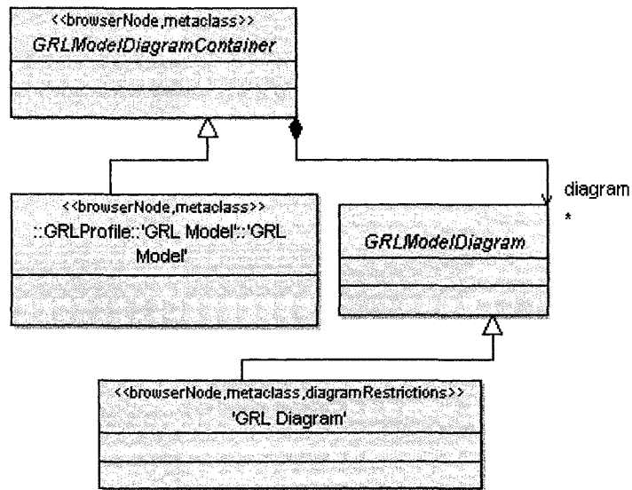
Figure 55 GRL Editor Package (1)
