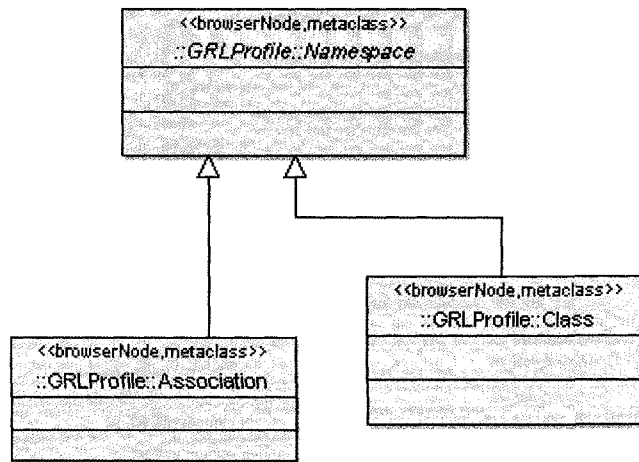
Figure 54 GRL Model Package (4)
