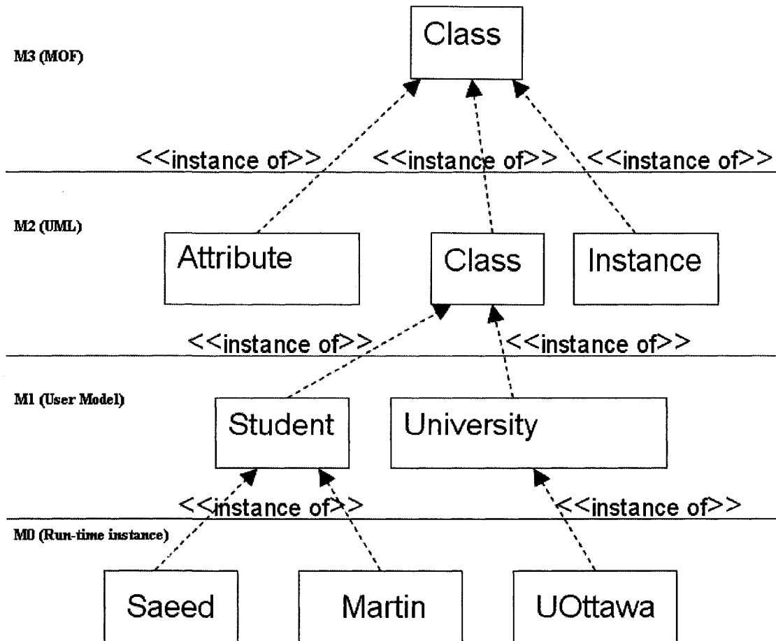
Figure 3 Four Layers of Metamodel
