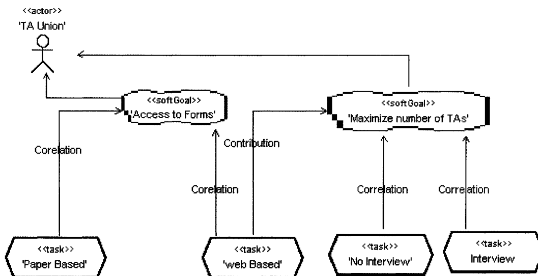
Figure 74 TA Union, Modelled with Tau GRL Profile
