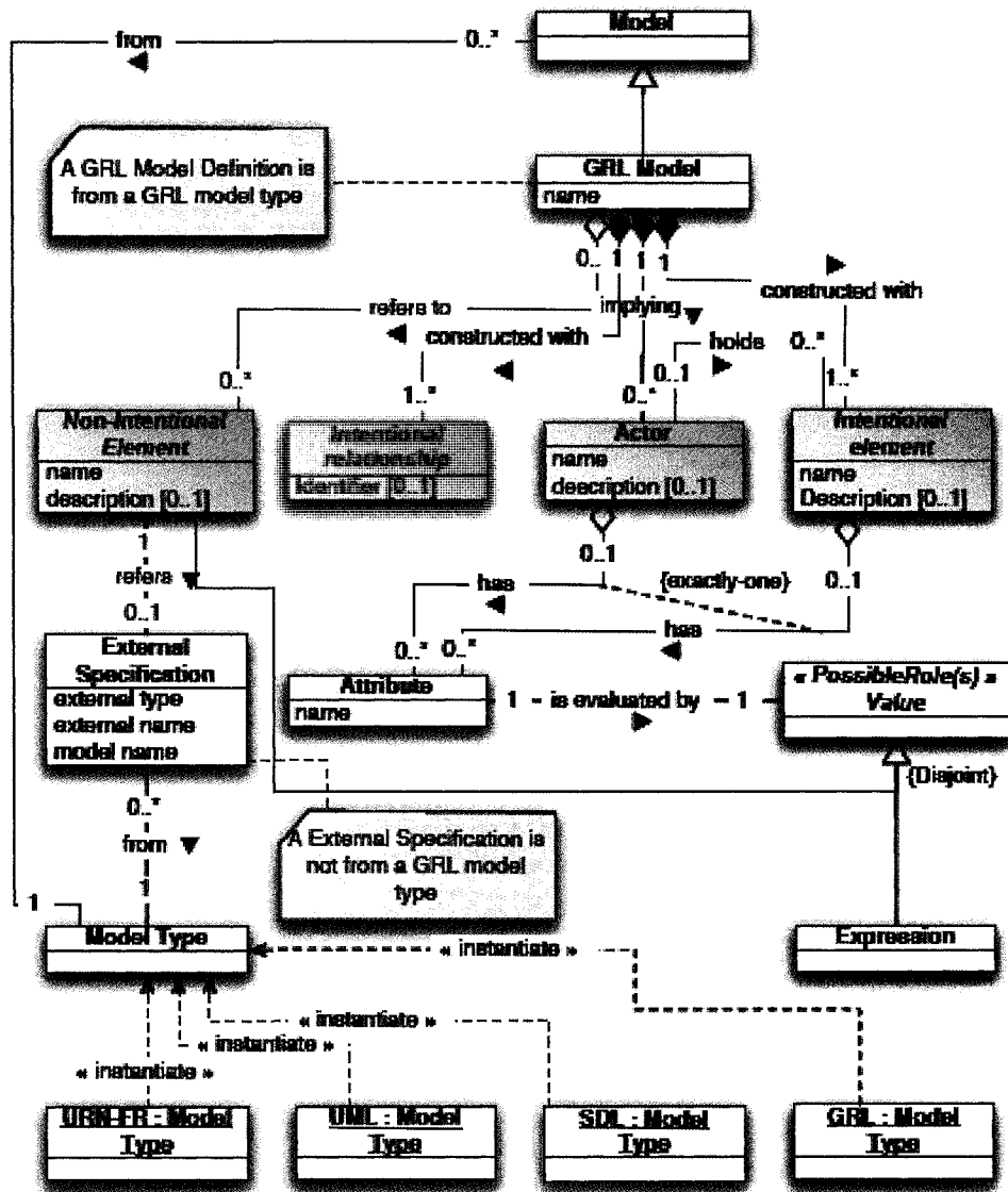
Figure 14 Top Level View of GRL Metamodel [6]
