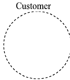
Figure 24 Actor
