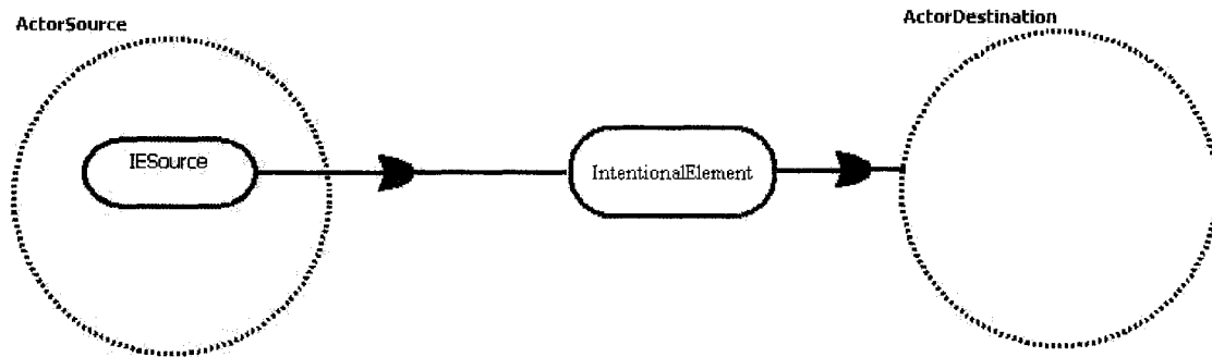
Figure 40 Dependency Scenario 3
