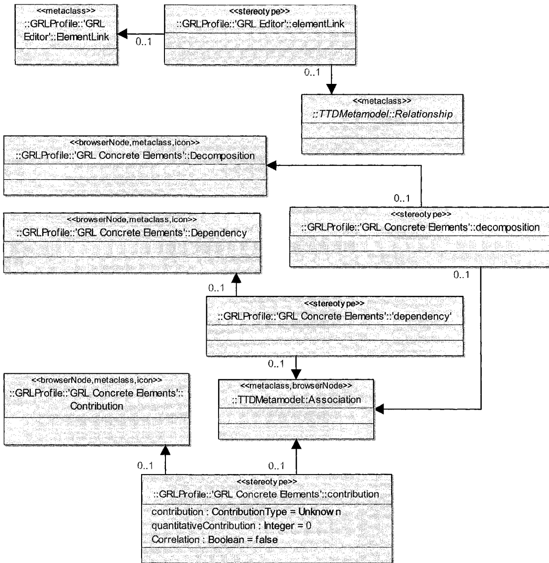
Figure 61 GRL Abstract Elements Package (1)
