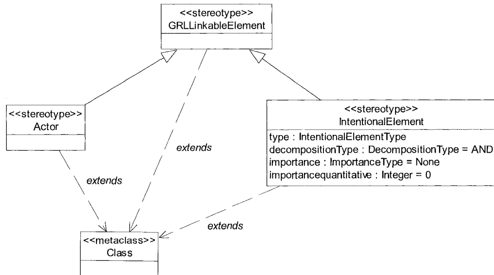
Figure 46 GRL Linkable Element
