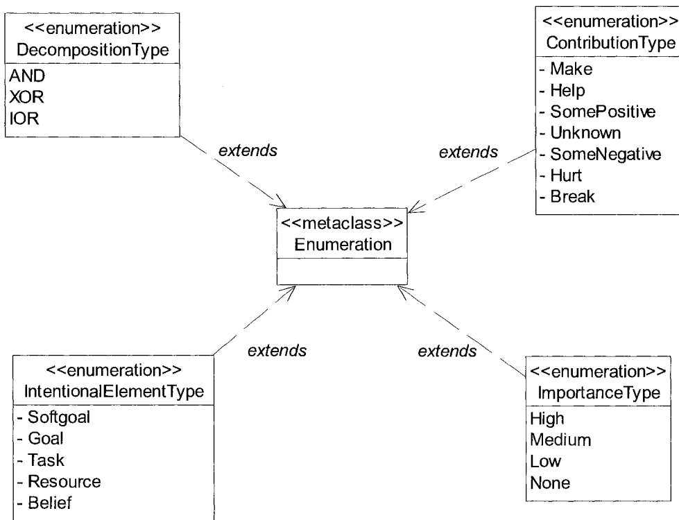
Figure 48 Enumerations
