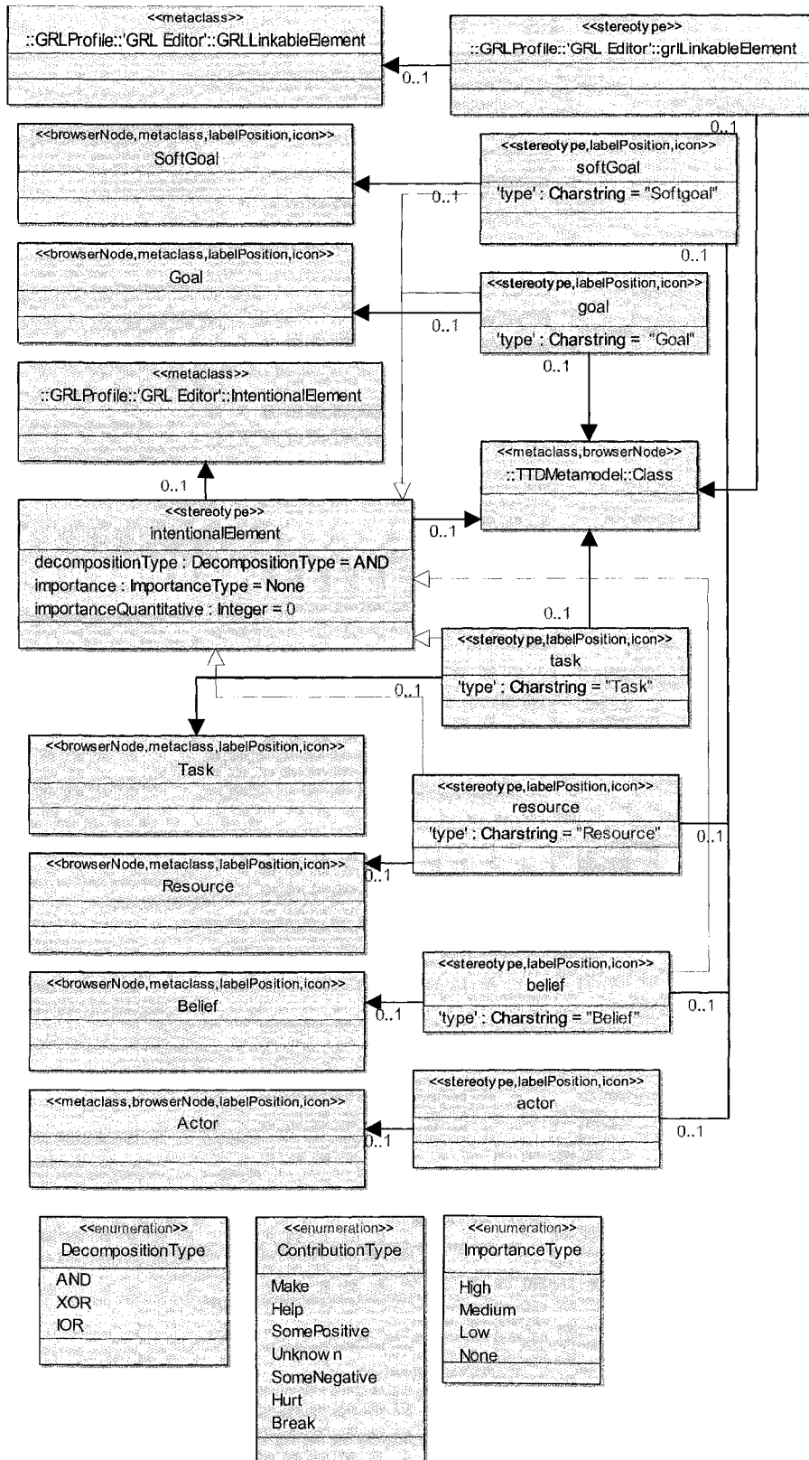
Figure 62 GRL Abstract Elements Package (2)
