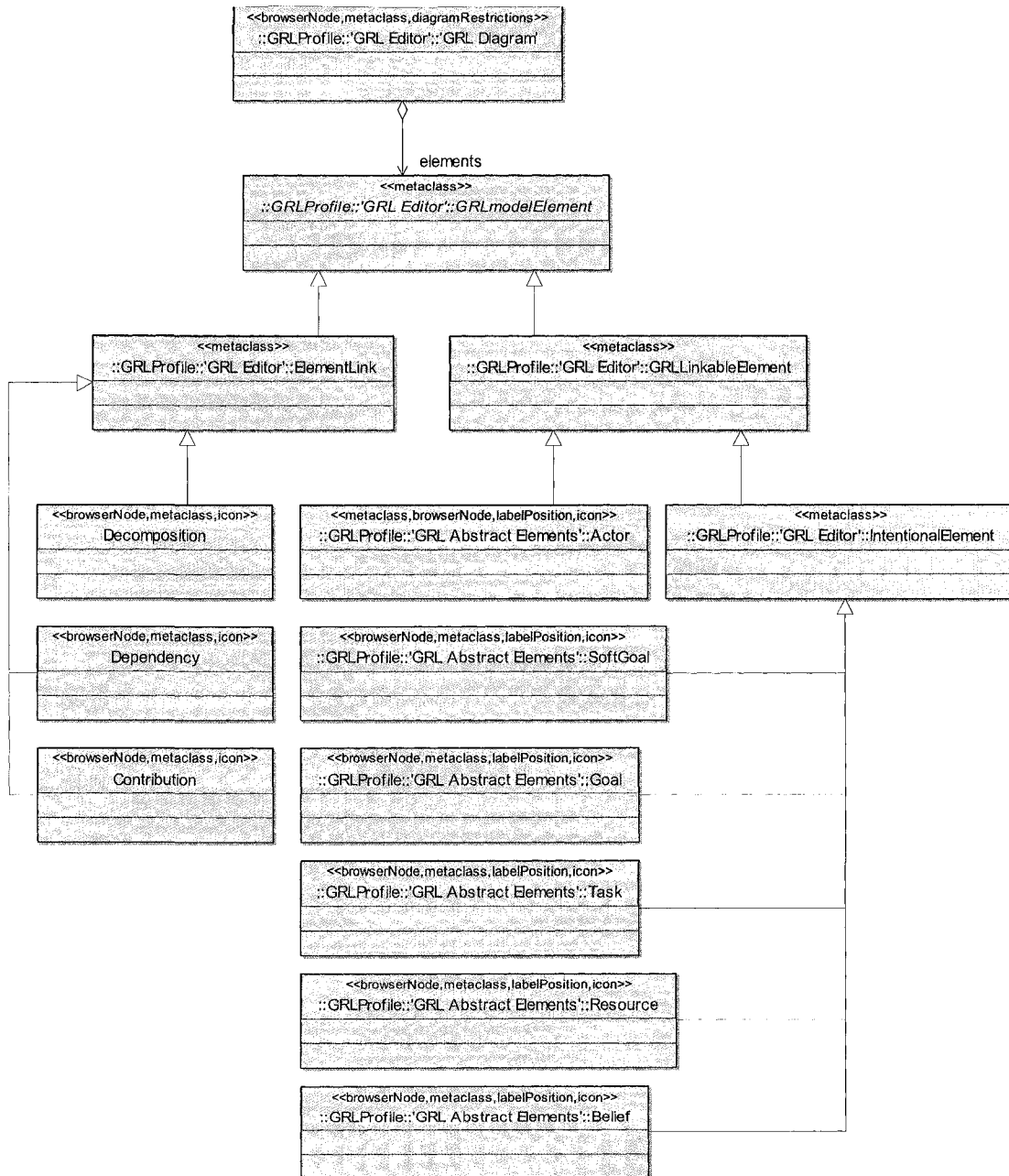
Figure 59 GRL Concrete Elements Package (1)
