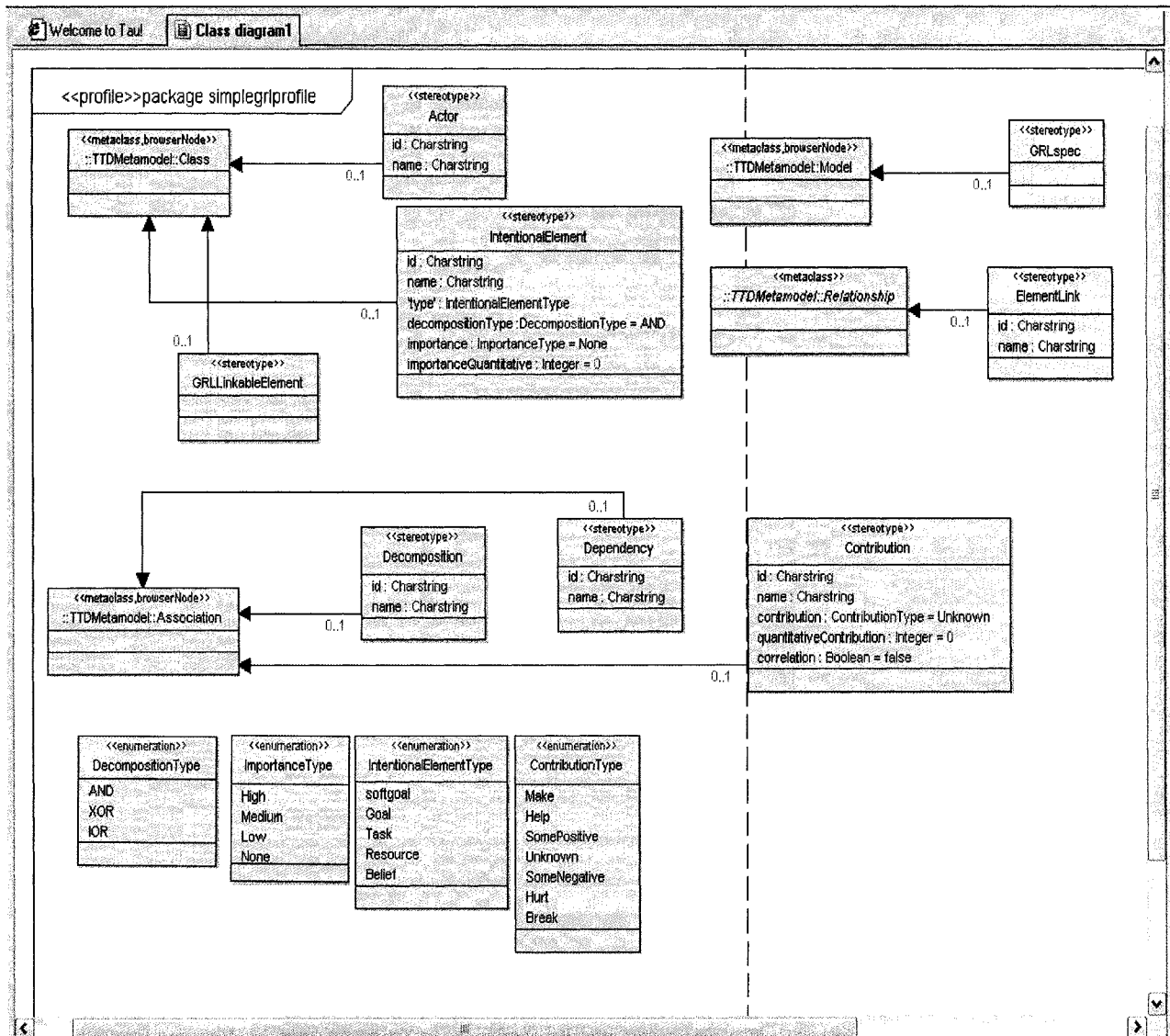
Figure 50 GRL Profile by Stereotype Mechanism (1)
