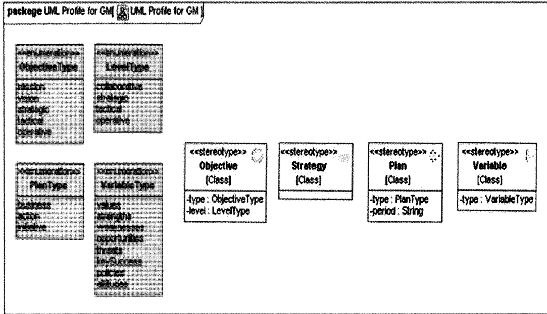
Figure 20 Diagram of the UML Profile for Enterprise Goal Modelling [9]
