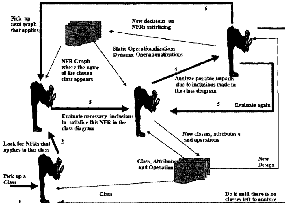
Figure 23 The Class Diagram Integration Process [5]
