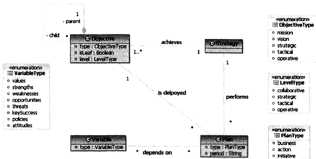
Figure 19 Goal Metamodel: Organizational Metamodel Excerpt [9]
