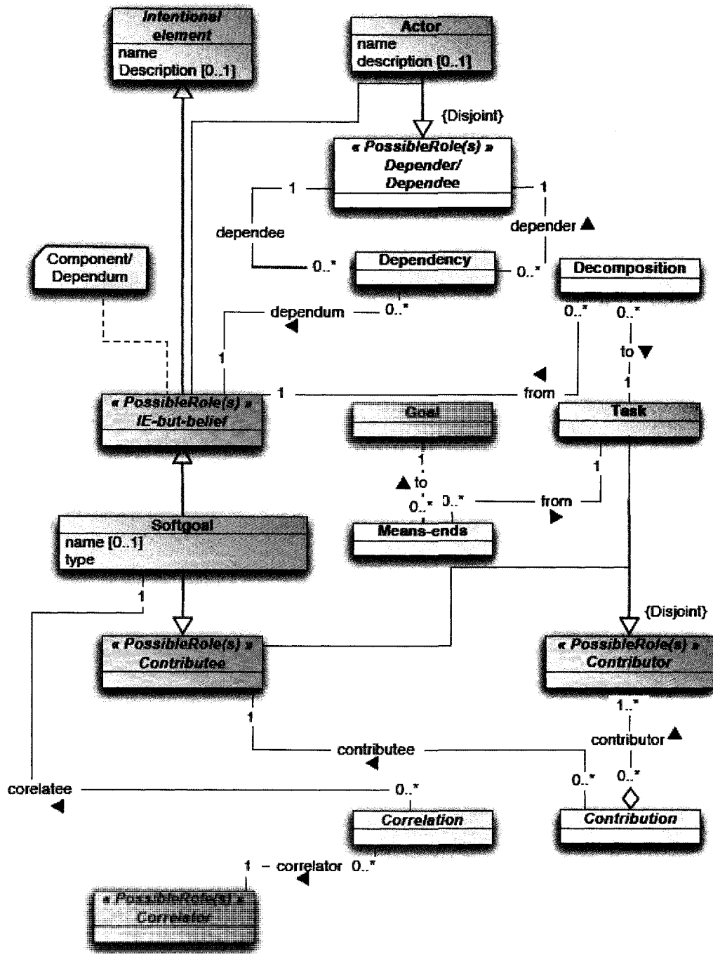
Figure 17 GRL Metamodel: Zoom on Intentional Relationships [6]
