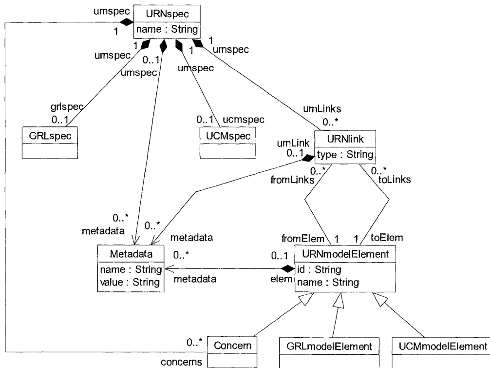
Figure 8 High-Level Overview of the URN Metamodel (Z.151)
