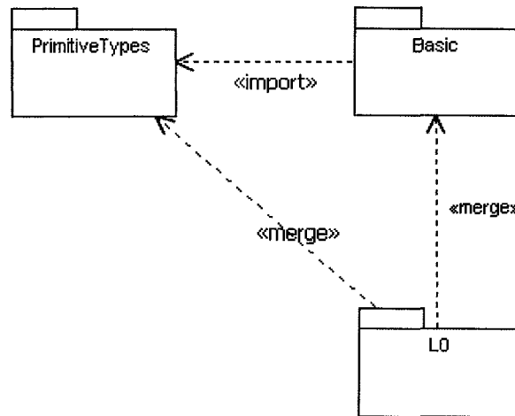
Figure 4 Level 0 (UML Superstructure)
