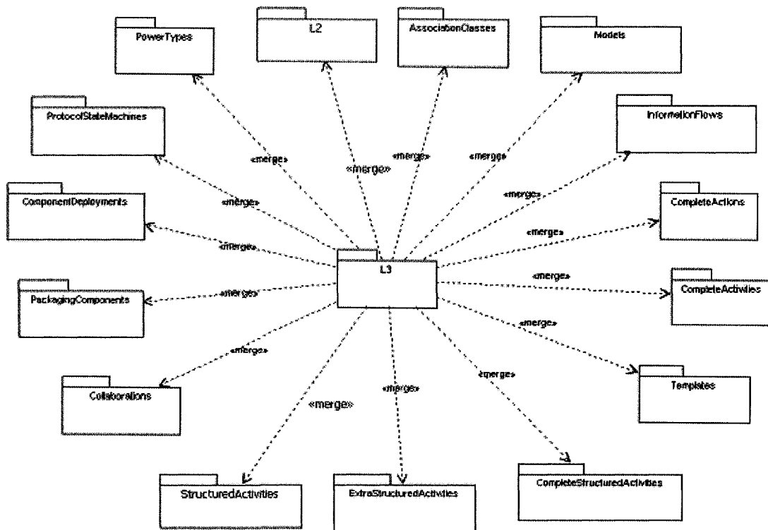
Figure 7 Level 3 (UML Superstructure)
