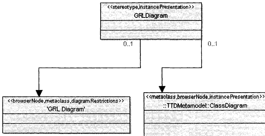
Figure 56 GRL Editor Package (2)
