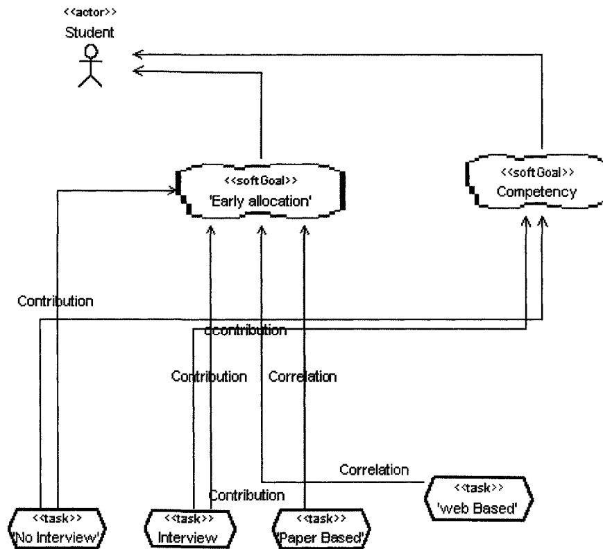
Figure 73 Student, Modelled with Tau GRL Profile
