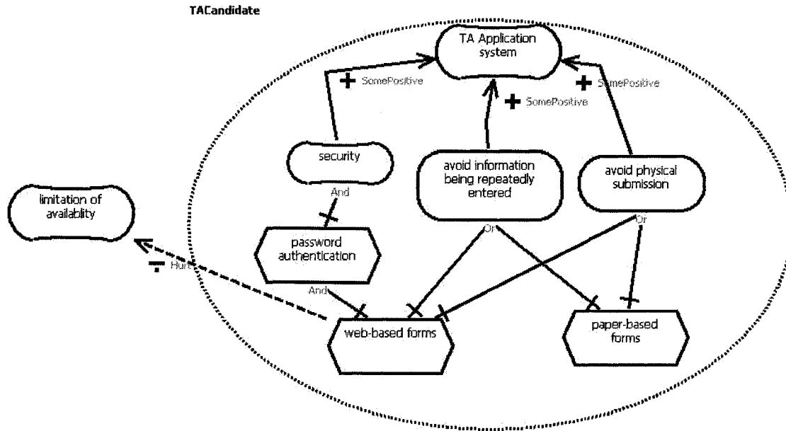
Figure 11 GRL Model Sample
