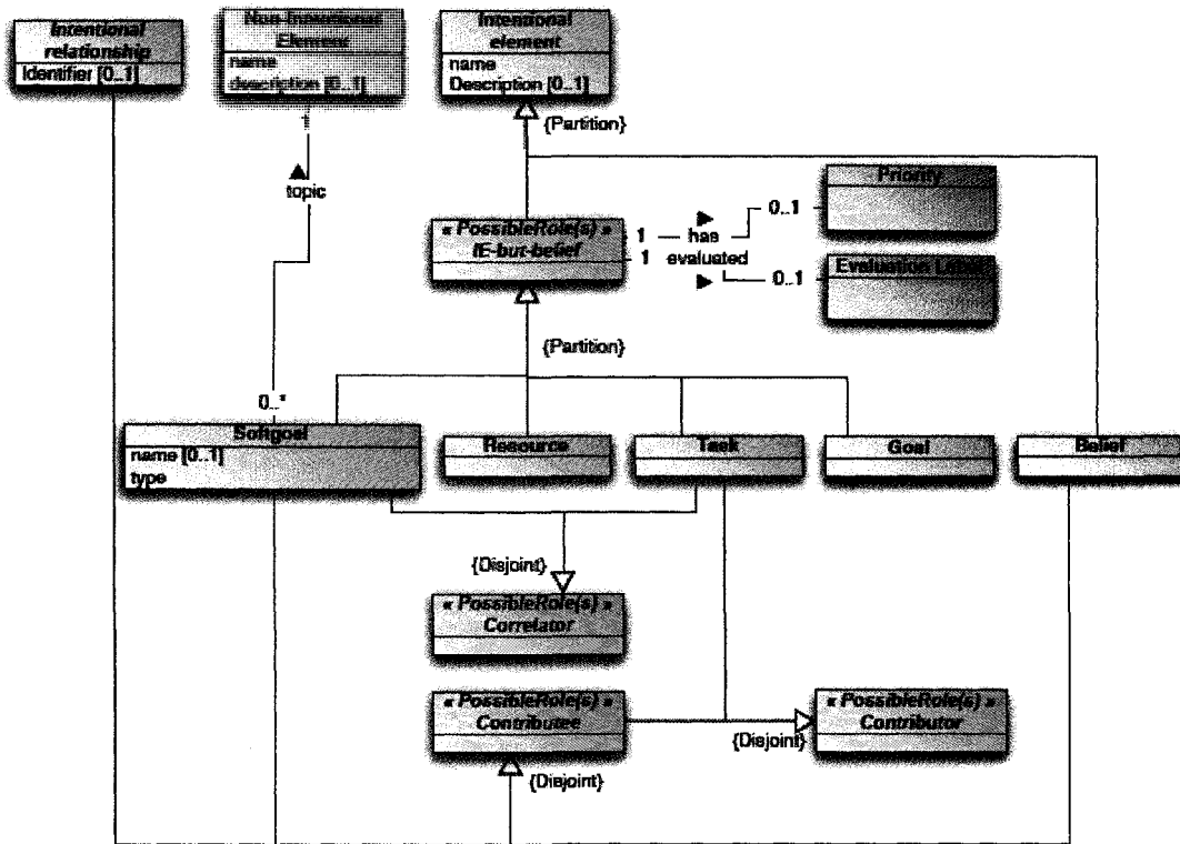
Figure 15 GRL Metamodel: Zoom on Intentional Elements [6]
