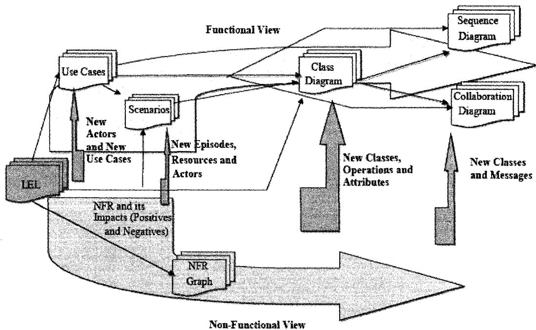
Figure 22 An Strategy Overview for Dealing with NFR [5]
