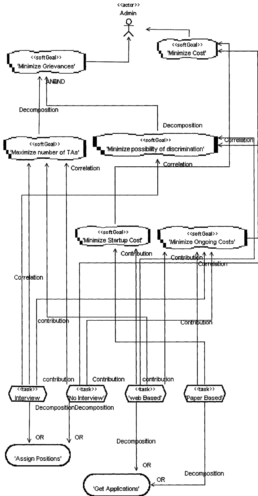
Figure 72 Admin, Modelled with Tau GRL Profile
