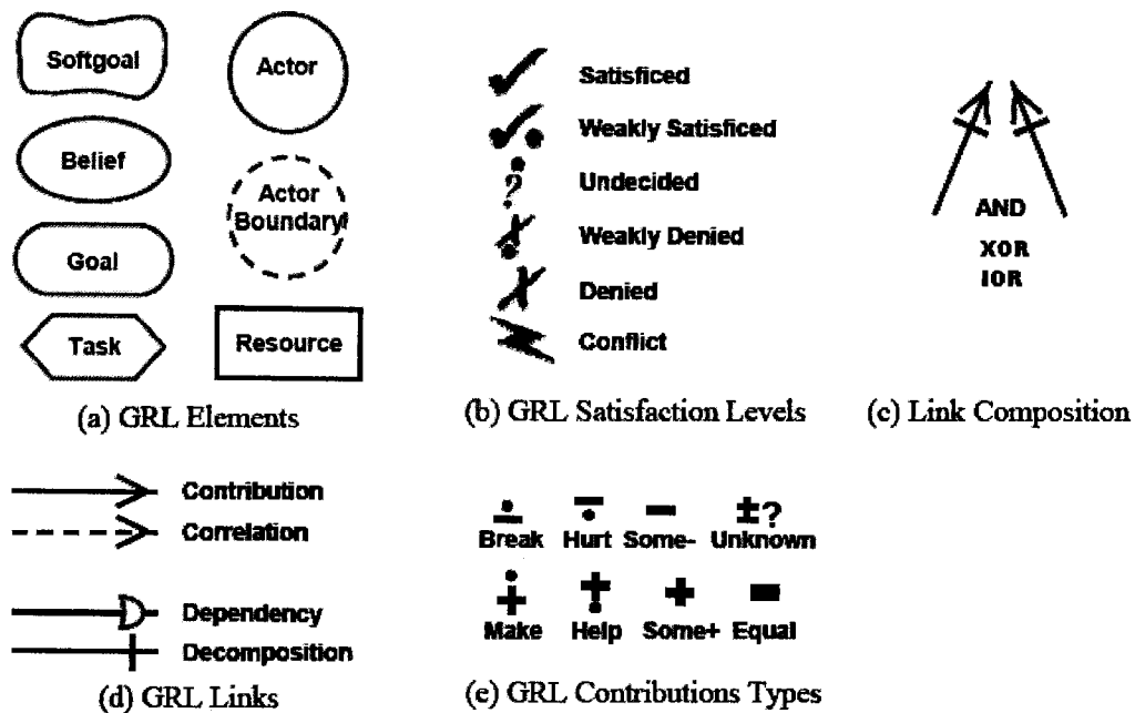
Figure 10 Summary of GRL Notations
