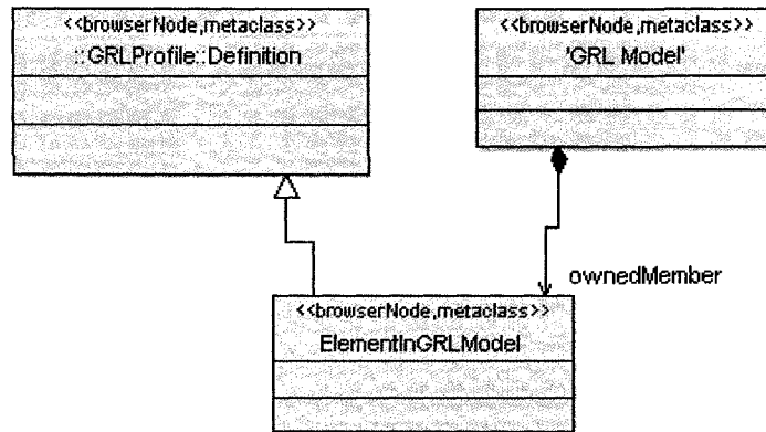
Figure 53 GRL Model Package (3)
