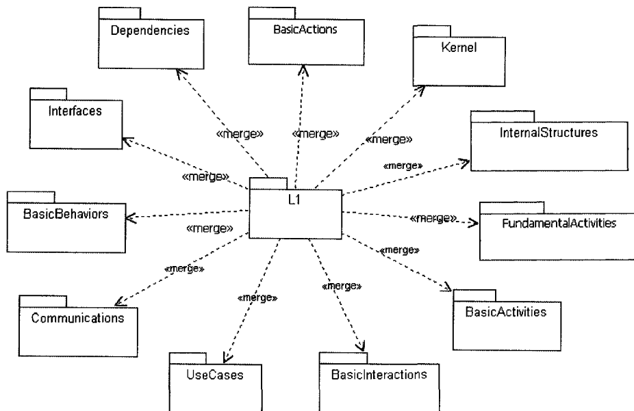
Figure 5 Level 1 (UML Superstructure)
