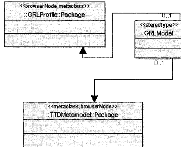
Figure 51 GRL Model Package (1)
