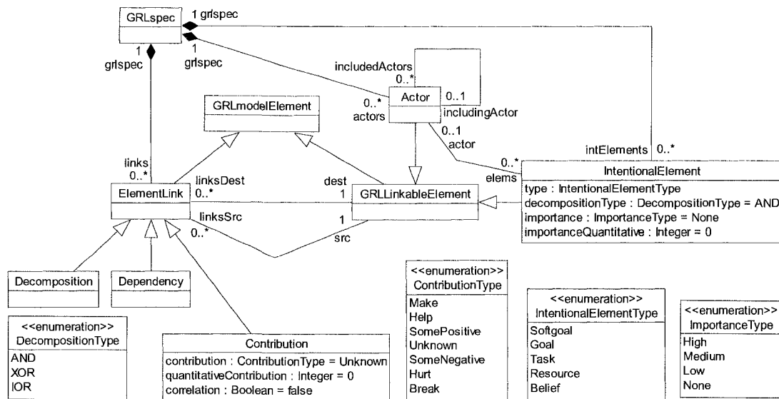
Figure 13 Metamodel of GRL [17]
