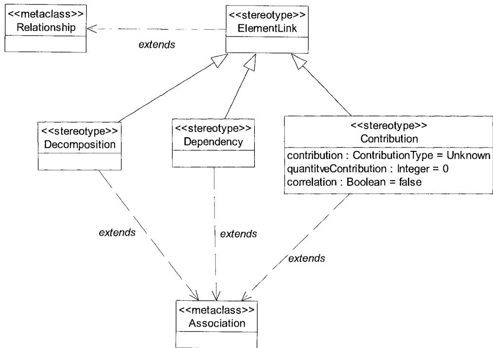
Figure 45 Element Link
