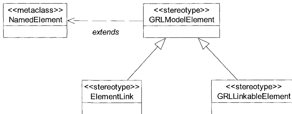
Figure 44 GRL Model Element
