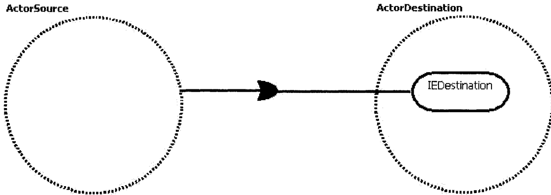
Figure 39 Dependency Scenario 2
