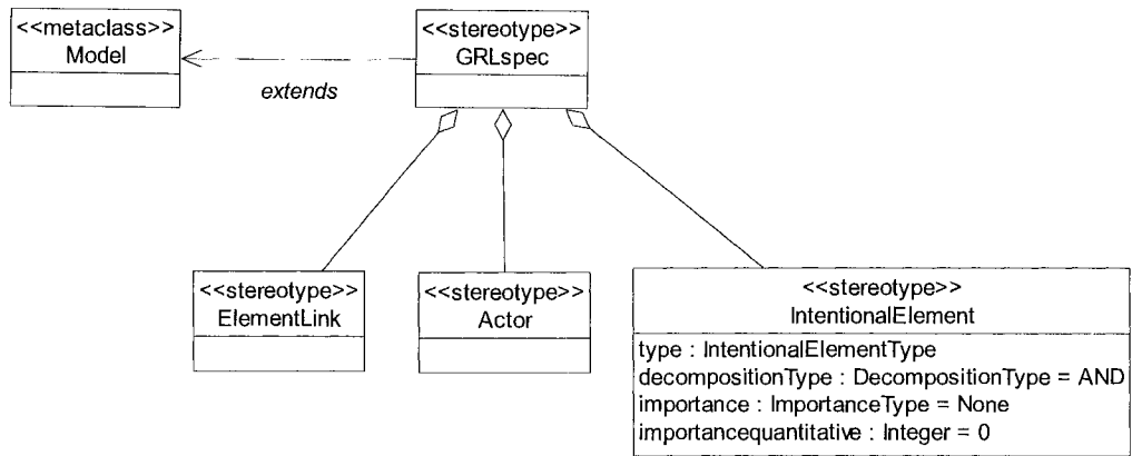
Figure 47 GRL Spec
