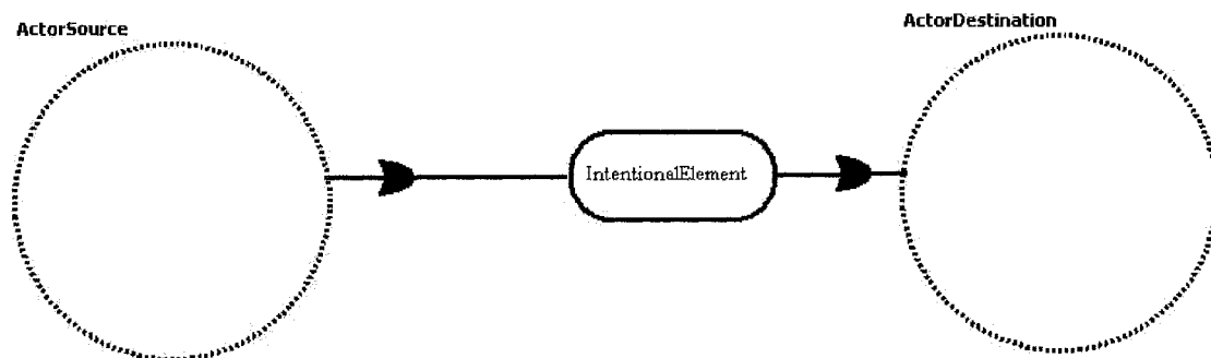
Figure 38 Dependency Scenario 1
