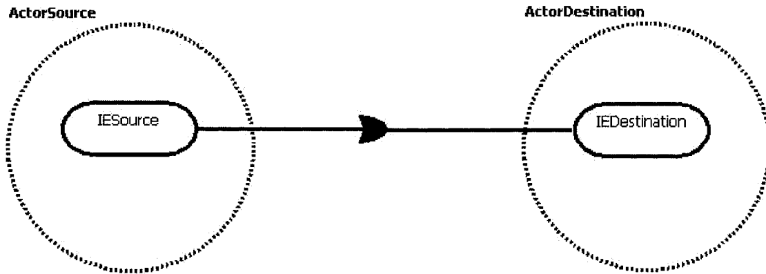
Figure 41 Dependency Scenario 4
