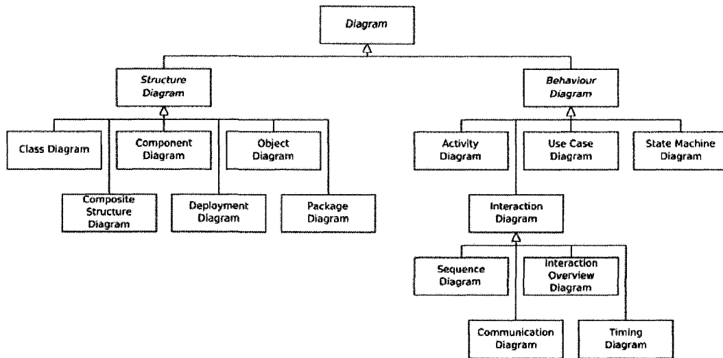
Figure 1 UML Diagrams Presentation in Class Diagram (UML IS)
