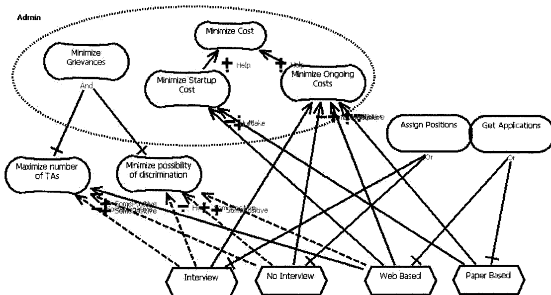
Figure 67 Admin, Modelled with jUCMNav
