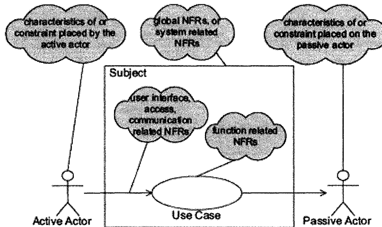
Figure 21 NFR Association Points in UseCase Model for NFR Types [25]
