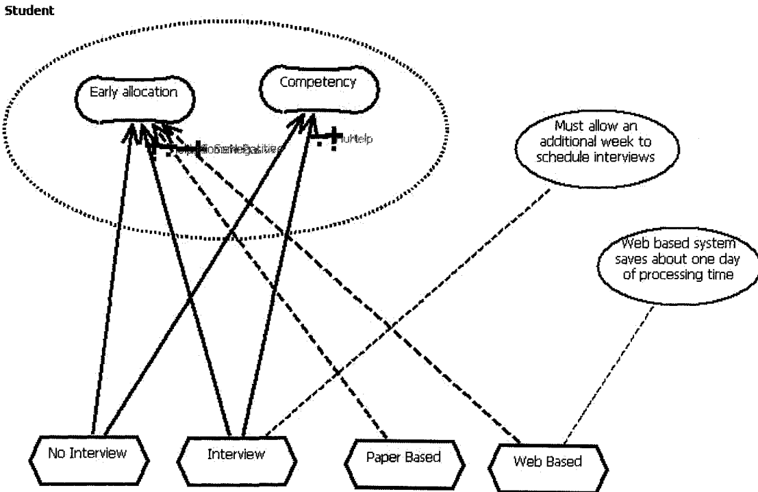
Figure 68 Student as Designed in jUCMNav
