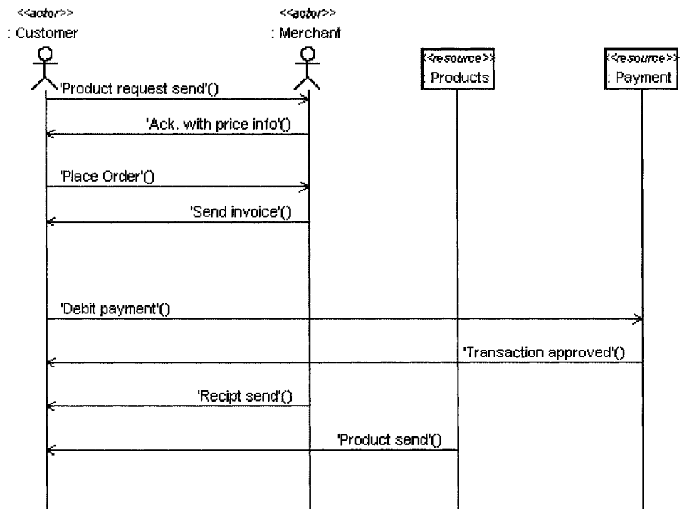
Figure 80 Customer Merchant Dependency (Sequence Diagram)
