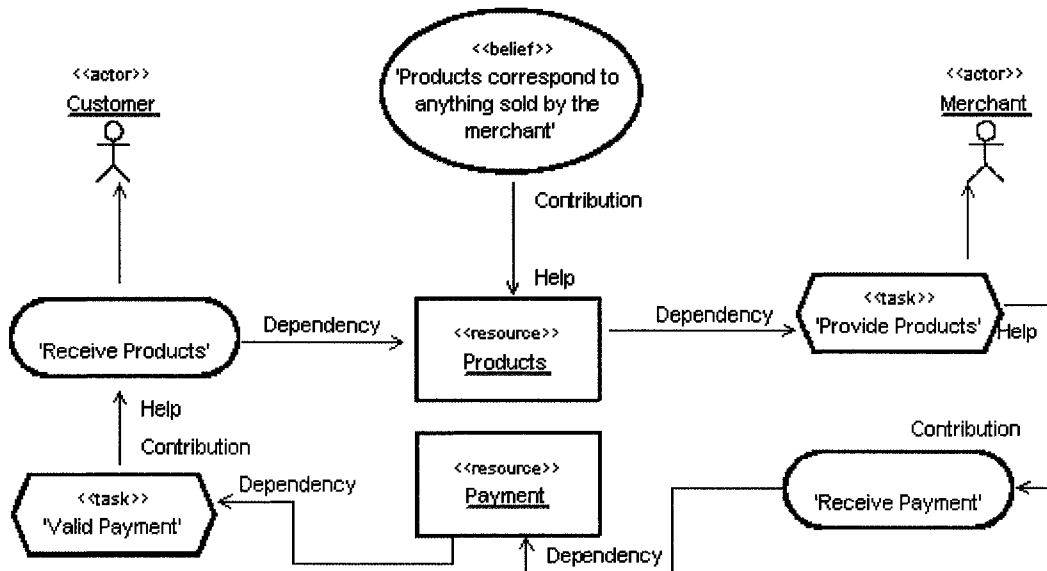
Figure 76 GRL Diagram to Show Links
