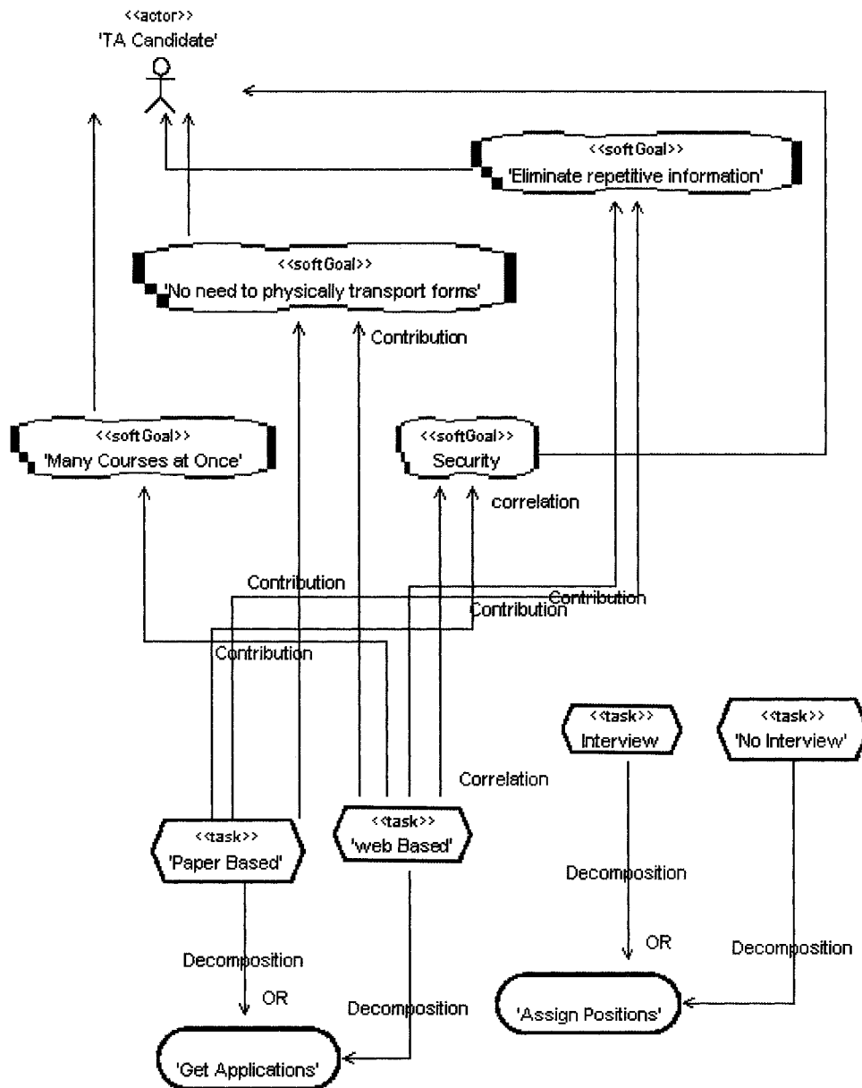
Figure 71 TA Candidate, Modelled with Tau GRL Profile
