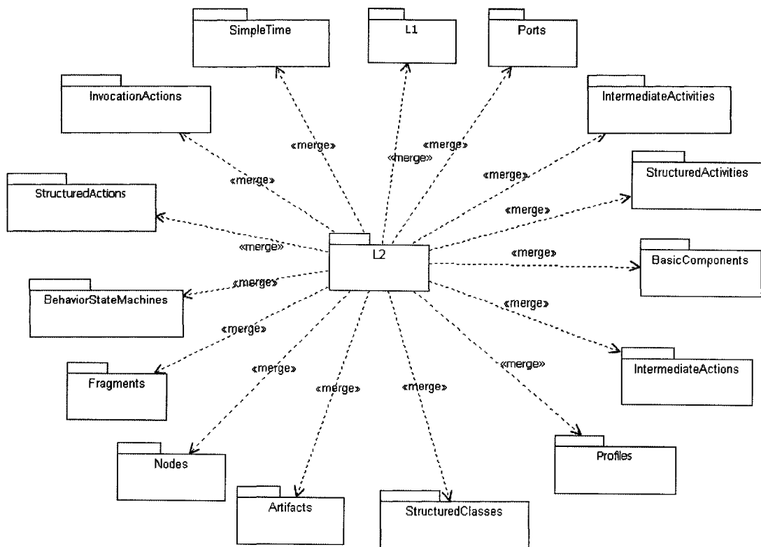
Figure 6 Level 2 (UML Superstructure)
