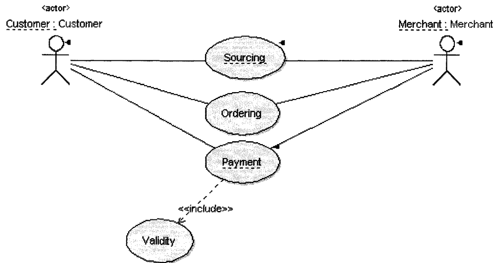
Figure 77 Use Case Diagram to Show Links
