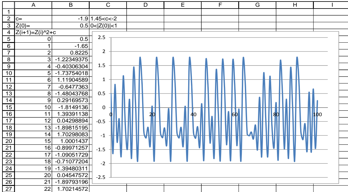
Figure 8 Equation from the Scientific American Fractal T-Shirt
