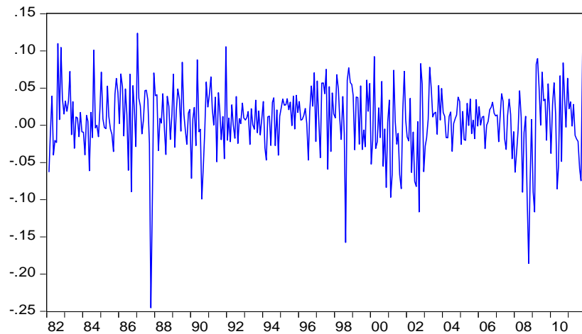
Figure 1 Monthly SP&500 returns – January 1982 to February 2012 S&P500 returns
