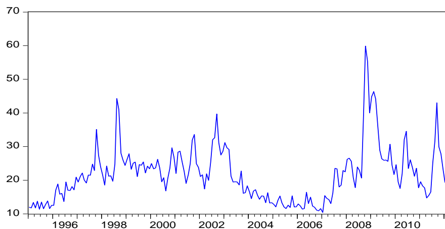
Figure 2 Monthly S&P500 Volatility Index (VIX) – January 1995 to March 2012 VIX
