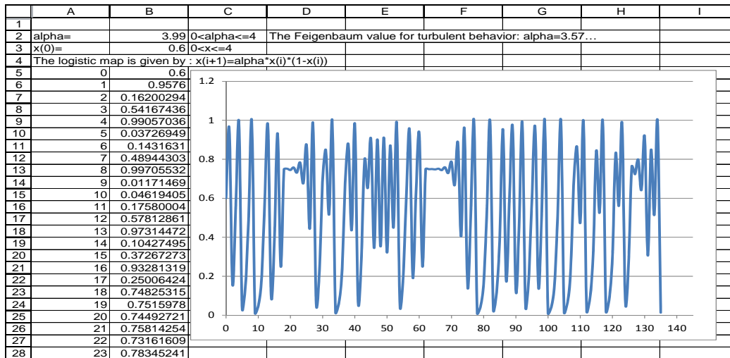
The logistic map
