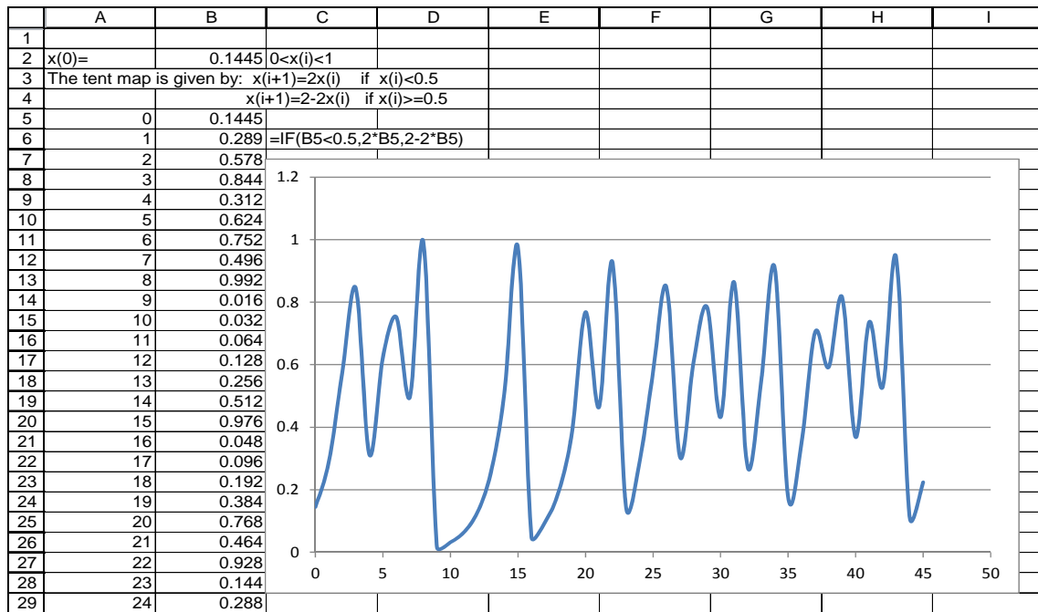
The tent map
