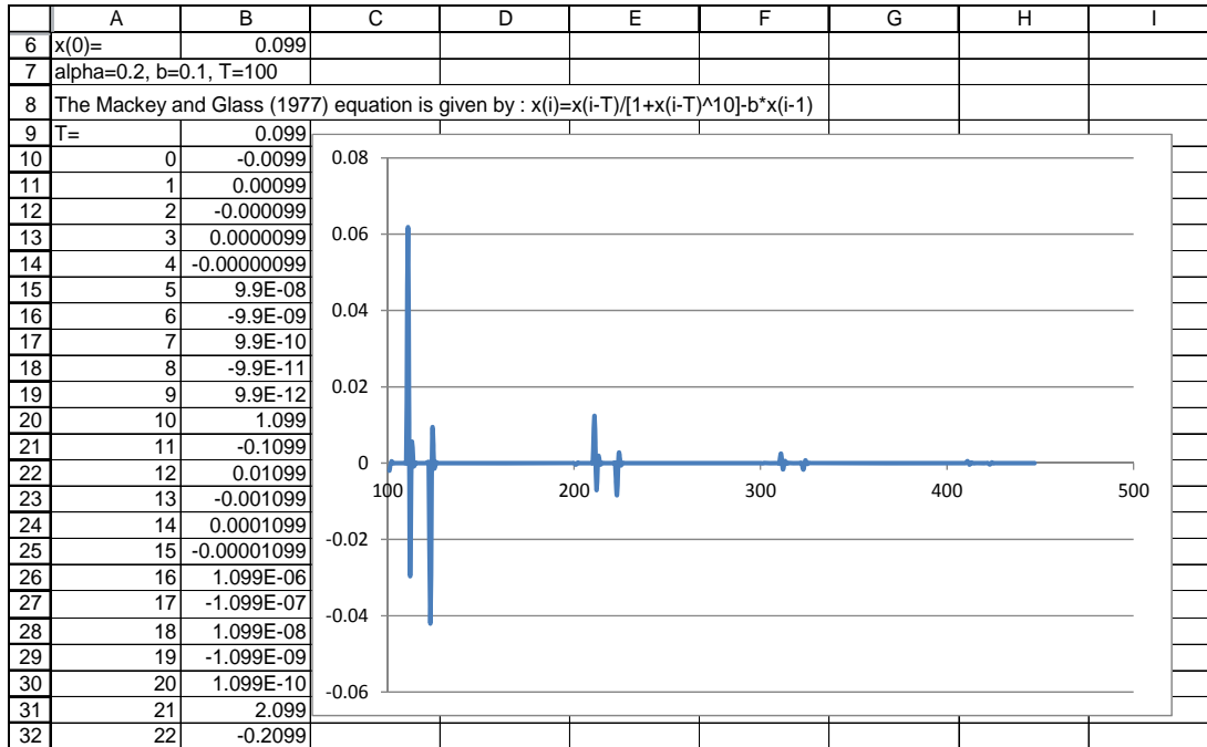
The Mackey and Glass (1977) equation
