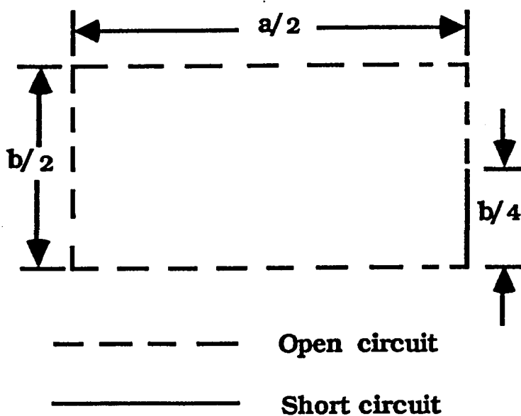
(a) A Simplified Geometry of a Finned Waveguide
