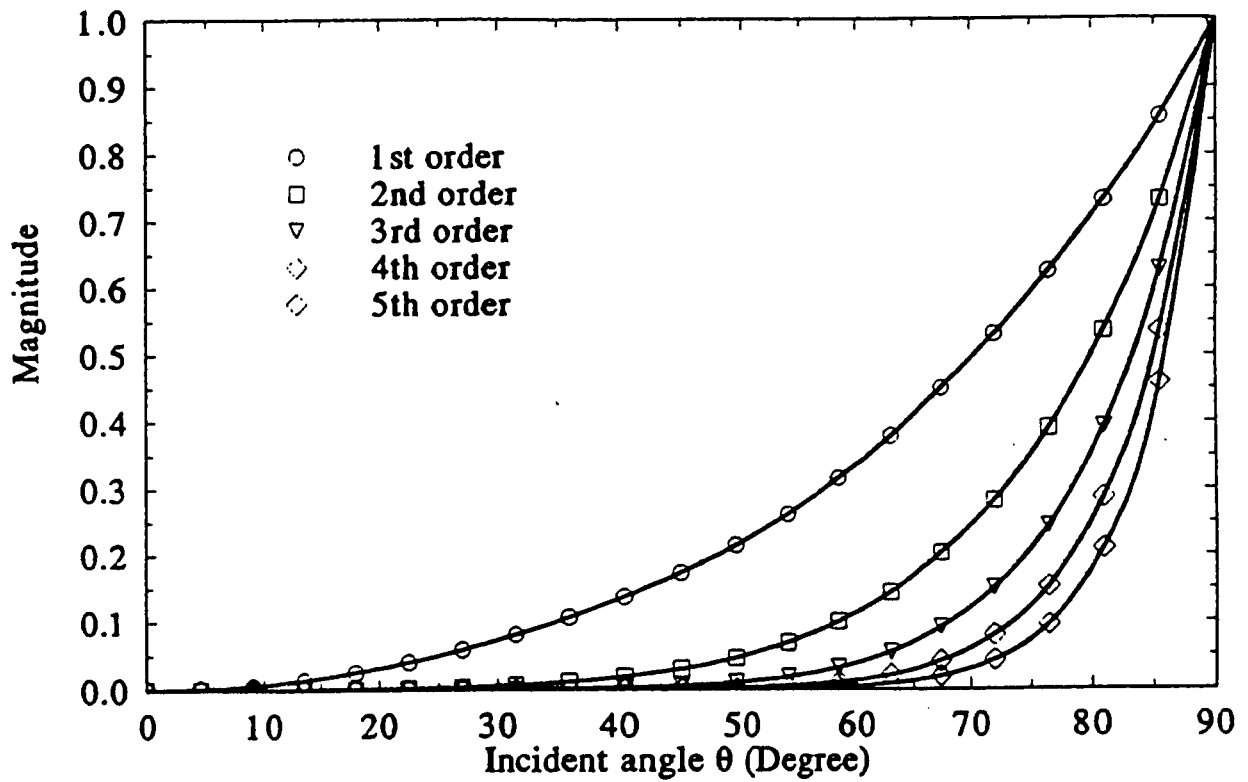
Reflection Coefficients of Higdon's Conditions (For either physical modes or spurious modes) ( \theta_i = 0^\circ, i = 1, 2, \dots, P, \Delta l/\lambda = 0.025 )
