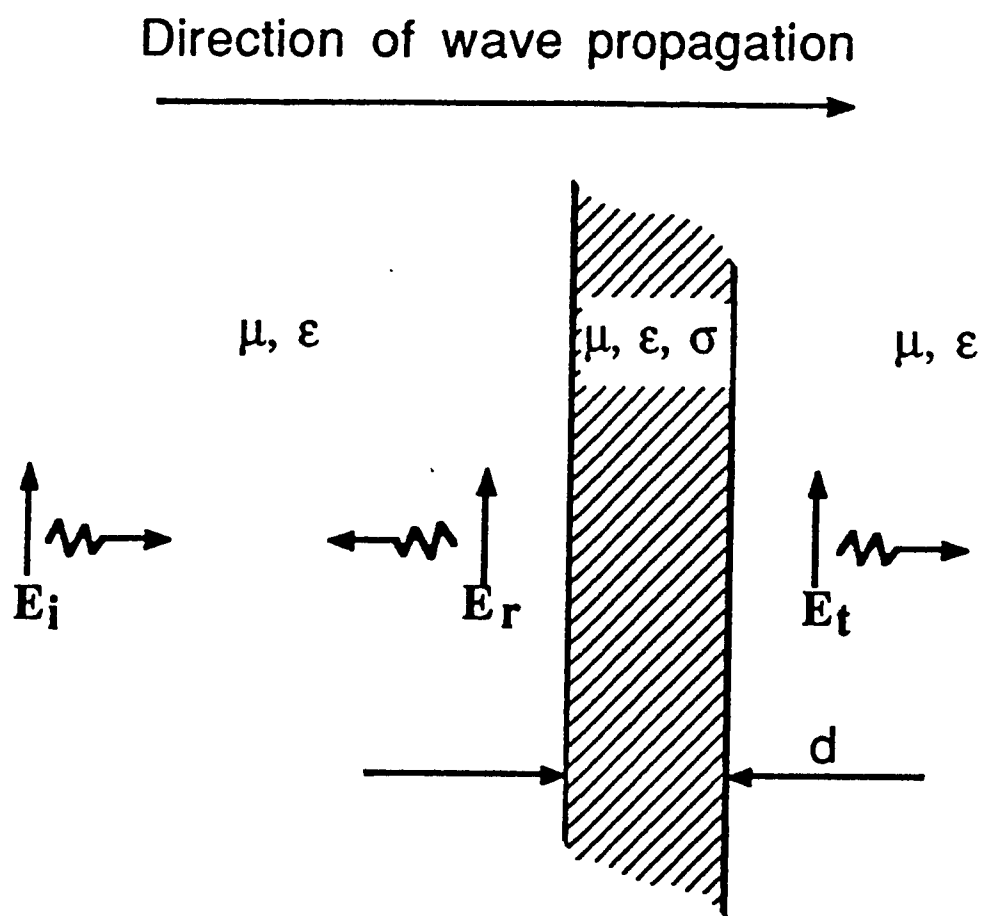
Figure 5.7: An Infinite Conducting Sheet with Thickness d and Conductivity \sigma Irradiated by a Plane Wave
