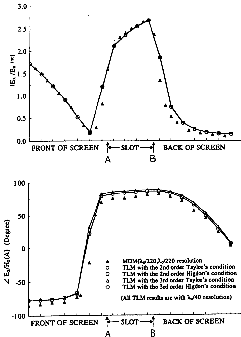
Figure 4.20: Comparison of the TLM and Frequency-domain Surface EFIE Results for the Gap Electric Field Distribution in the Slotted Screen
