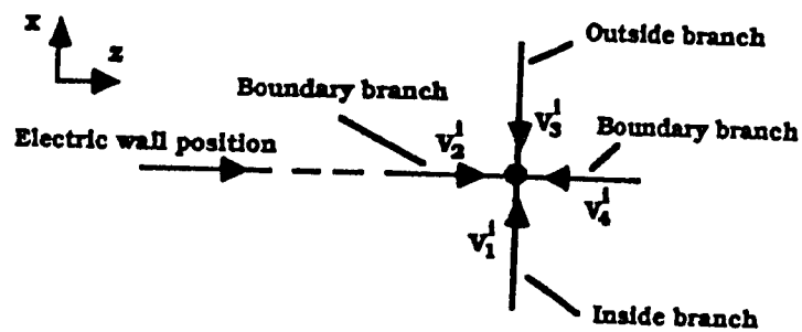
(c) The Electric Wall Placed Across a Node
