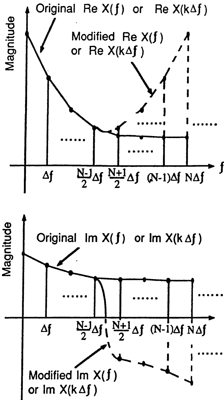
Figure 5.1: The Original and Modified X(f) or X(k\Delta f) when N is odd
