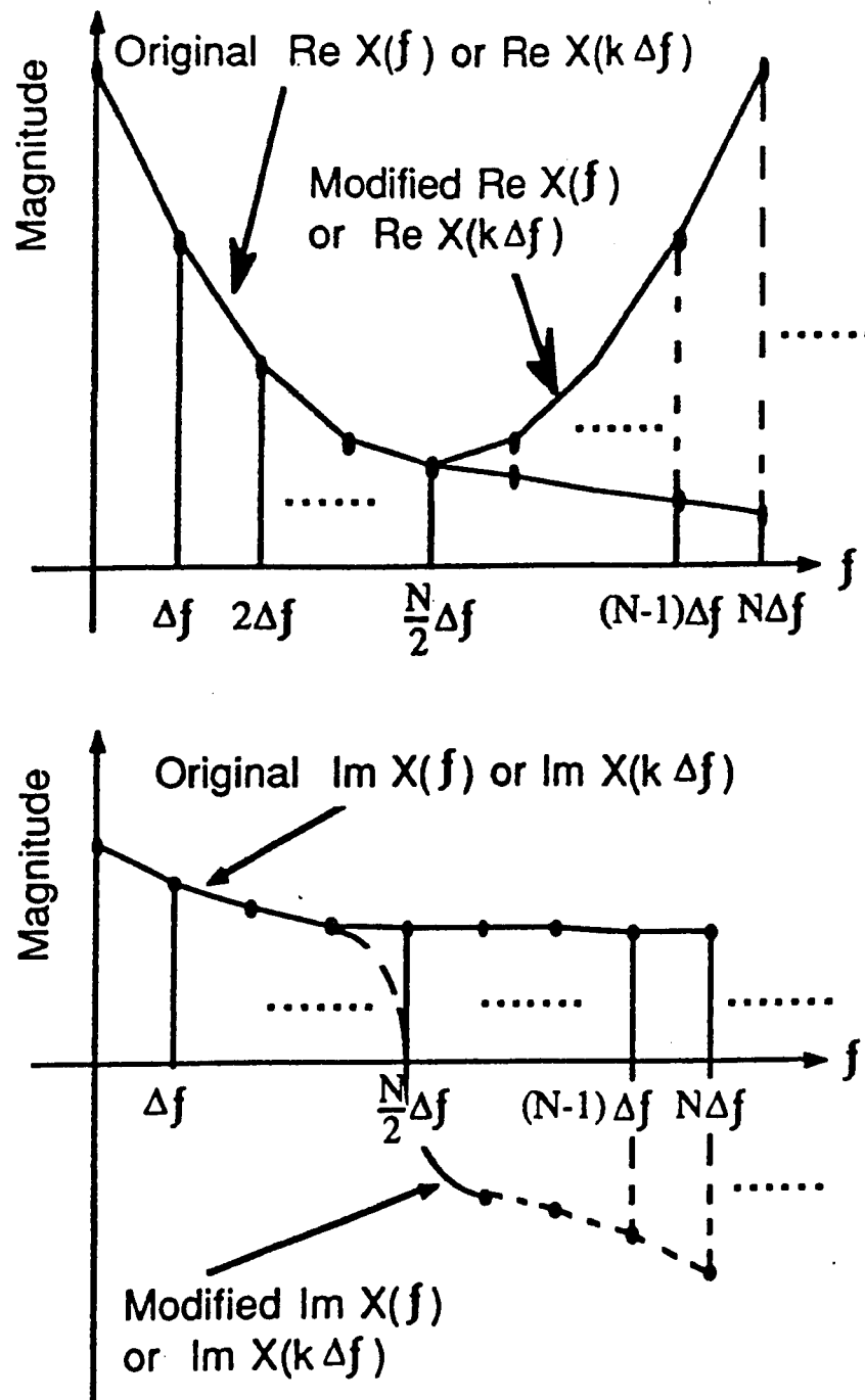
Figure 5.2: The Original and Modified X(f) or X(k\Delta f) when N is even
