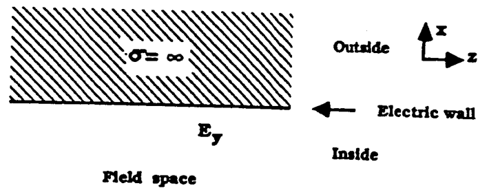
(a) An Electric Wall
