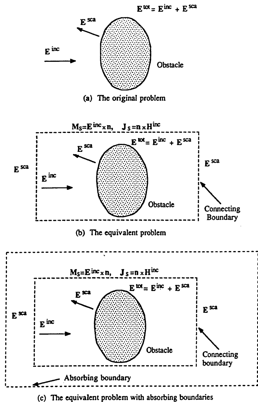
Figure 4.14: An Obstacle Illuminated by an Electromagnetic Wave
