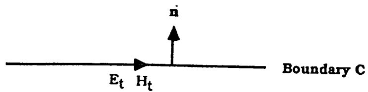
(a) A Perfect Reflecting Wall
