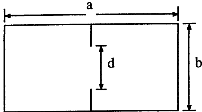
(a) Cross-section of a finned rectangular waveguide
