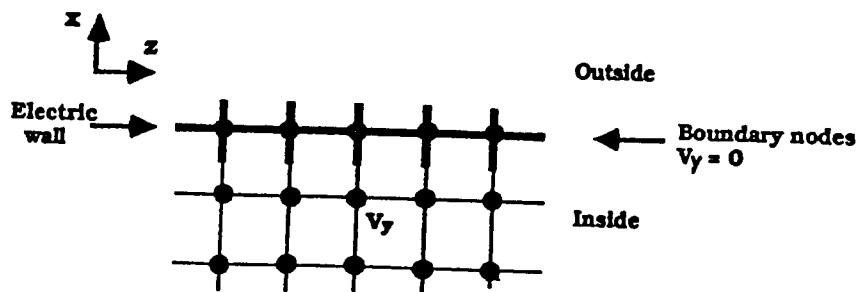
(b) The TLM Simulation With Electric Wall Placed Across the Nodes
