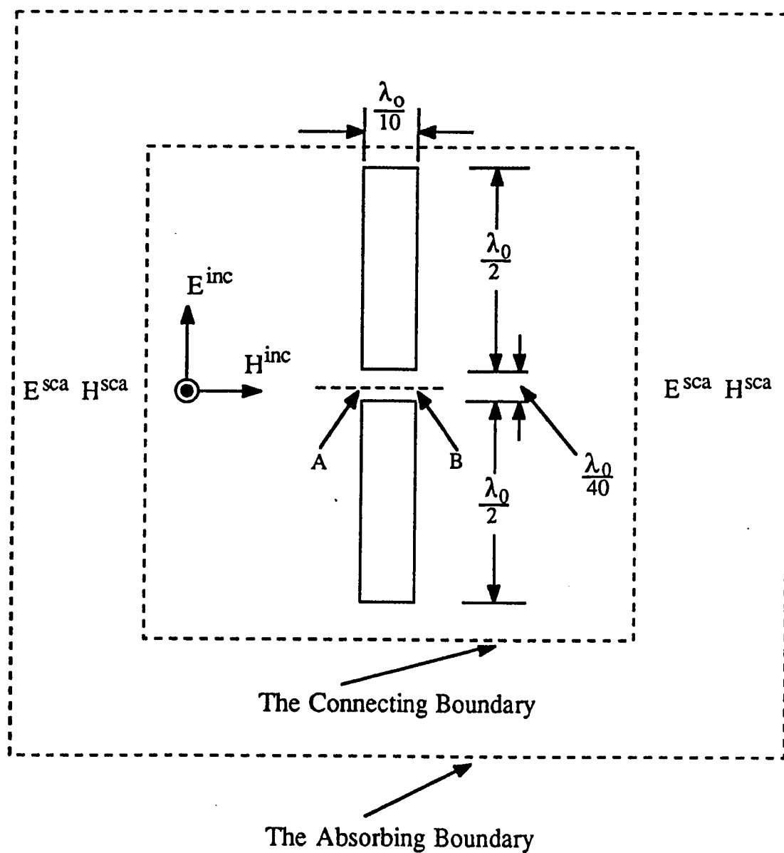
Figure 4.19: A Straight Slotted Conducting Screen
