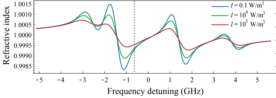
FIGURE 1.5: Refractive index of natural Rb at D_2 line in the non-linear regime calculated from Eq. (1.30). Our nonlinear experiment presented in Chapter 3 was performed at the frequency detuning shown by the dashed line. At this wavelength, the refractive index is larger at higher laser intensities, resulting in self-focusing of the laser beam.
