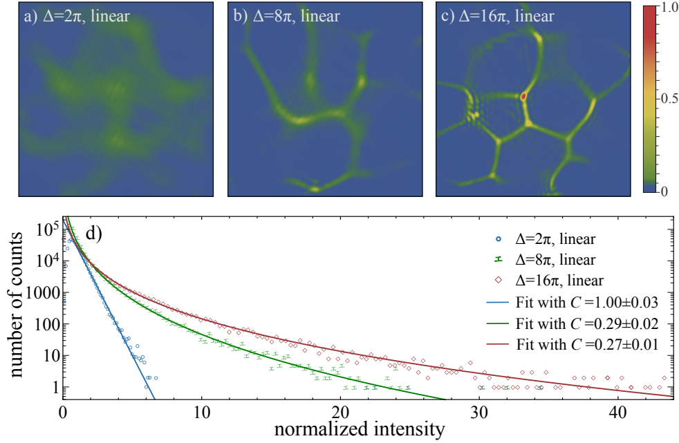
FIGURE 3.2: Generation of caustics upon linear propagation. a, b, c) Examples of patterns formed after propagation in free space from different phase masks with amplitudes \Delta = 2\pi , 8\pi and 16\pi , respectively. We see that sharp caustics are formed only under strong phase modulation. d) Intensity distributions for the patterns generated upon propagation through free space from three different phase amplitudes \Delta . The C -parameter from the fit function characterizes the heavy-tailed behaviour; the lower the C -parameter, the longer the tail of the distribution. Thus, sharp caustics are distinguished by their heavy-tailed statistics.
