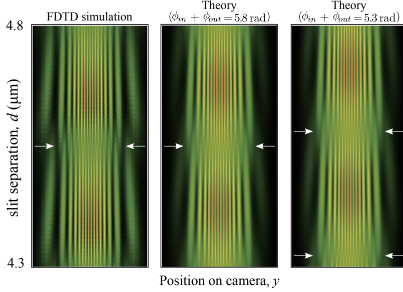
FIGURE 5.4: Far-field interference pattern for different slit separations from 4.3\text{ }\mu\text{m} to 4.8\text{ }\mu\text{m} obtained from FDTD simulation and from our theoretical model. For the theoretical plots Eq. (5.2) is multiplied by a sinc function to account for the finite width of the slits. The theoretical result matches to the numerical simulation when we incorporate a coupling phase of \phi_{in} + \phi_{out} = 5.8 radians. With other values of the coupling phase the position of the minimum visibility (indicated by the arrows) shifts, as shown in the rightmost plot. The excellent agreement between the simulation and the theoretical results confirms the validity of our theoretical model. The outer fringes in the theoretical plots are faint due to the deviation from the small angle approximation used for the sinc function.
