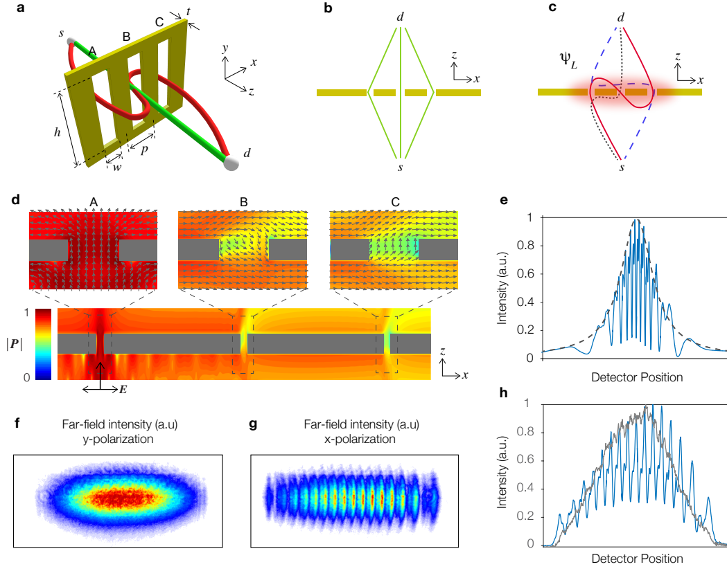
FIGURE 4.1: Trajectories of light in a three-slit interferometer. a) The three-slit structure considered in this study. The red path going from point s to point d illustrates a possible looped trajectory of light. b) Direct trajectories of light resulting from considering only the first term in Eq. (4.8). c) Examples of exotic looped trajectories arising from the higher order terms in Eq. (4.8). The red cloud in the vicinity of the slits depicts the near-field distribution, which increases the probability of photons to follow looped trajectories. d) Normalized Poynting vector \mathbf{P} in the vicinity of the three slits obtained through full wave simulations at a wavelength \lambda = 810 nm, using a slit width w equals to 200 nm, slit separation p = 4.6 \mu\text{m} , sample thickness t = 110 nm, and assuming infinite height, h = \infty . The simulations consider a Gaussian beam excitation polarized along x , and focused onto slit A. The Poynting vector clearly exhibits a looped trajectory such as the solid path in (c). e) Far-field interference patterns calculated under x -polarized (solid) and y -polarized (dashed) optical excitation. Interference fringes are formed in the far field only when strong near fields are excited ( x -polarization). f) Experimental evidence that shows the far-field pattern for a situation in which only one slit is illuminated with y -polarized heralded single-photons. g) The presence of exotic looped trajectories leads to an increase in the visibility of the far-field pattern. This effect is observed when x -polarized light illuminates one of the slits. h, The transverse profile of the patterns shown in (f) and (g).
