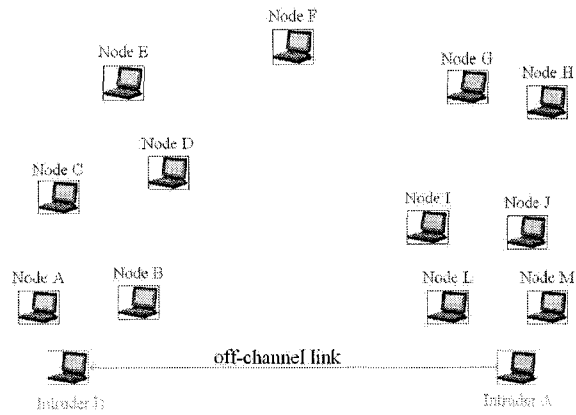
Figure 2.2: When a wormhole is treated as a misbehaving link, attackers are not detected and can create wormhole attacks targeting other nodes on the network. Detection only occurs after performance metrics are triggered, meaning there is latency in attack identification.
