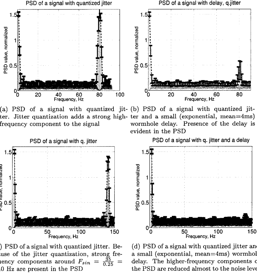
Figure 5.10: PSDs of signals with embedded quantized jitter
