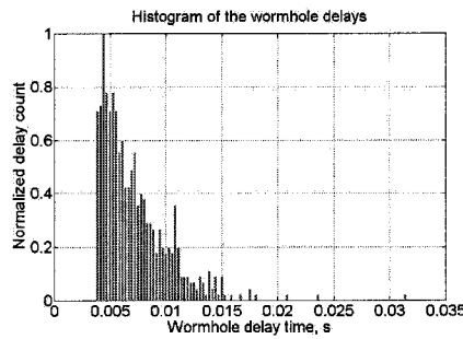
Figure 5.15: Normalized histogram of the wormhole delays obtained in an NS-2 experiment (without traffic)
