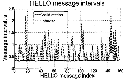
Figure 4.1: HMTIs obtained from the experimental work with the wormhole attack, where solid line shows an HMTI profile of a valid station, and a dashed line gives the HMTIs of an intruder. It can be observed that the HMTI values for the intruder are often higher than the HMTI values of a valid node.
