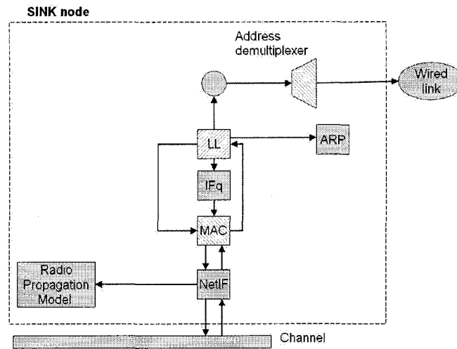
Figure 3.6: A wormhole sink node. A sink node is a simplified version of a general NS-2 wireless node. Striped parts are those that were changed to create a sink: the medium access component, the link layer, and the address demultiplexer. On the MAC layer, the SINK is programmed to accept and reject particular packets. On the LL layer, the changes are introduced to make sure all packets, even those that are supposed to be handled by the ARP layer, go up the protocol stack. The address demultiplexer is programmed to forward everything it receives up to the single wired link, regardless of IP addresses.
