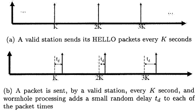
Figure 5.1: Signals that are formed by periodic HELLO messages for the valid node and for a wormhole attacker. Figure 5.1(a) shows a signal U(t) that is formed when a valid station sends its HELLO messages every K seconds. Figure 5.1(b) shows a signal V(t) that is formed when a random delay t_d is added to each regularly transmitted packet. Since each t_d is random, delays added to different packets also differ (but their ensemble obeys a certain statistical distribution).
