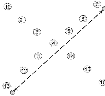
Figure A.1: A 'star' network layout with a wormhole connecting opposite ends of rays. A network, created with NS-2, has the 'star' shape with 4 rays. A wormhole 'connects' nodes 13 and 7.
