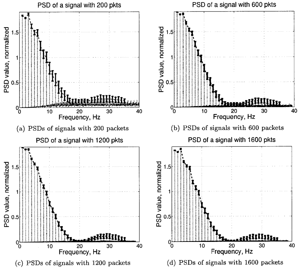
Figure 5.6: PSDs of signals obtained by keeping the experimental parameters the same and varying the number of packets used to obtain a PSD. In the figures above, the error bars show the range of measurements obtained by running 30 independent experiments with the same settings. Note that the error bars become smaller (which implies that the PSDs converge) as the number of packets increases.
