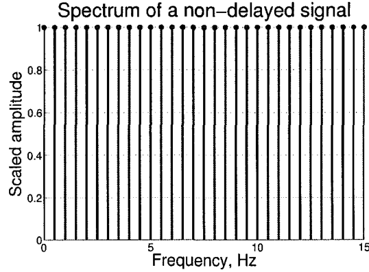
Figure 5.3: PSD of a perfectly regular signal U(t) with K = 2 . The \delta functions are located at integer multiples of \frac{1}{K} , and the envelope of the PSD is constant.
