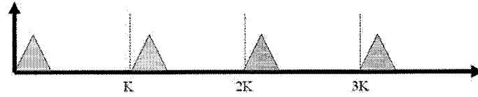
(b) As a result of convolving two square signals, a triangular signal is obtained on one period, with the same periodicity as the original signal.
