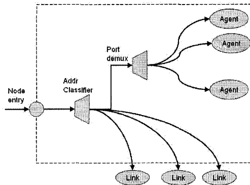
Figure 3.3: An NS-2 wired node. Packets, received by a node, are handled by the node's entry point — the address classifier. The address classifier determines whether a packet is destined to the node itself (in which case it is routed to the port demultiplexer), or to other nodes (it is then sent on to the corresponding wired link). The port demultiplexer, in turn, determines which agent should be receiving this packet. When node's agents themselves generate a packet, the packet, too, is sent to the node's entry point, where it is routed accordingly.
