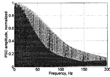
(d) The PSDs obtained in the experiment with 3 traffic flows of 0.1 MB each and 2 traffic flows of 0.01Mb each
