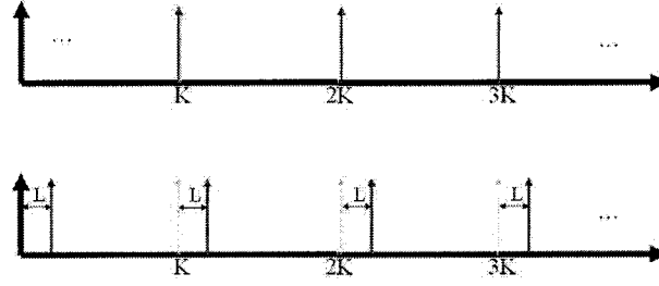
Figure 5.2: Autocorrelation of valid station's packet timings. Bottom shows time-shifted signal that is multiplied with the non-time-shifted version. It is obvious that the autocorrelation function will be periodic with period K , and non-zero only when the lag L is a multiple of K .
