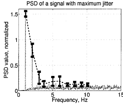
Figure 5.9: PSD of a signal with uniform jitter where maximum jitter value is \frac{K}{4} and P = 200 packets are used to determine a PSD. The PSD of such signal does not have high-frequency components, and varies a lot in individual experiments (shown by long error bars) due to a small number of packets used to characterize a PSD. These two factors together – a small number of packets and the lack of high-frequency components – make wormhole attack detection in this setting difficult.
