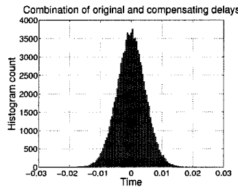
(c) The histogram of the delay that is achieved by combining a wormhole delay and a compensating delay presented above. The total delay is approximately Gaussian, with mean 0, and variance \sim 0.0212 * 10^{-3} .
