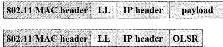
Figure 3.2: A schematic view of 802.11 packets' headers, a non-OLSR packet (top) and an OLSR packet (bottom). Within the NTA-MANET suite, parsing of 802.11 headers and parsing of OLSR data were implemented.
