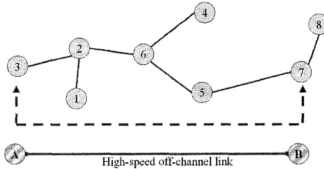
Figure 2.1: A network under a wormhole attack. Intruders A and B are connected by an off-channel link (e.g. a wired or satellite link), which they use to tunnel network data from one part of the network to the other. Without a wormhole, nodes 7 and 3 are 4 hops apart — their messages to each other should go through nodes 2, 6, and 5. When intruders A and B activate a wormhole, nodes 7 and 3 are able to directly overhear one another’s messages, and are lead to believe they are immediate neighbours. Once this happens, all further communications between nodes 3 and 7 will go through the wormhole link introduced by A and B.
