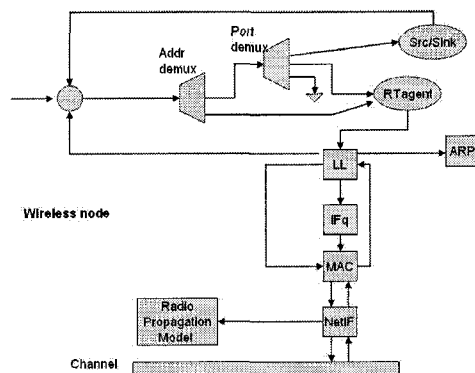
Figure 3.4: An NS-2 wireless node. In the NS-2 wired domain, the connectivity is determined by wired links. In wireless NS-2 world, there is a concept of a shared wireless channel, which the nodes use to communicate. When a packet is delivered to a node on the channel, it is handled by the MAC and LL layers, and is then sent up to the node entry point — the IP address demultiplexer. If a packet is destined to the node itself, it is sent to the port demultiplexer. Otherwise, it is handed down to the routing agent, which determines where to send it next. All packets that are placed on the wireless channel go through routing agent, link layer, and MAC components.
