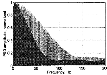
(e) The PSDs obtained in the experiment with 5 traffic flows of 0.1 MB each
