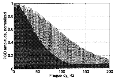
(c) The PSDs obtained in the experiment with 5 traffic flows of 0.01Mb each
