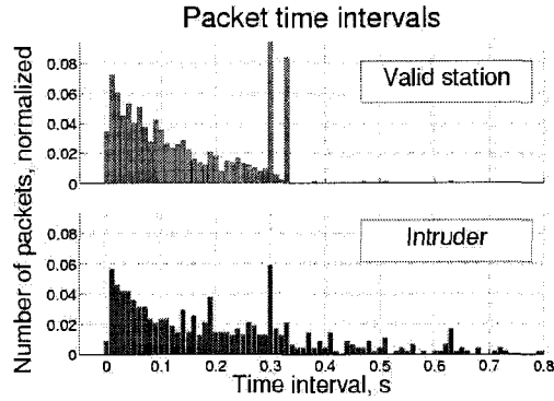
Figure 4.2: Normalized histogram of the packet intervals. A valid node is shown on top, while the intruder is presented on the bottom. It can be observed that for a valid node the packet interval is upper-bounded by the HELLO message interval, as it should be. For the intruder, that is not the case: a great deal of packet intervals are much higher than the HELLO message interval.
