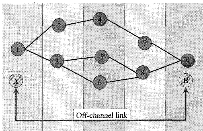
Figure 2.4: A testbed wormhole attack: experimental setup. Altogether, there were 9 valid nodes on the network and 2 intruders (A and B) connecting distant network parts. One of the intruders was programmed to randomly drop a portion of the traffic it was retransmitting.
