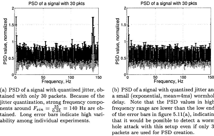
Figure 5.11: PSDs of signals with quantized jitter that are obtained using only 30 packets. From these figures, it is clear that a wormhole introduces a delay to a PSD that is apparent even if only 30 packets are used for PSD calculations.
