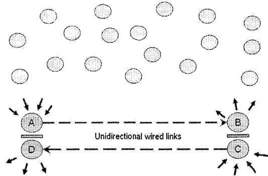
Figure 3.5: Schematics of the wormhole attack implementation in NS-2. Each end of a wormhole has two components: a sink that records all it hears (A and C on the diagram) and a source that replays everything it receives on the wired side (B and D) wirelessly. Sinks and sources are connected by unidirectional links. For example, sink A records everything it hears wirelessly and transfers it over a unidirectional wired link to source B. Source B, in turn, replays wirelessly all packets it receives from sink A. Along with a sink and a source, each end of the wormhole includes a firewall to prevent infinite loops arising from sinks replaying packets coming from sources.
