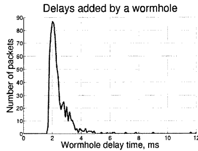
Figure 5.12: Profile of the experimental time delay resulting from packet traveling through a wormhole. The delay is measured by comparing the sniffer timestamps of packets broadcast by the legitimate node and the same packet after it is rebroadcast at the end of the wormhole.
