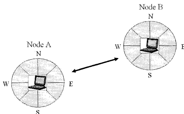
Figure 2.3: Nodes using directional antennas. When nodes A and B communicate, they send their messages on specific ‘sectors’: node A uses its North-East sector, node B - South-West. Therefore both nodes know how they are located with respect to each other. From knowing the sector on which it receives B’s messages, A knows that B is located to the North-East. Had nodes A and B used omni-directional antennas, A would not be able to say anything at all about B’s location.
