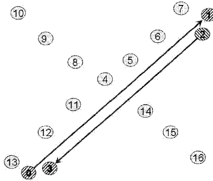
Figure A.4: A star topology from figure A.1 with wormhole attackers identified. In routing tables coming out of the star topology (figures A.1, A.3, A.2) attacking nodes are not present. They are, in essence, invisible. In the NS-2 trace, however, the attackers can be observed. In this star topology, the attackers 0 and 3(a sink and a source) are placed next to node 13, while the other sink and source (nodes 1 and 2) are placed next to node 7.
