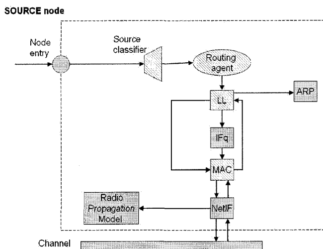
Figure 3.7: A wormhole source node. A source node takes everything it receives on the wire and sends it on the wired medium. To create a source node, the ‘wireless’ node is simplified, and the following components are altered: the address classifier (so that it forwards everything to the routing agent), the routing agent, and the lower wireless media-related stack layers. At the MAC layer, a source node should ignore everything it hears.
