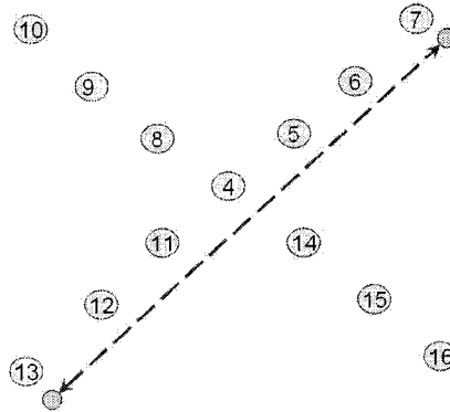
Figure 5.14: The NS-2 MANET used in this experiment has a ‘star’ shape, as shown here. The wormhole attackers ‘connect’ opposite star rays (nodes 13 and 7)
