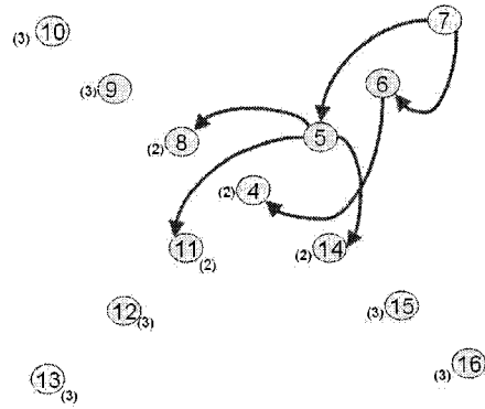
Figure A.2: Graphical representation of node 7 routing table (no wormhole present). The number of hops is shown in brackets; links in the two-hop region of node 7 are shown by arrows
