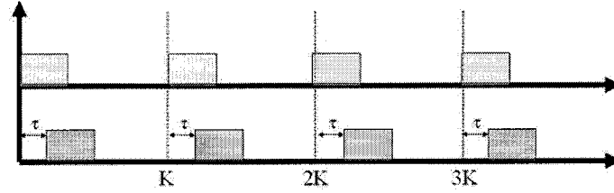
(a) To obtain an autocorrelation, a signal is multiplied with a time-shifted version of itself. The bottom signal ‘slides’ with respect to the top signal. In this case – the case of two uniform distributions – two squares are shifted and multiplied.
