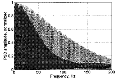
(a) The PSDs obtained in the 'baseline' experiment with no traffic load on the network (except for routing messages)
