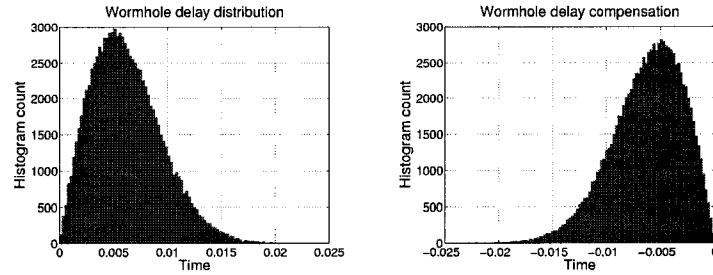
(a) A wormhole delay histogram. The delay this wormhole introduces is Rayleigh, with mean 0.005 seconds and variance \sim 0.0106 * 10^{-3} .
