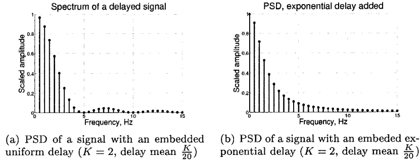
Figure 5.5: PSDs of signals with uniform and exponential delays
