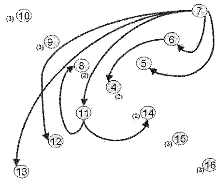
Figure A.3: Graphical representation of node 7 routing table with a wormhole ‘connecting’ nodes 7 and 13. Nodes as distant as 13, 12, and 11, node 7 considers to be direct neighbours. Note, that communication with nodes 14 and 8 also goes through the wormhole, as node 7 considers them to be 2 hops away (going through node 11).
