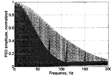
(b) The PSDs obtained in the experiment with 3 traffic flows of 0.01Mb each
