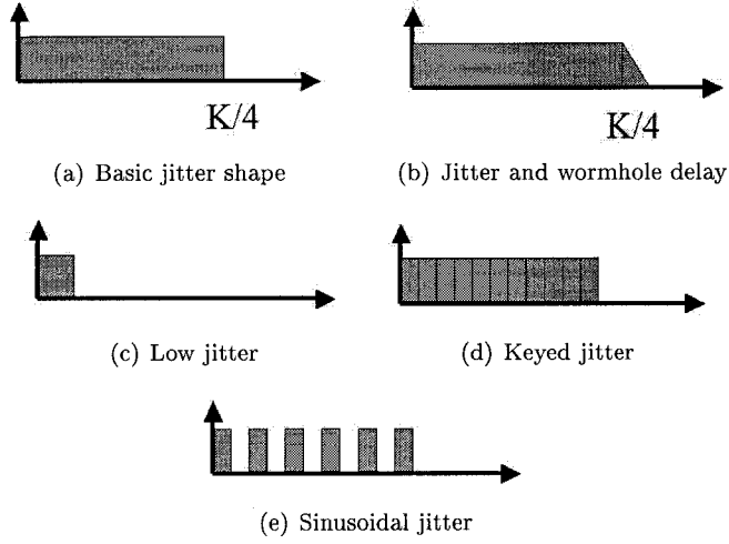
Figure 5.7: Figure 5.7(a) shows the basic jitter shape recommended by OLSR RFCs, where K is the HELLO message interval. Figure 5.7(b) shows that the addition of a wormhole delay on top of the jitter results in ‘smoothing’ of a distribution edge and in increasing the jitter range past \frac{K}{4} . The rest of the figures show the different jitter shapes proposed. Figure 5.7(c) demonstrates how the jitter’s maximum value can be decreased. Figure 5.7(d) demonstrates the idea of keyed pseudo-random jitter: each of the intervals, shown in this figure, corresponds to a particular value of keyed function. Finally, Figure 5.7(e) shows a ‘quantized’ jitter distribution: instead of occupying complete range of 0 to \frac{K}{4} , jitter values within this range are distributed such that a sinusoid can be fitted to them.
