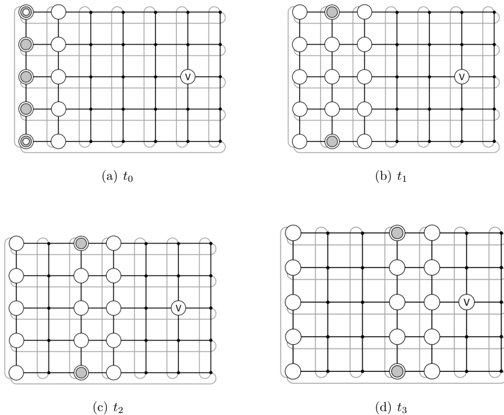
Figure 4.12: Arrangement of agents PBVD-T: part 1
