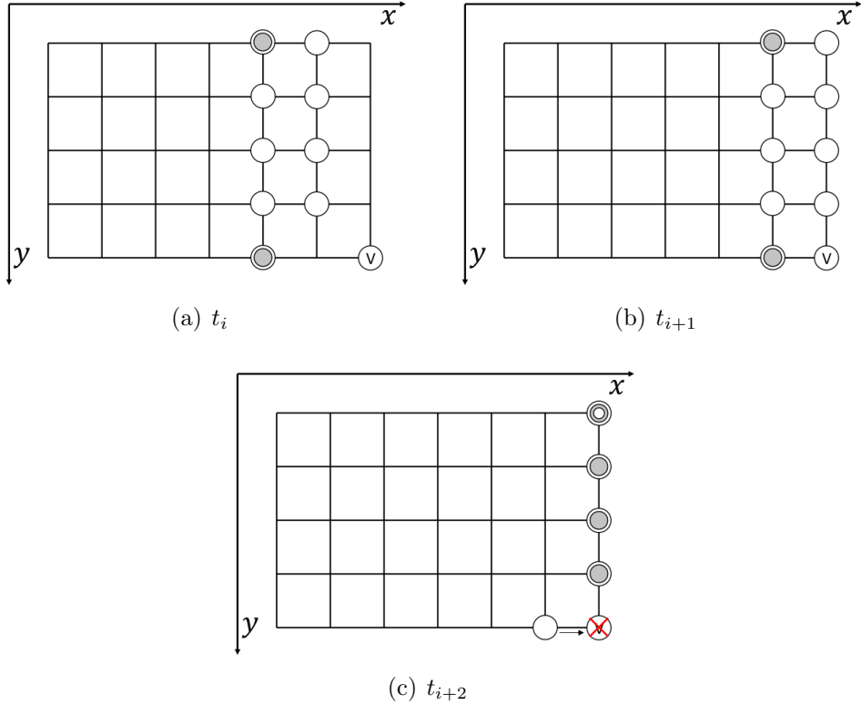
Figure 4.9: Arrangement of the agents in the elimination phase when the newly formed BV resides in a corner node (when x = d_1 - 1 and y = 0 or y = d_2 - 1 )
