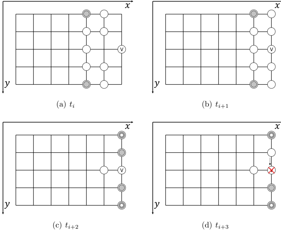
Figure 4.7: Arrangement of the agents in the elimination phase when the newly formed BV resides in a border node (when x = d_1 - 1 )
