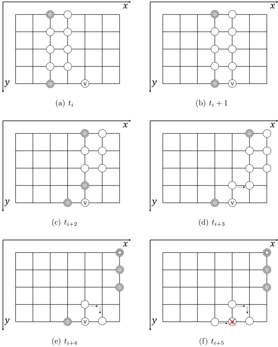
Figure 4.8: Arrangement of the agents in the elimination phase when the newly formed BV resides in a border node (when y = 0 or y = d_2 - 1 )
