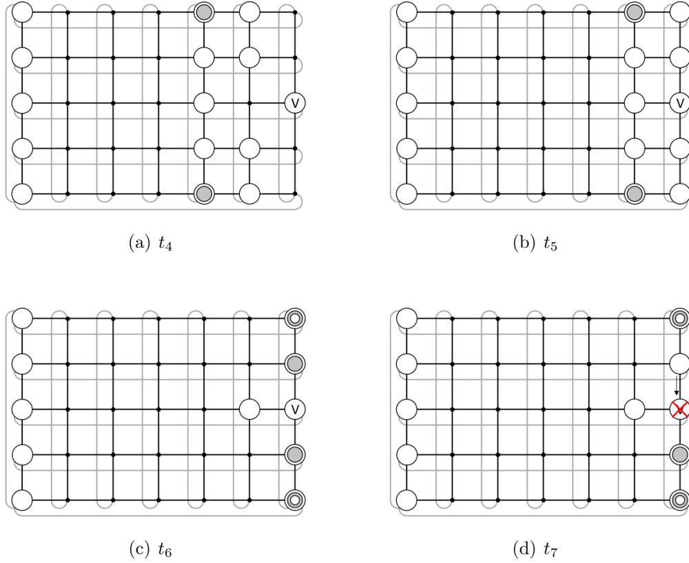
Figure 4.13: Arrangement of agents PBVD-T: part 2
