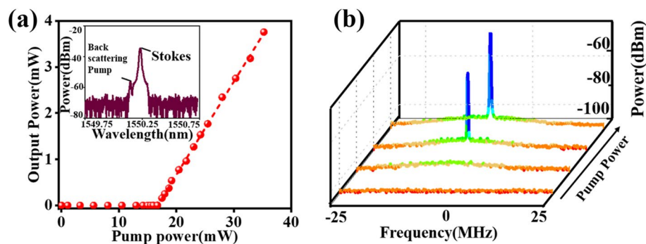
Fig. 2 BRFL emission characteristics. a Optical power with respect to the pumping power shows a typical laser threshold behavior ( P_{\text{th}} = 15.64 mW). b Beat signals for different pump power ratios ( P/P_{\text{th}} = 0.1, 0.8, 1.2, 2.0 ), its center frequency was normalized to the Brillouin frequency shift of 10.8-GHz in silica fibers
