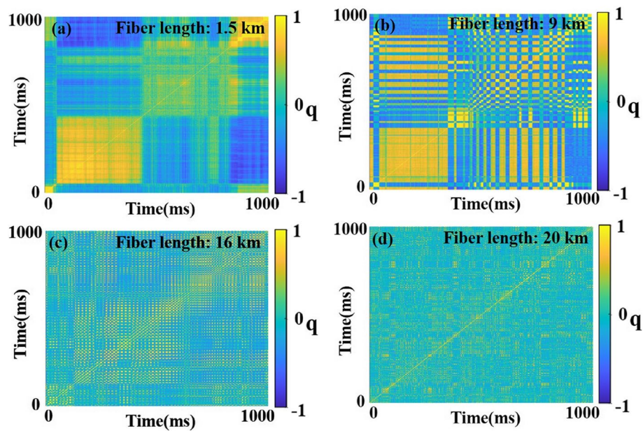
Fig. 9 The q distribution of BRFL spectrum with different modes density determined by different fiber lengths of a 1.5 km, b 9 km, c 16 km and d 20 km
