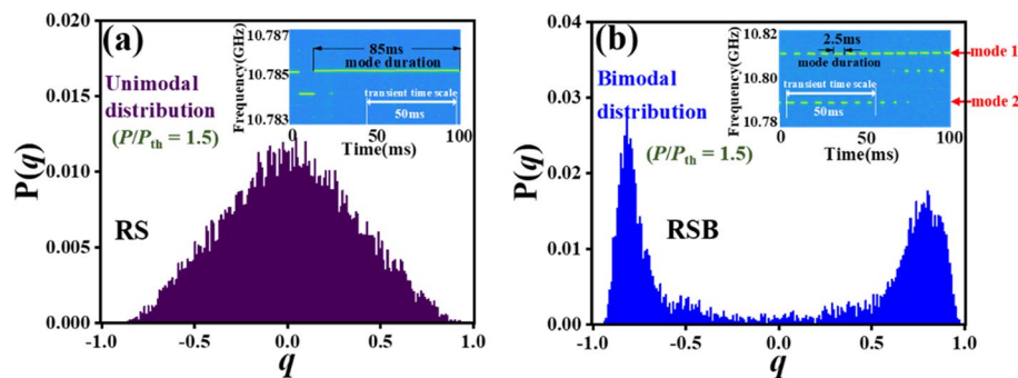
Fig. 7 Distribution of P(q) when P/P_{th} = 1.5 under the observation time of 50 ms. a Unimodal state b Bimodal state. The insets correspond the mode evolutions
