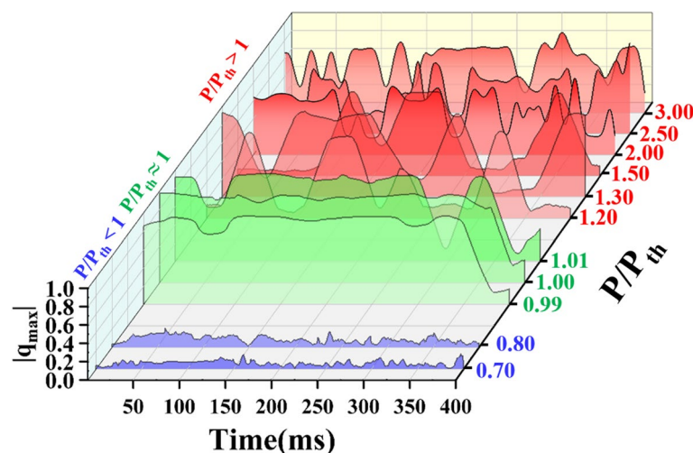
Fig. 6 Temporal evolution of |q_{max}| (400-ms observation time) under different pump power ratios. Three typical pump power regimes: (i) P/P_{th} < 1 (blue curves), (ii) P/P_{th} \approx 1 around threshold (green curves) and (iii) P/P_{th} > 1 (red curves)
