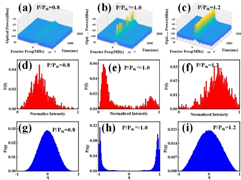
Fig. 3 BRFL for each excitation power in the regimes well below [ P/P_{th} = 0.8 ], around [ P/P_{th} \approx 1.0 ], and above [ P/P_{th} = 1.2 ]. a–c Spectra of 1000 consecutive shots for each excitation power. d–f Intensity distribution calculated from 1000 spectra. g–i Distribution P(q) of values of the Parisi overlap parameter q for the same values of the excitation power ratio P/P_{th}
