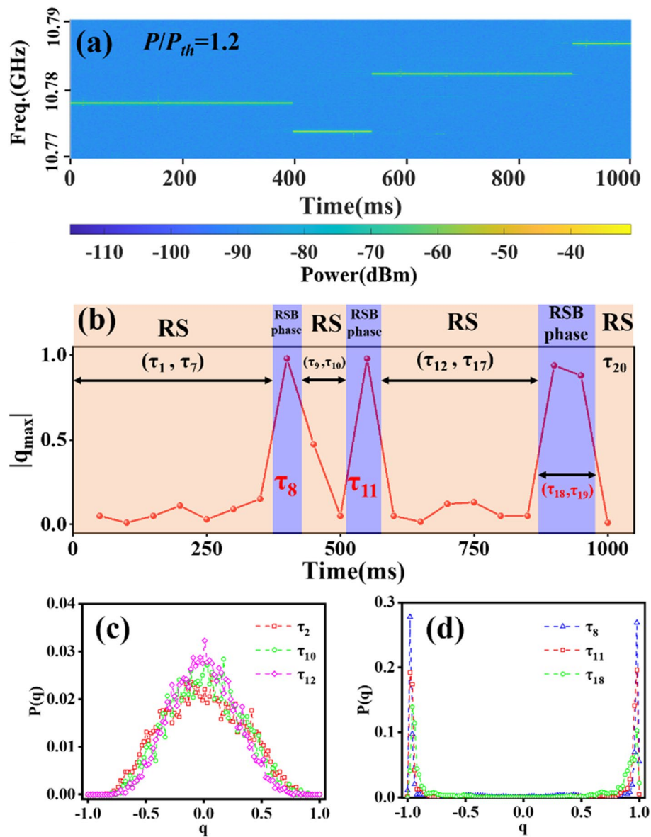
Fig. 4 Time-domain evolution of RSB in the BRFL under P/P_{th} = 1.2 . a The spectra of the beat signal within 1000 ms above the laser threshold. b |q_{\max}| in 20 subsequent time windows with a time interval of 50 ms. c P(q) within sub-time windows of \tau_2, \tau_{10} and \tau_{12} . d P(q) within sub-time windows of \tau_8, \tau_{11} and \tau_{18}
