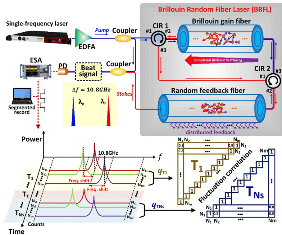
Fig. 1 Schematic for the transient RSB observation and statistical analysis in the BRFL. EDFA—Erbium doped fiber amplifier, CIR—optical fiber circulator, PD – photodetector, ESA—electrical signal analyzer
