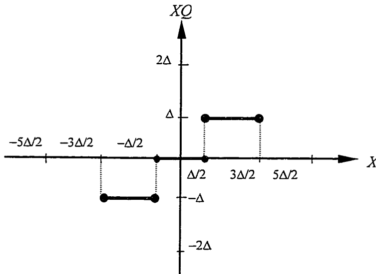
Figure 2.9 2-bit deadzone-type quantizer
