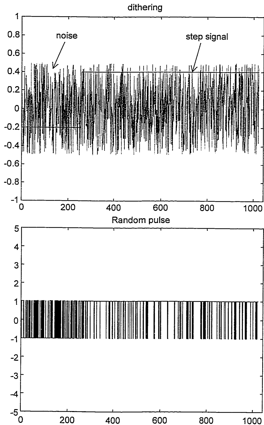
Figure 2.11 1-bit random pulse representation of a step signal
