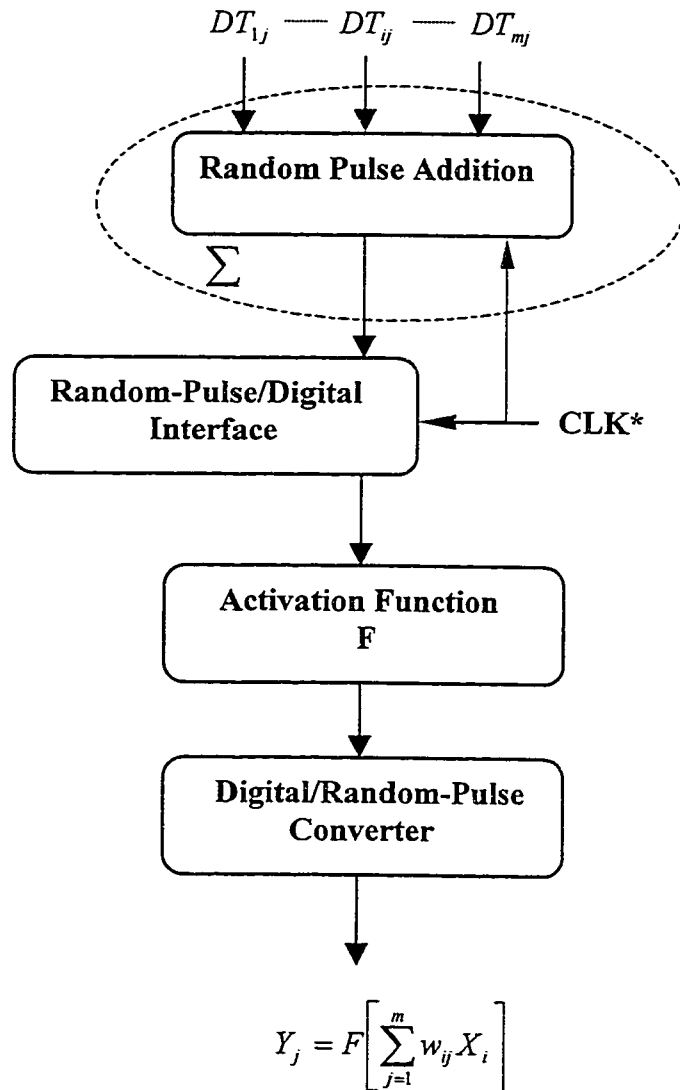
Figure 3.24 Random pulse implementation of the neuron body
