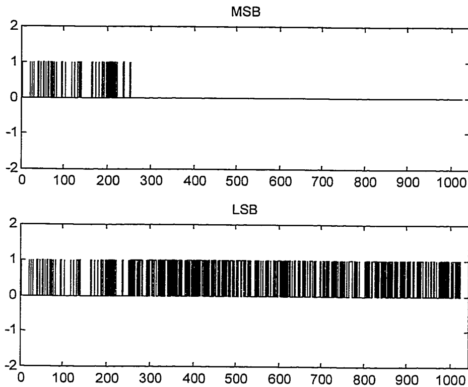
Figure 2.12 2-bit random-pulse representation of a step signal
