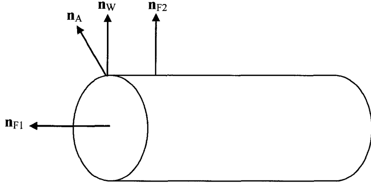
Figure 4.3: Illustration of the difference between the normal at a point on a curve obtained as the curvature-weighted average \mathbf{n}_W of the normals \mathbf{n}_{F1} and \mathbf{n}_{F2} to the adjacent faces and the unweighted average \mathbf{n}_A of the two normals.
