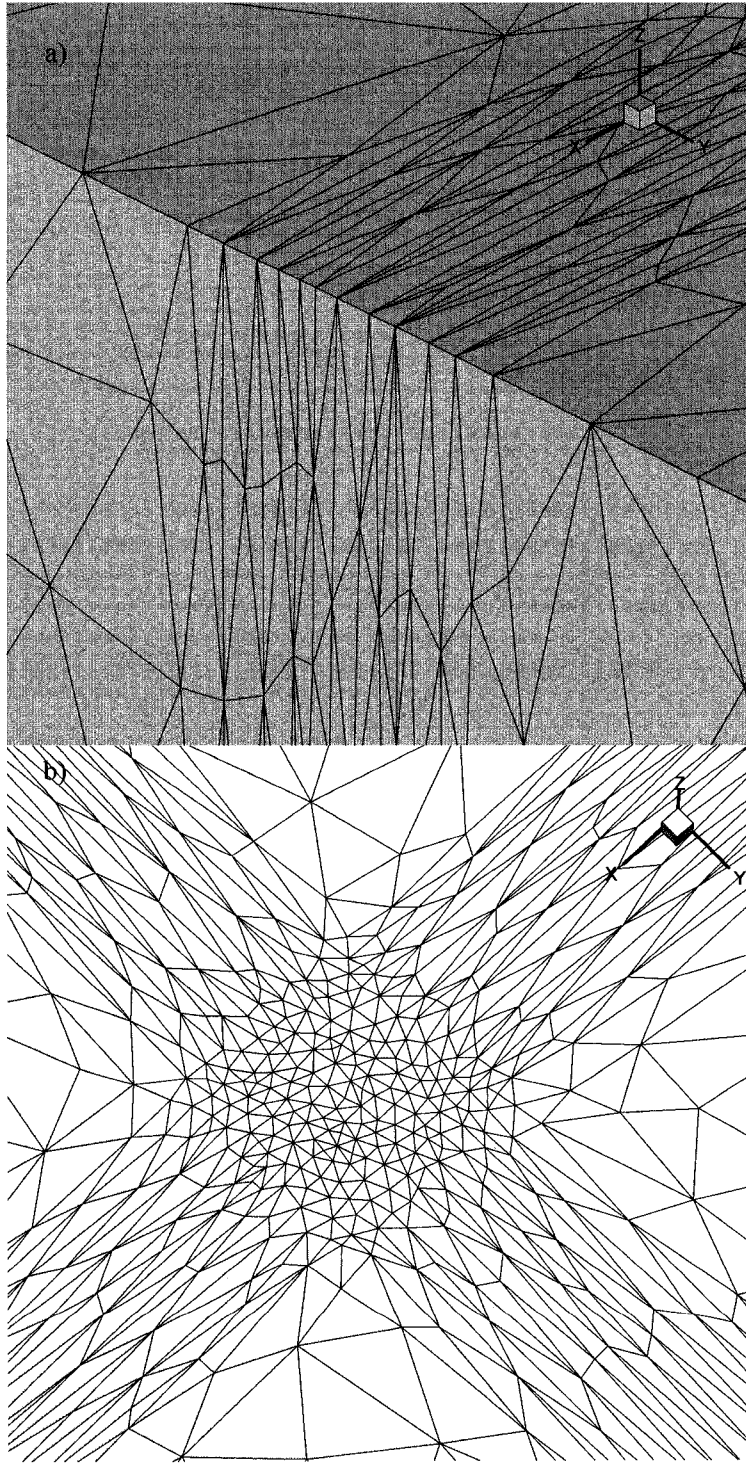
Figure 8.5: Analytic metric 3-D. Details of mesh faces corresponding to a) x = 1 and z = 1 ; b) z = 1 .
