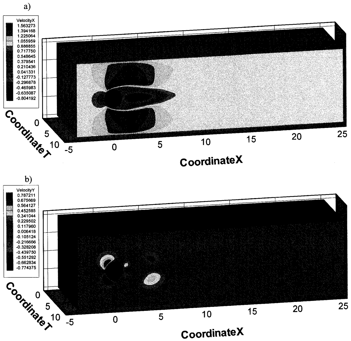
Figure 8.48: Unsteady 2-D flow past a circular cylinder. a) Scalar field for u velocity at t = 10 ; b) scalar field for the v velocity at t = 10 .
