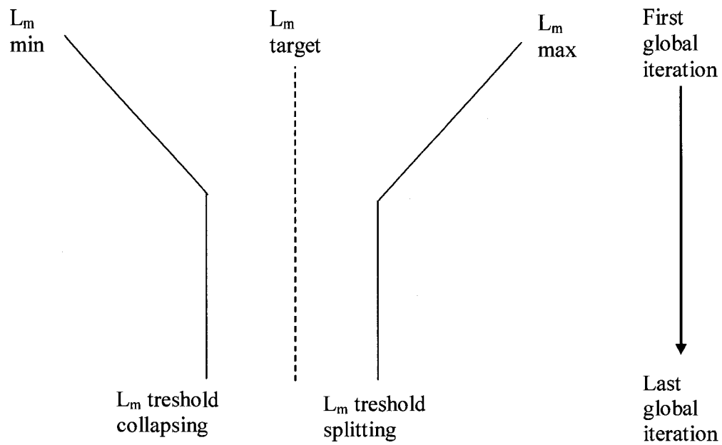
Figure 6.9: Illustrations of the variations of the metric edge length threshold for collapsing, on the left, and refinement, on the right, as the global adaptation iteration progresses from the first iteration on the top to the last iteration at the bottom.
