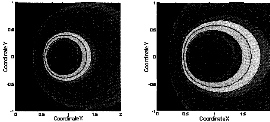
Figure 6.1: Isocontours of the anisotropic measure of quality given by equation 6.1 (left) and its square root (right). The quality is measured for a triangle with two fixed vertices at (0.0, -0.5) and (0.0, 0.5) and a third vertex at the position (x, y) .
