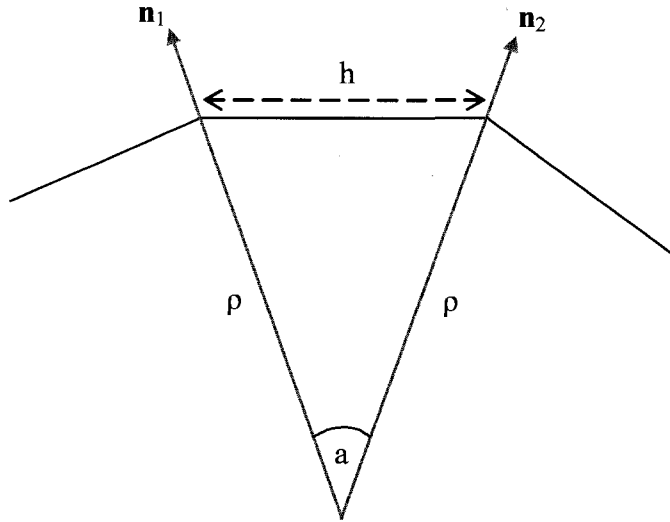
Figure 4.4: Illustration of the point normals and face size used to compute the approximate curvature ( 1/\rho ).
