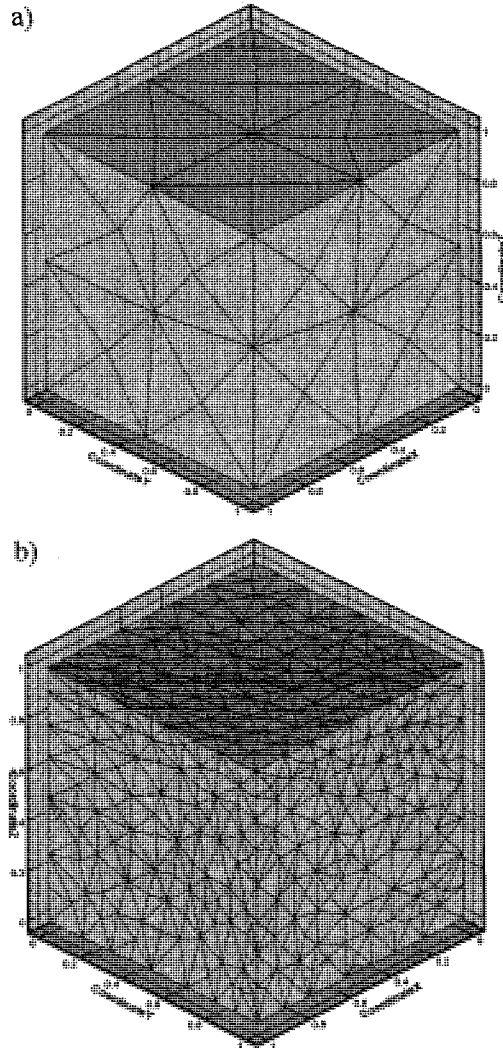
Figure 8.23: Unsteady 3-D heat transfer. a) Initial mesh at t = 0 ; b) adapted mesh at t = 0 .
