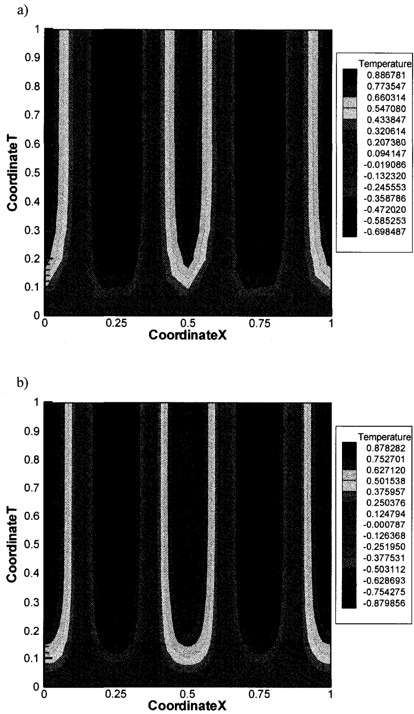
Figure 8.14: Unsteady 1-D heat transfer. a) Initial temperature field; b) adapted temperature field.
