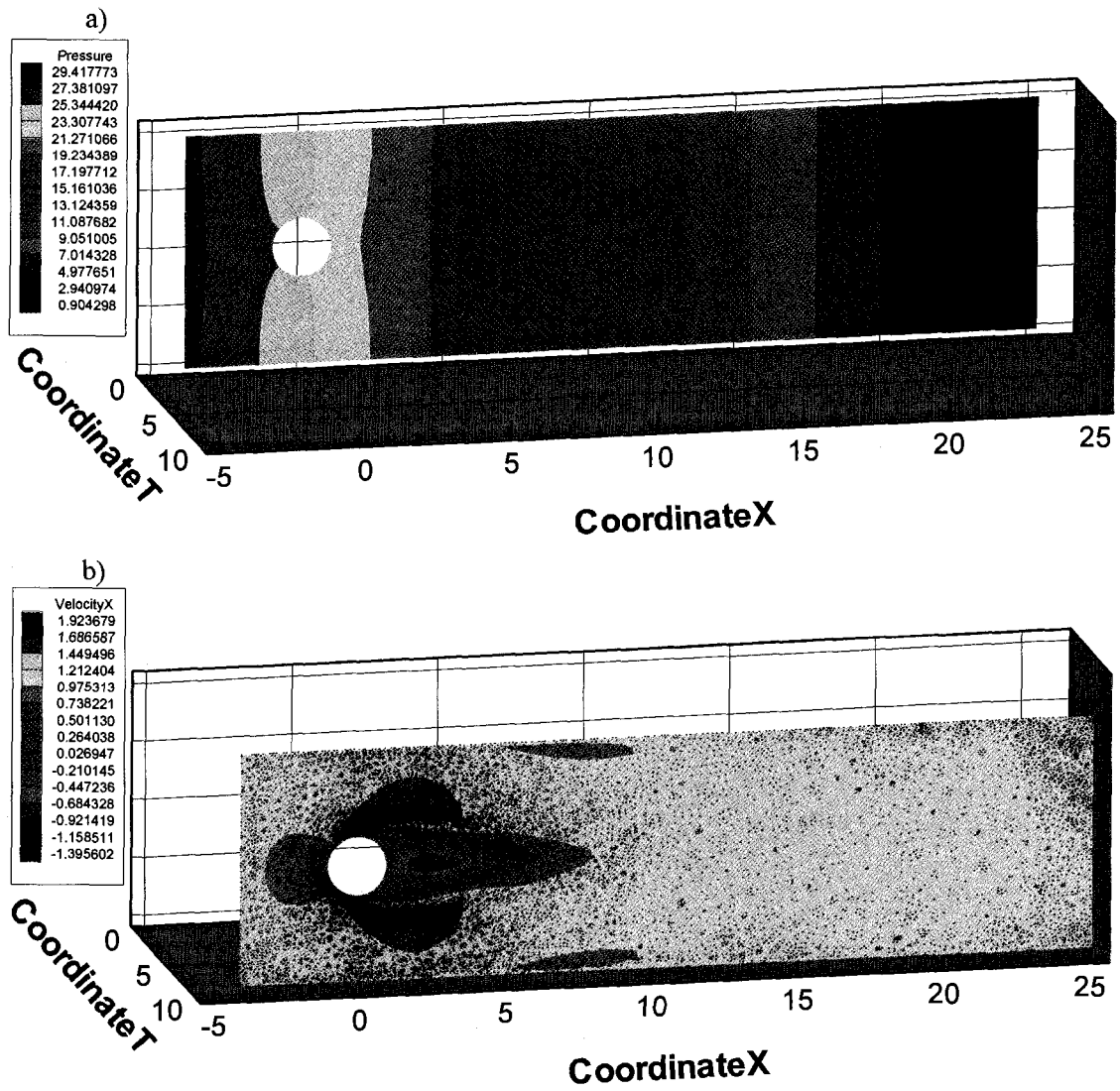
Figure 8.50: Unsteady 2-D flow past a circular cylinder. a) Pressure isocontours at t = 0.2 ; b) isocontours of u and velocity vector field at t = 9.9 .
