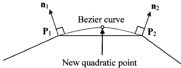
Figure 4.5: Illustration of the Bezier curve used to compute the additional point required to form a quadratic edge on the boundary. The Bezier curve passes through both end points of the linear edge and is perpendicular to the normals at these points.
