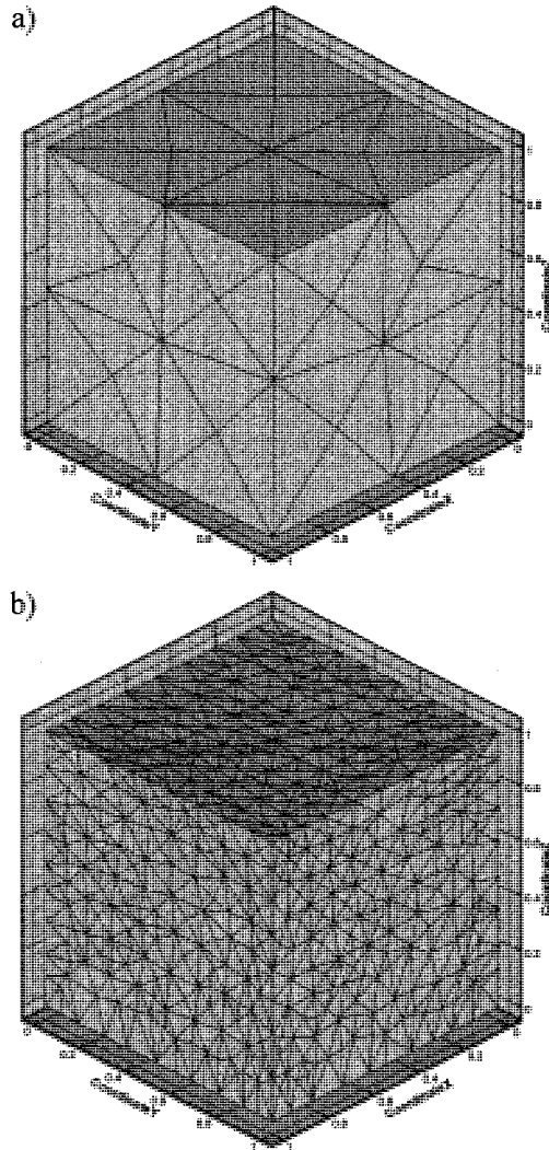
Figure 8.24: Unsteady 3-D heat transfer. a) Initial mesh at t = 1 ; b) adapted mesh at t = 1 .
