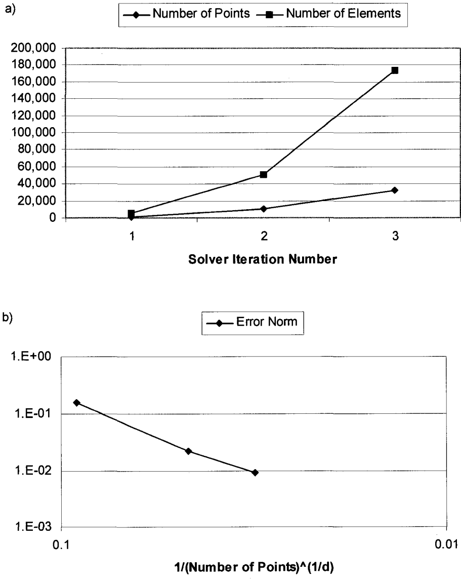
Figure 8.22: Unsteady 2-D heat transfer. a) Numbers of mesh points and elements; b) L^2 error norm as a function of 1/N_p^{1/d} .
