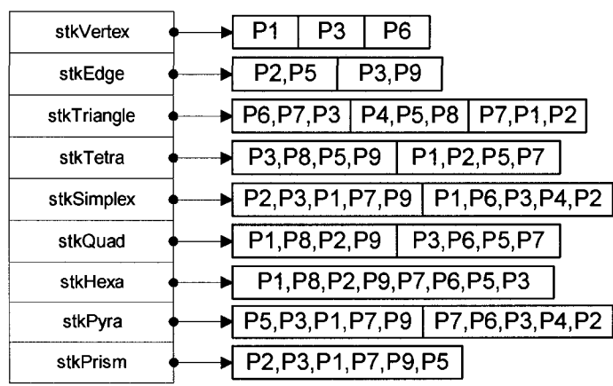
Figure 3.4: Illustration of the element types supported by STK along with their local node numbering.
