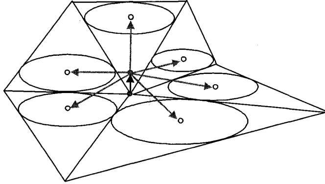
Figure 6.12: Illustration of the point relocation strategy based on the average inscribed ellipsoid of the elements incident to a point. The dark arrow shows the potential displacement from the previous point location to the new trial point location.
