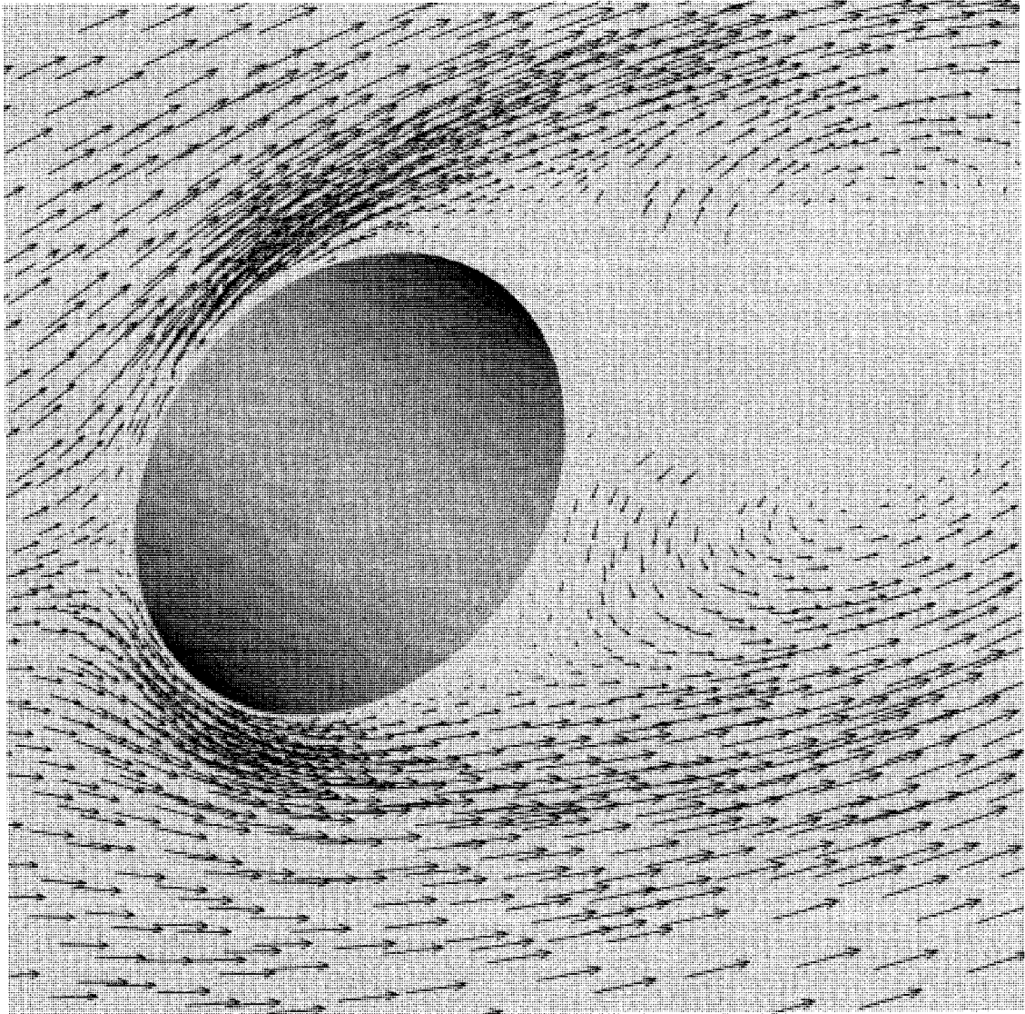
Figure 8.49: Unsteady 2-D flow past a circular cylinder. Detail of the velocity vector field near the cylinder at t = 10 .
