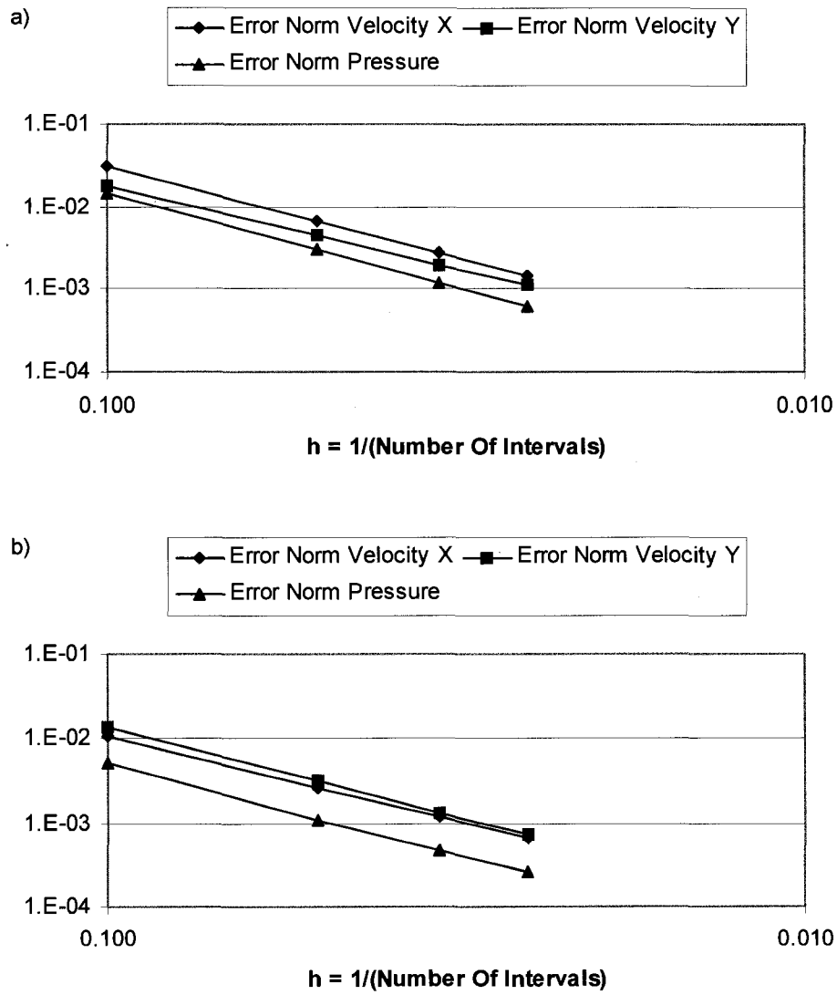
Figure 8.31: Steady and unsteady 2-D flow in a cavity. L^2 error norm as a function of the characteristic mesh size for a) the steady case and b) the unsteady case.
