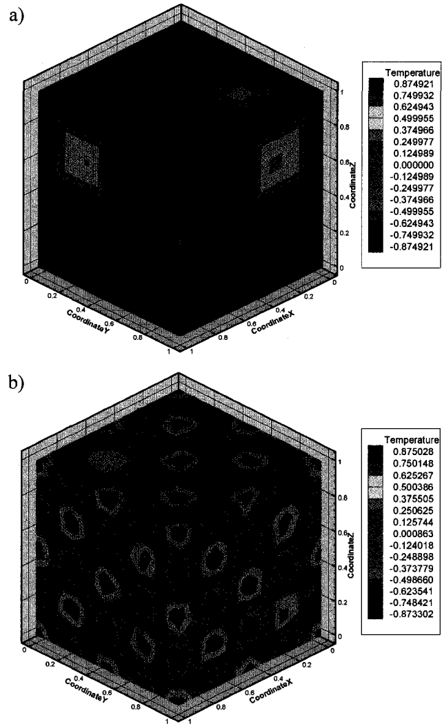
Figure 8.25: Unsteady 3-D heat transfer. a) Initial temperature field at t = 1 ; b) adapted solution at t = 1 .
