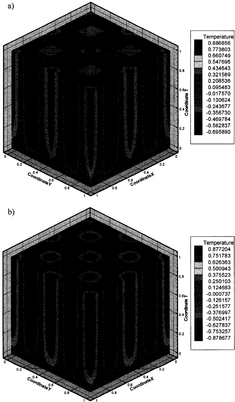
Figure 8.19: Unsteady 2-D heat transfer. a) Initial temperature field; b) adapted temperature field.
