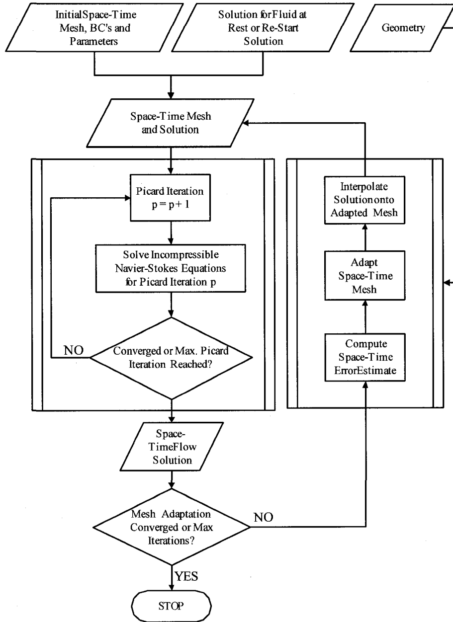
Figure 7.5: Schematic representation of the combined space-time FEM solver and the space-time mesh adaptation procedures.
