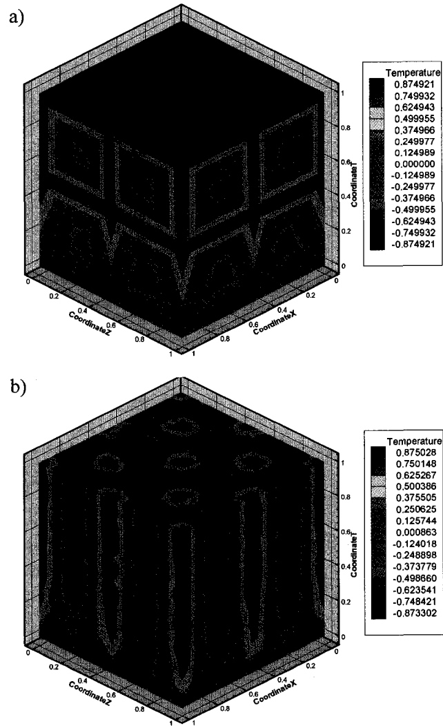
Figure 8.27: Unsteady 3-D heat transfer. a) Initial temperature field at y = 0 ; b) adapted solution at y = 0 .
