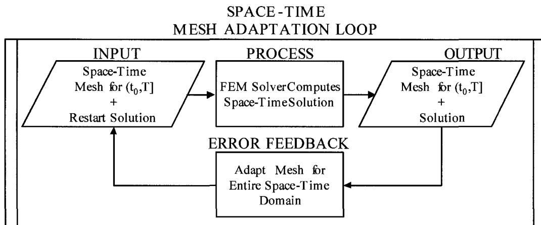
Figure 7.4: Fully coupled space-time mesh adaptation loop, in which the complete space-time solution comprising the entire time range is recomputed at each mesh adaptation iteration.
