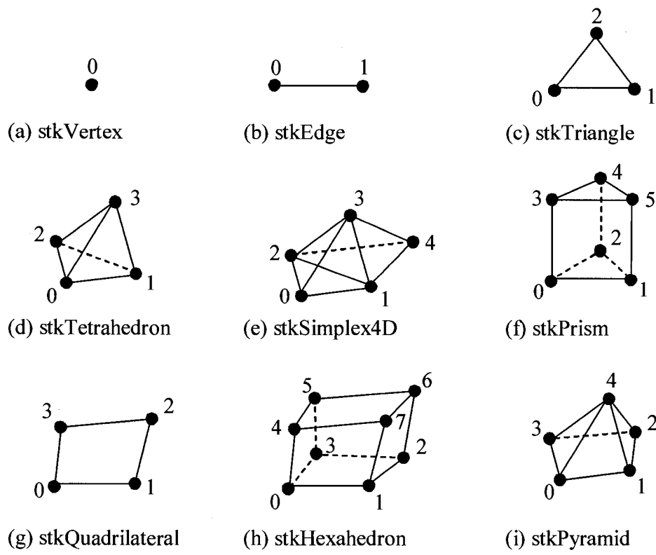
Figure 3.4: Illustration of the element types supported by STK along with their local node numbering.
