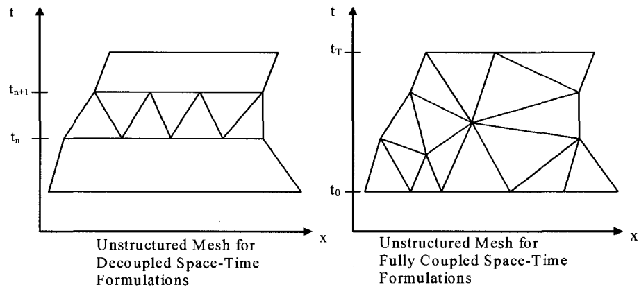
Figure 5.1: Illustration of representative meshes for a space-time slab ( left) and a fully coupled, or time-continuous, space-time mesh (right).
