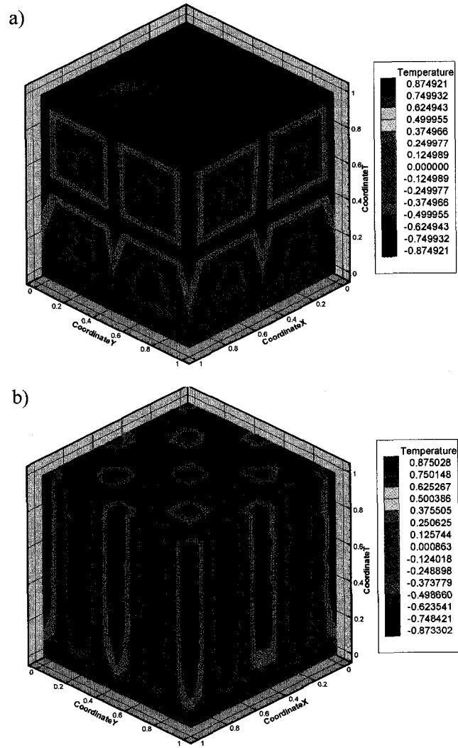
Figure 8.28: Unsteady 3-D heat transfer. a) Initial solution at z = 0 ; b) adapted solution at z = 0 .
