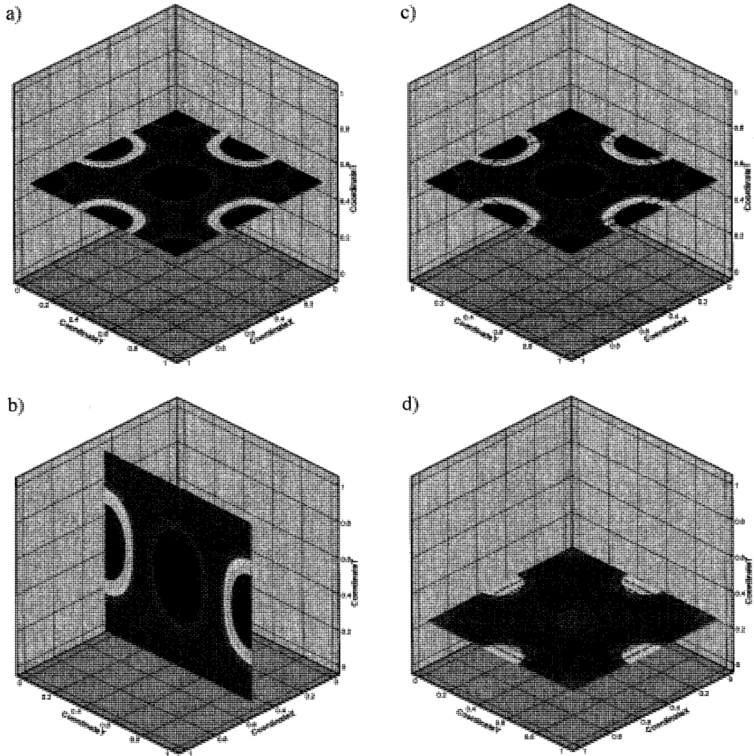
Figure 8.40: Unsteady 2-D flow in a cavity. a) Pressure at t = 0.5 ; b) pressure at x = 0.5 ; c) streamlines and pressure at t = 0.5 ; d) streamlines and pressure at t = 0.25 .
