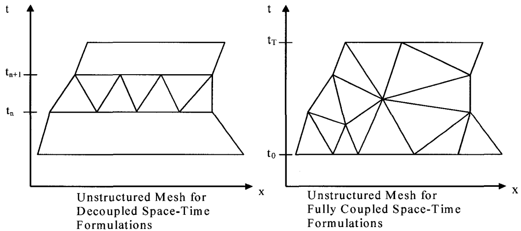
Figure 7.1: Illustration of a decoupled space-time mesh (left side) and a fully coupled space-time mesh (right side).
