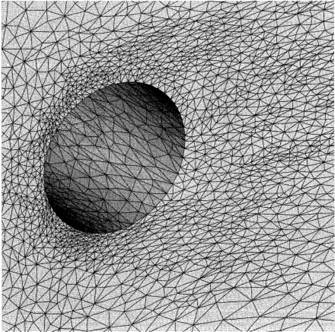
Figure 8.47: Unsteady 2-D flow past a circular cylinder. Detail of the adapted mesh near the cylinder at t = 10 .
