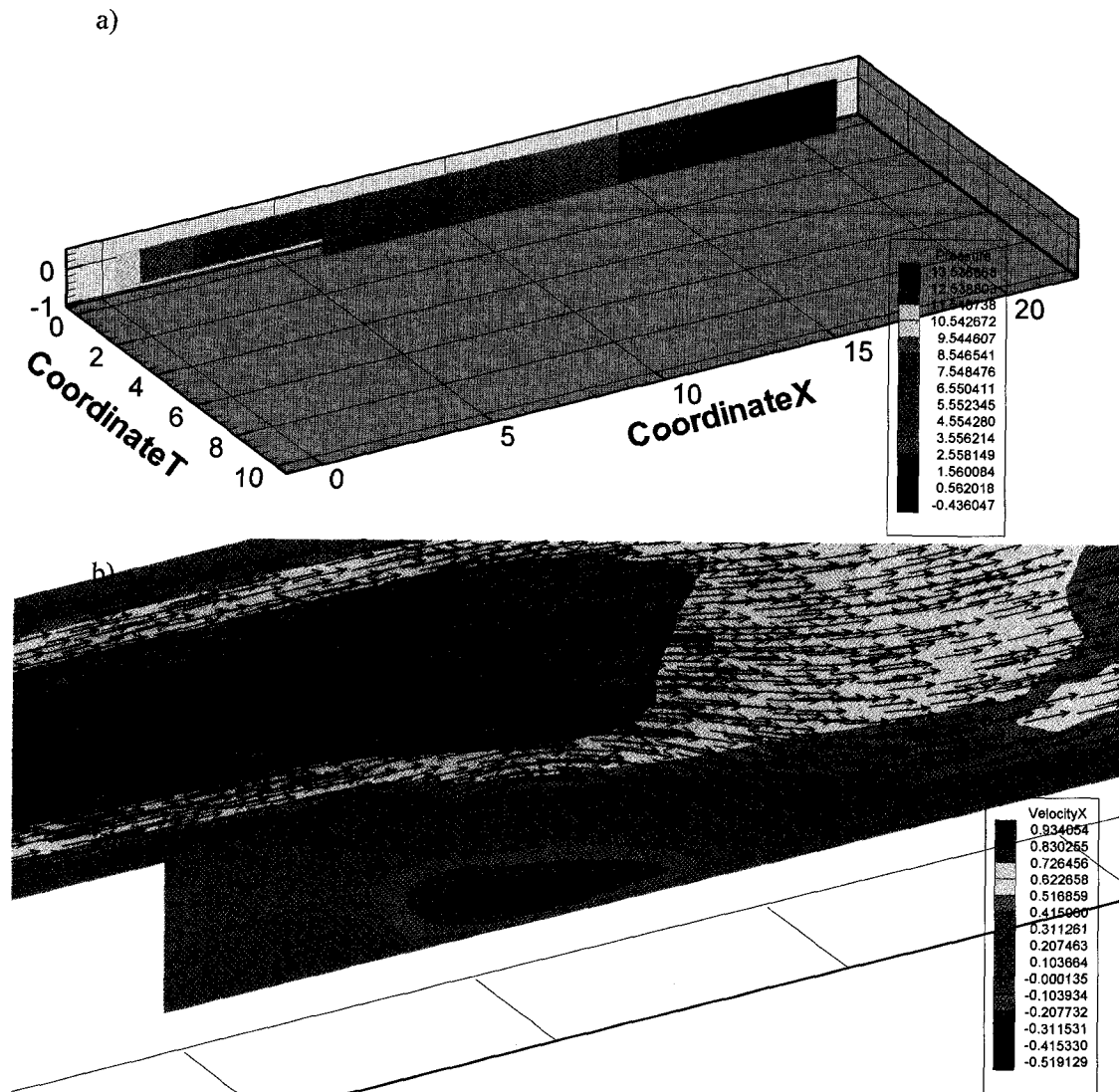
Figure 8.57: Unsteady 2-D flow past a back-facing step. a) Pressure contours at t = 0.2 ; b) u contours and velocity vectors at t = 9.9 .
