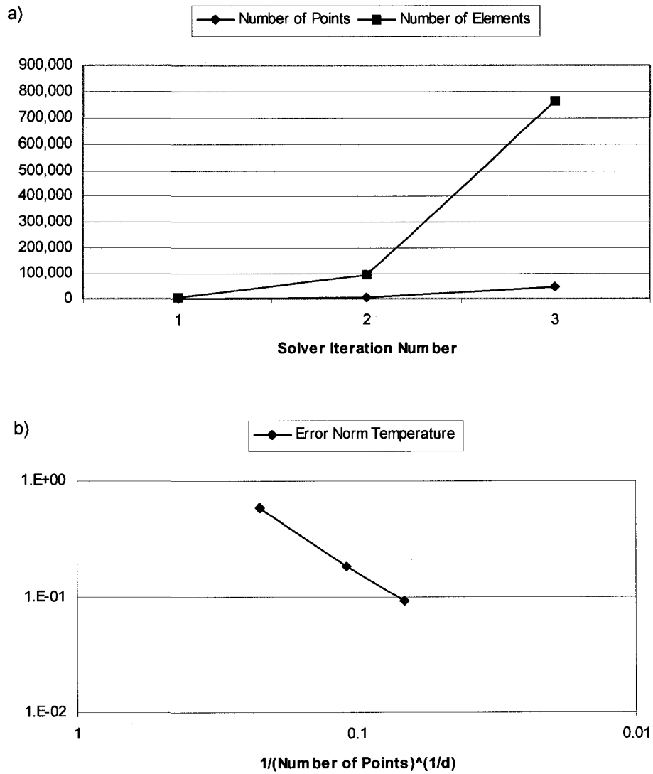
Figure 8.30: Unsteady 3-D heat transfer. a) Numbers of mesh points and elements; b) L^2 error norm as a function of 1/N_p^{1/d} .
