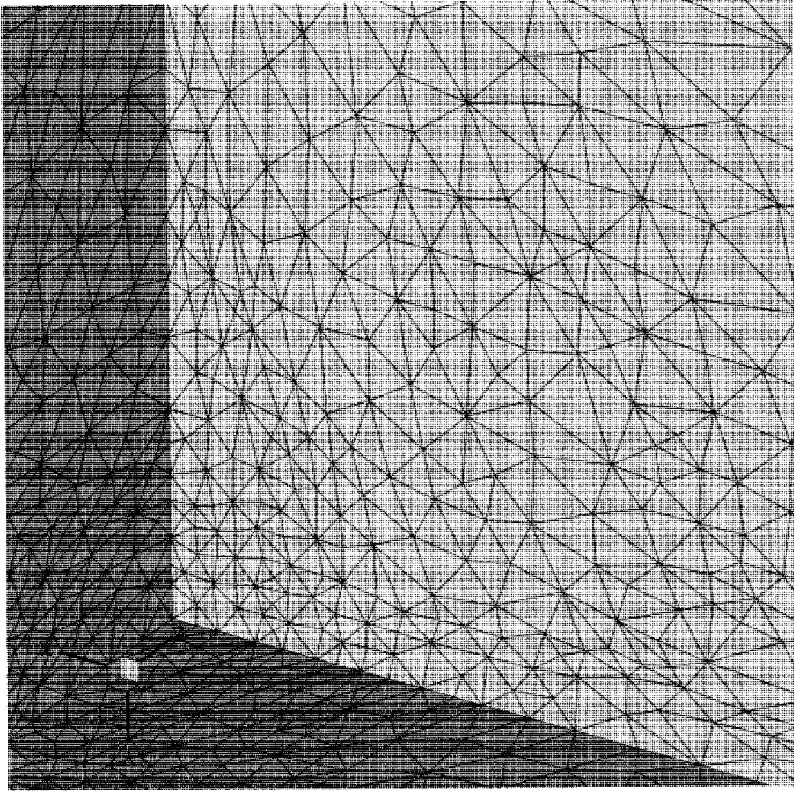
Figure 8.62: Unsteady 2-D flow in a lid-driven cavity. Adapted mesh near the point (1, 1, 1), in which the z axis corresponds to time.
