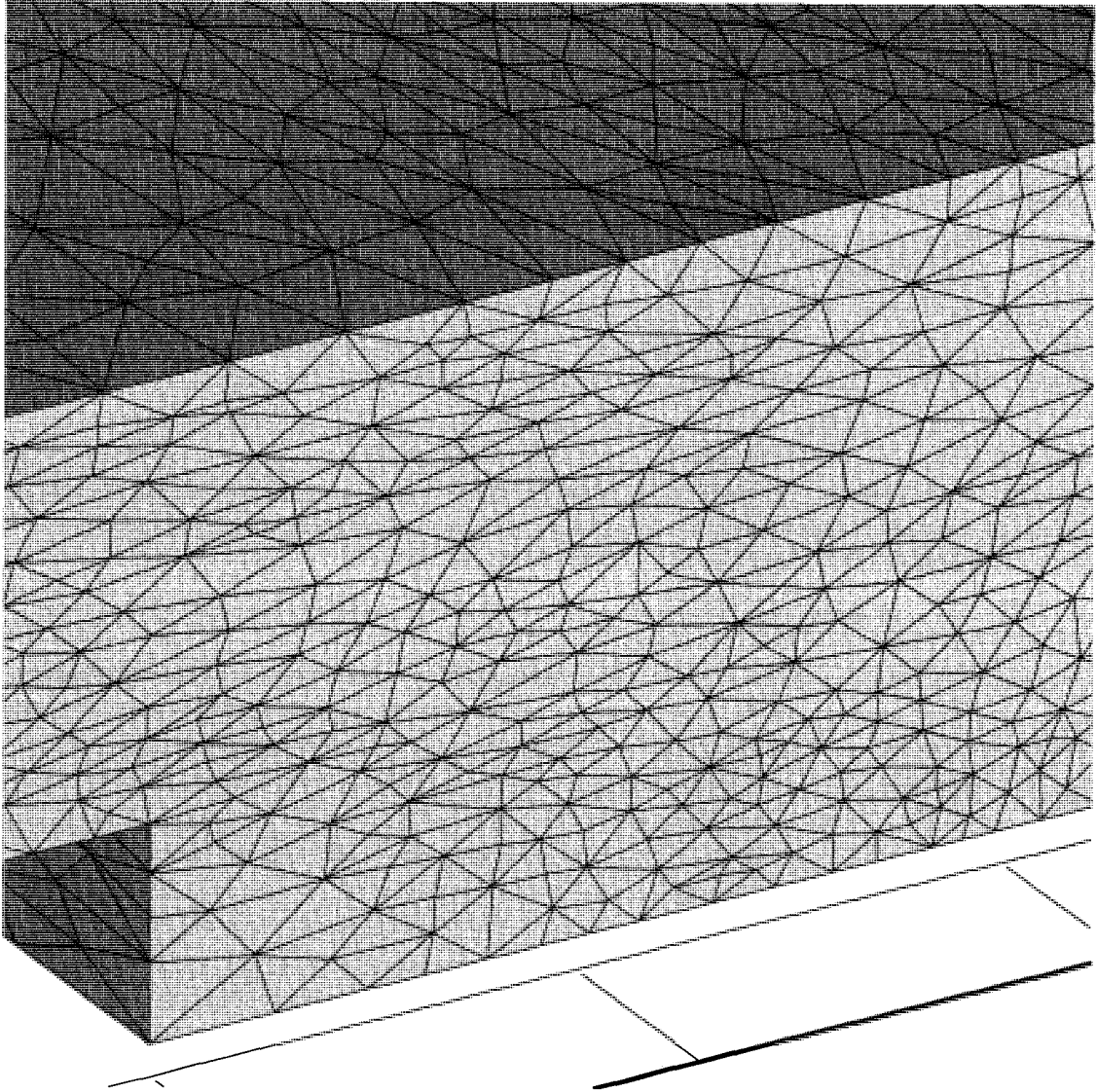
Figure 8.55: Unsteady 2-D flow past a back-facing step. Adapted mesh near the step at t = 10 .
