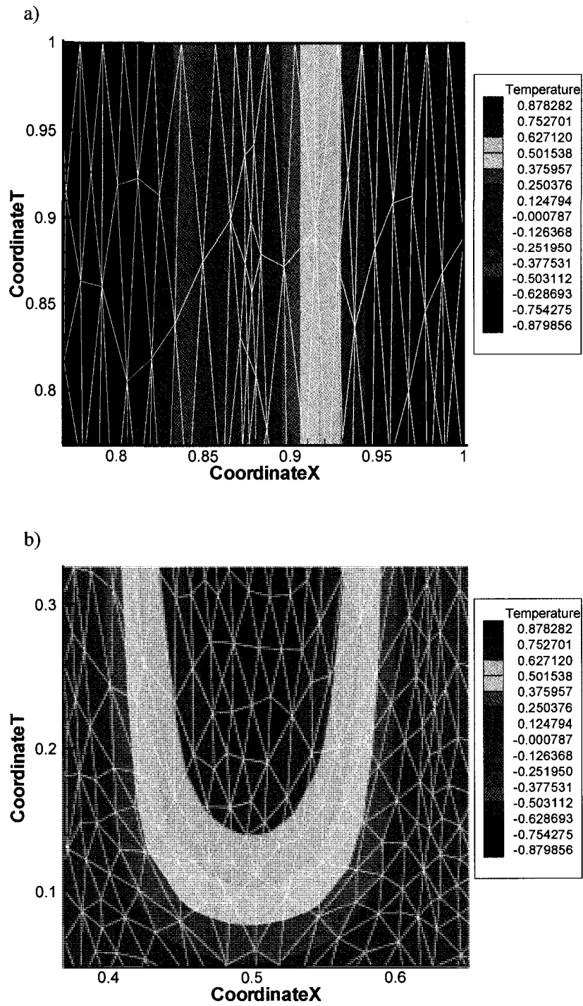
Figure 8.15: Unsteady 1-D heat transfer. a) Temperature field and mesh near corner point (1,1); b) temperature field and mesh near point (0.5,0.2).
