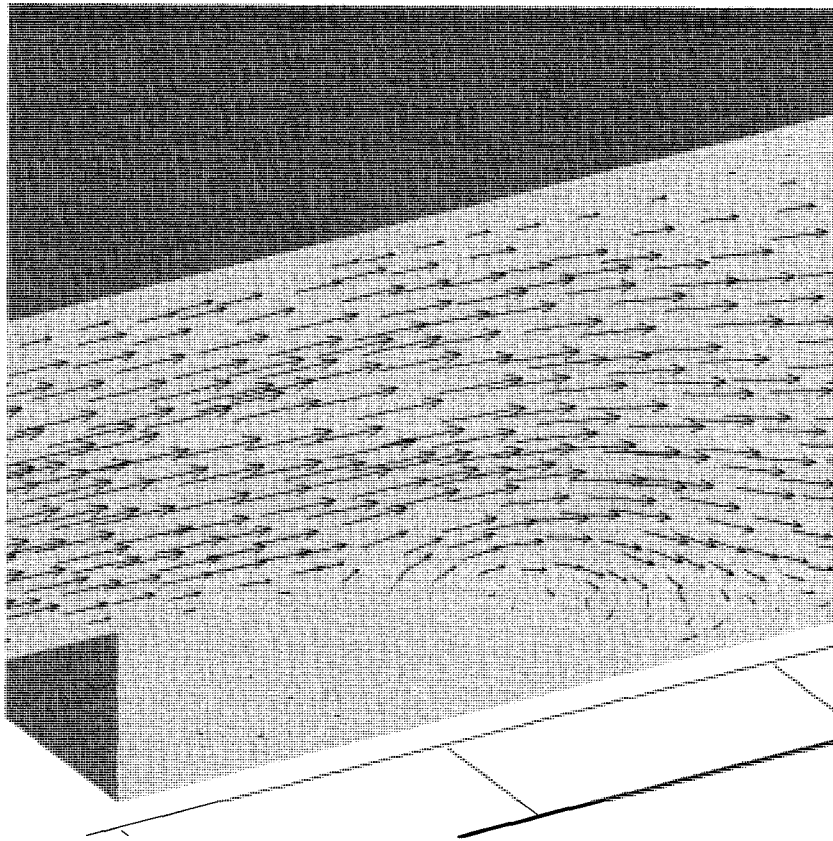
Figure 8.56: Unsteady 2-D flow past a back-facing step. Velocity vectors near the step at t = 10 .
