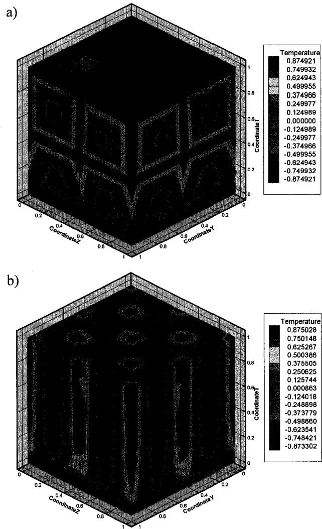
Figure 8.26: Unsteady 3-D heat transfer. a) Initial temperature field at x = 0 ; b) adapted solution at x = 0 .
