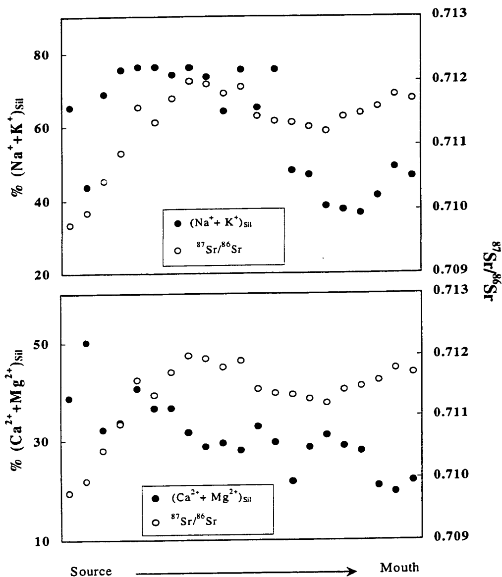
Fig. 6.18. Percent silicate derived \text{Na}^+ + \text{K}^+ and ^{87}\text{Sr}/^{86}\text{Sr} (top), percent silicate derived \text{Ca}^{2+} + \text{Mg}^{2+} and ^{87}\text{Sr}/^{86}\text{Sr} (bottom) for the Indus main channel during the winter. The arrow points in the direction of the flow of Indus.
