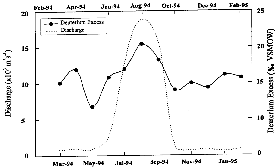
Fig. 4.6. Monthly time series for instantaneous discharge and deuterium excess ( d = \delta\text{D}-8 (\delta^{18}\text{O}) ) at the Sukkur barrage. Discharge data from WAPDA, unpublished records.
