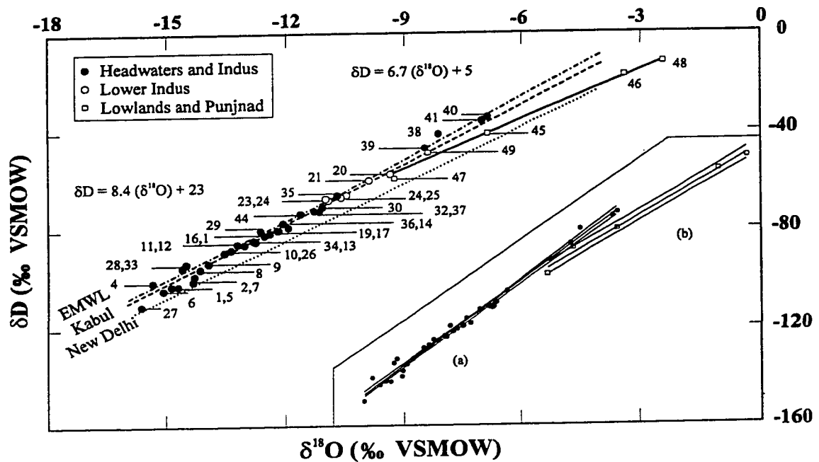
Fig. 4.3. Scatter plot of \delta D versus \delta^{18}O of water samples collected from the Indus River Basin during the summer. Dashed lines are Local Meteoric Water Lines: EMWL, Eastern Meteoric Water Line, \delta D = 8.08\delta^{18}O + 22 (Gat and Carmi, 1970); Kabul, \delta D = 8.01\delta^{18}O + 19 ; and New Delhi, \delta D = 7.68\delta^{18}O + 7 (IAEA-WMO). The solid line is a least square fit through the lowland tributaries + the Panjnad. Regression line through the headwaters + the Indus has been omitted for clarity. Note that the equation given for the headwaters and the Indus does not include samples downstream from Panjnad. The inset (a) and (b) shows the upper and lower confidence limits at the 95% significance level for the headwaters + Indus and the lowland tributaries + Panjnad respectively. Confidence limits established following the method described in Payne (1992). The Key to the sample numbers as in Fig. 3.1.
