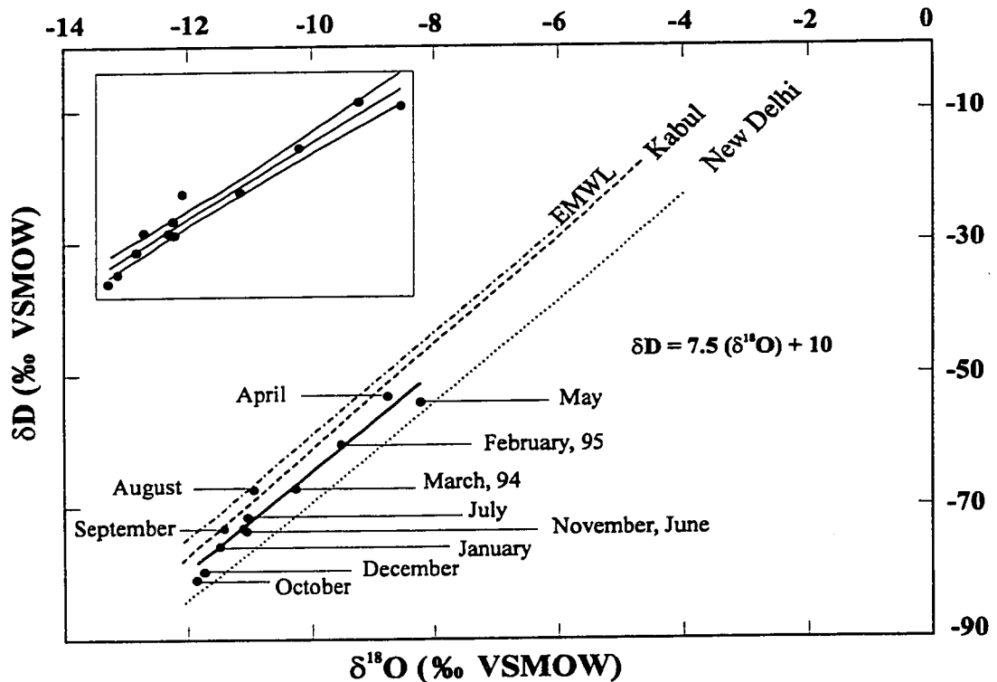
Fig. 4.5. Scatter plot of \delta\text{D} vs \delta^{18}\text{O} for time series at the Sukkur barrage. The solid line is regression through the data. Dashed lines are Local Meteoric Water Lines: EMWL, Eastern Meteoric Water Line, \delta\text{D} = 8.08\delta^{18}\text{O} + 22 (Gat and Carmi, 1970); Kabul, \delta\text{D} = 8.01\delta^{18}\text{O} + 19 ; and New Delhi, \delta\text{D} = 7.6\delta^{18}\text{O} + 7 (IAEA-WMO). The heavy line is a least square fit through the data points. The inset shows the upper and lower confidence limits at the 95% significance level on the regression. Confidence limits established following the method described in Payne (1992).
