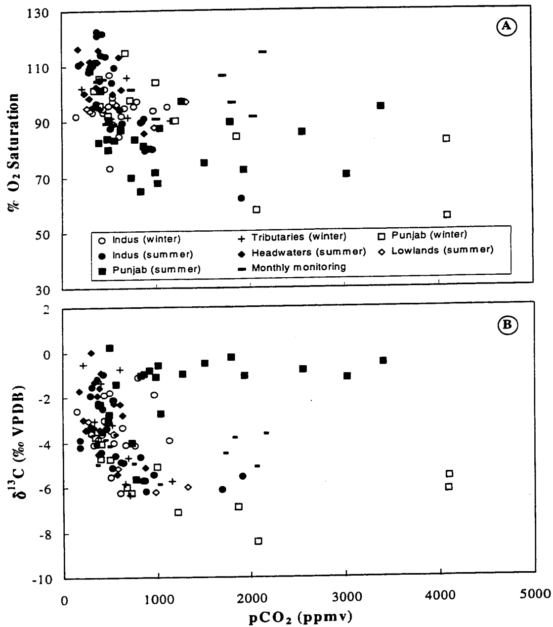
Fig.6.6. Percent oxygen saturation (A) and \delta^{13}\text{C} of DIC (B) versus p\text{CO}_2 for the Indus River Basin.
