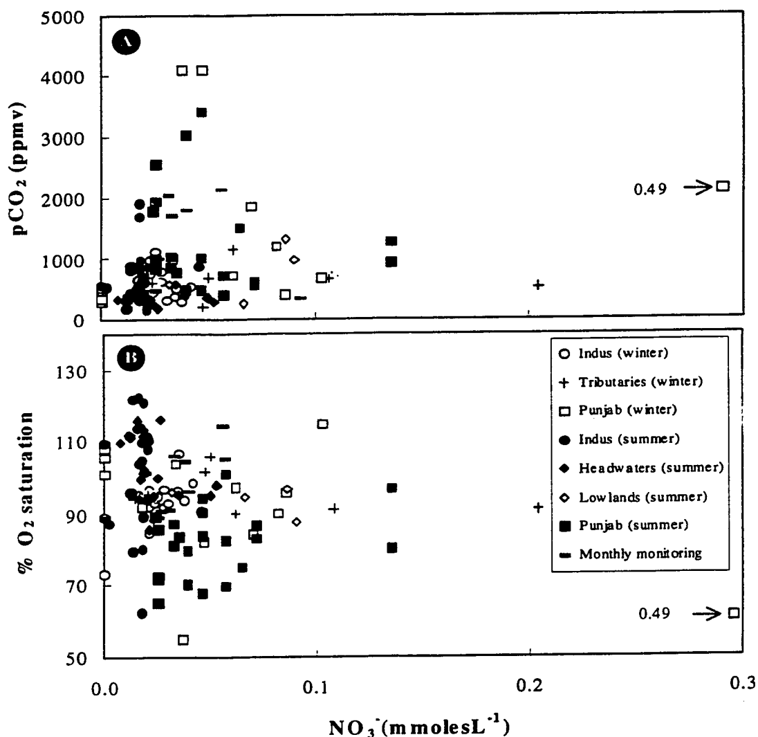
Fig. 6.9. \text{pCO}_2 (A) and percent oxygen saturation (B) versus nitrate concentration for the Indus River Basin.
