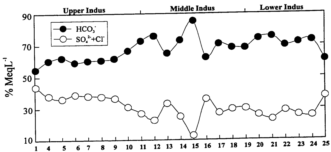
Fig. 5.8. Major anion concentrations and dissolved silica for the Indus main channel during the summer season. All ions expressed in percent meqL -1 except for Si that is in mmolL -1 . The key to the sample numbers as in Fig. 3.1
