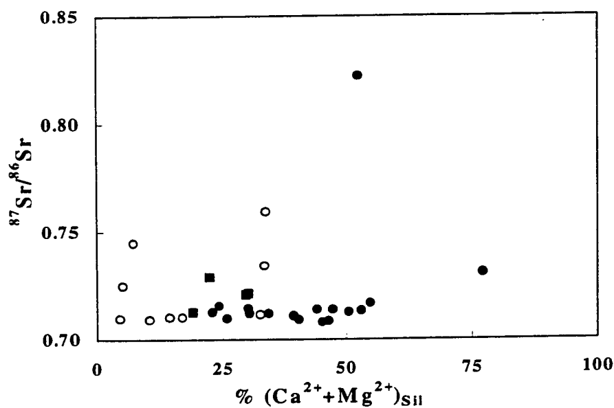
Fig. 6.20. Scatter plot of \% (Ca^{2+} + Mg^{2+})_{Sil} versus ^{87}Sr/^{86}Sr for the headwater tributaries and the Punjab rivers of the Indus River Basin during the summer. Note that only the lower order headwater tributaries in Pande et al. (1994), not sampled during the present study, are shown. In the former study, two samples with negative charge balance have been excluded. The key to the samples as in Fig. 6.19.
