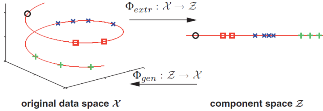
Figure 3.2 Non-linear dimensionality reduction in NLPKA (source: Scholz et al. , 2007)
