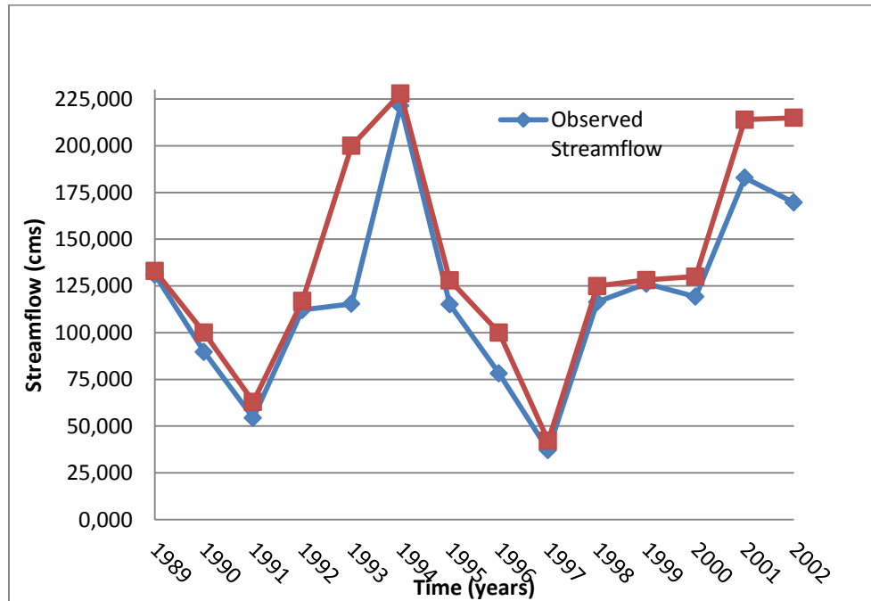
Figure 6.5 Observed and simulated streamflows (1989-2002)
