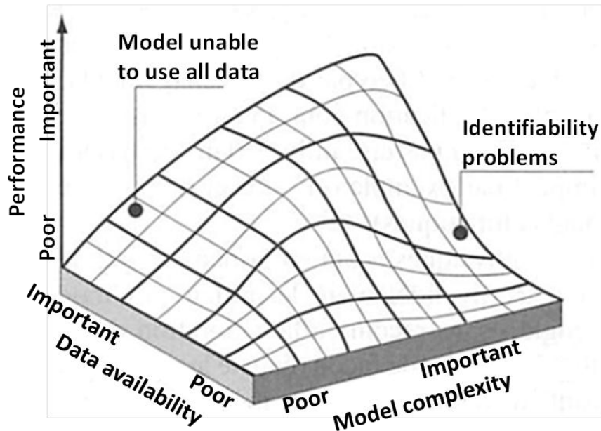
Figure 3.5 Schematic diagram of the relationship between complexity and performance of a hydrological model and data availability (adapted from Grayson & Blöschl, 2000)
