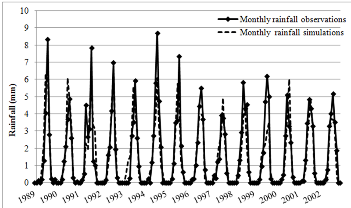
Figure 6.4 Observed and simulated rainfall using method of fragment (1989-2003)
