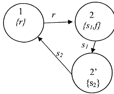
Figure 18. ESMP
