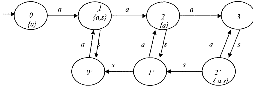
Figure 4. G/G/1/
