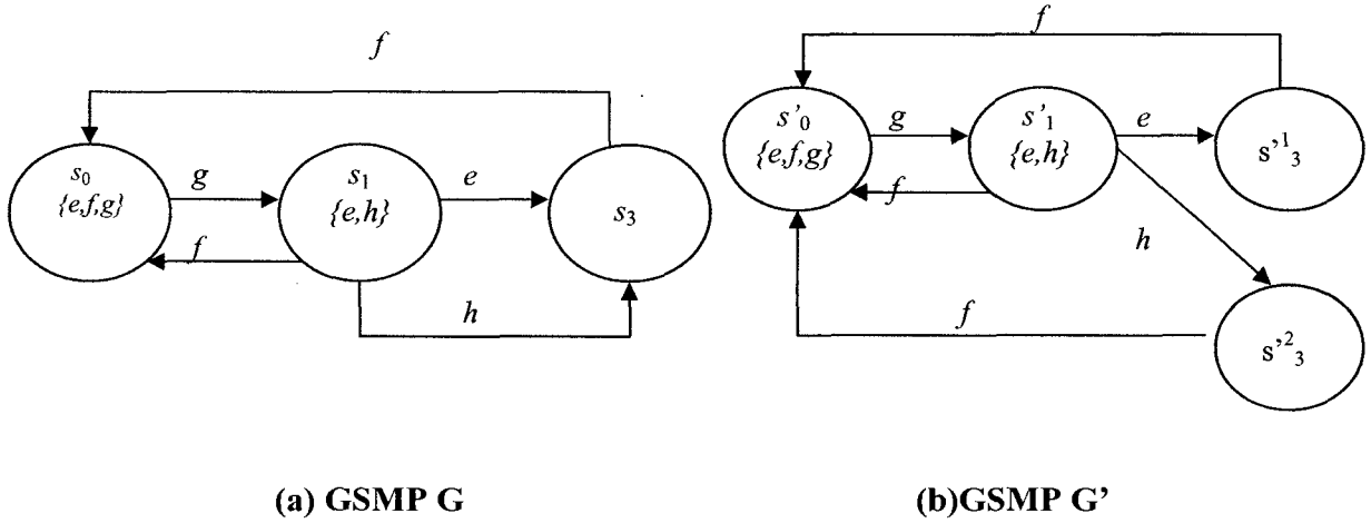
Figure 5. Two GSMPs
