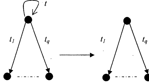
Figure 16. Cycle removal
