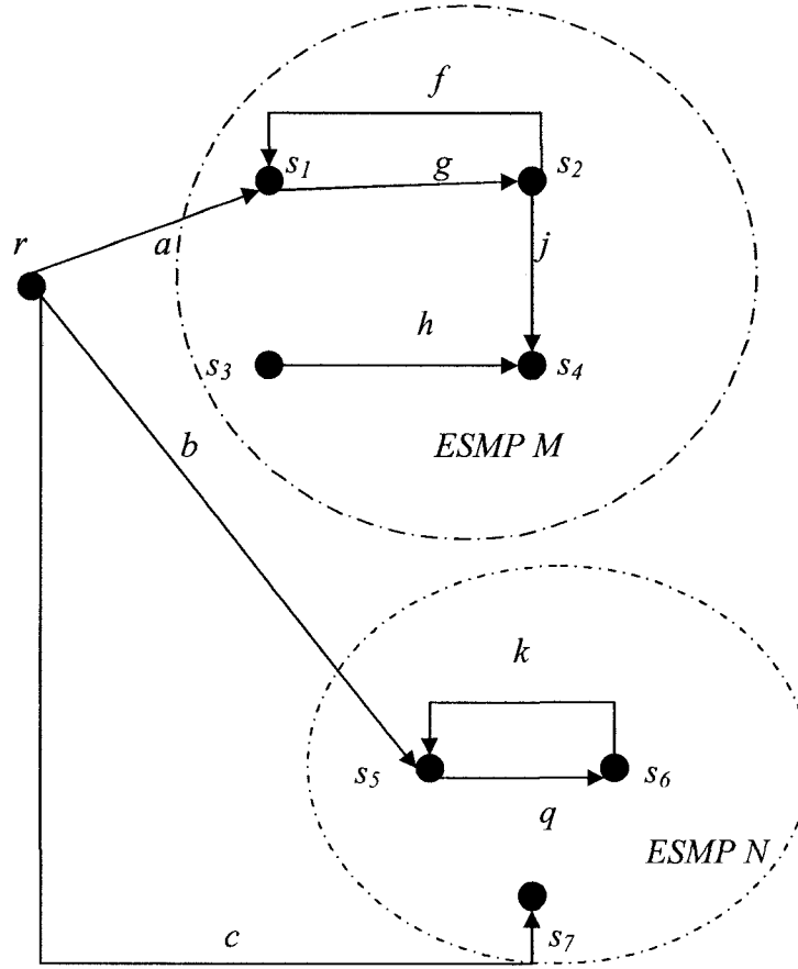
Figure 7. Nest
