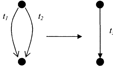
Figure 15. Alternate reduction
