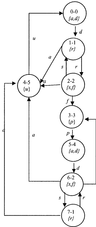
Figure 9. An HMRP
