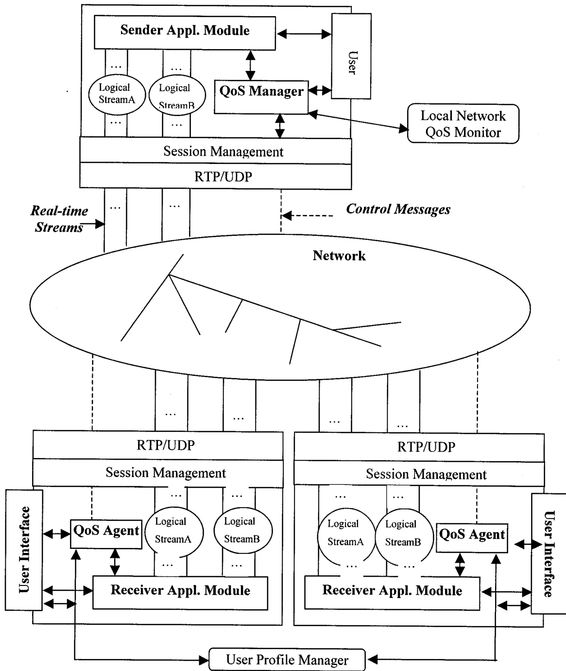
Figure 3.1. General System Architecture for Teleteaching Application Using MPEG-4/DMIF
