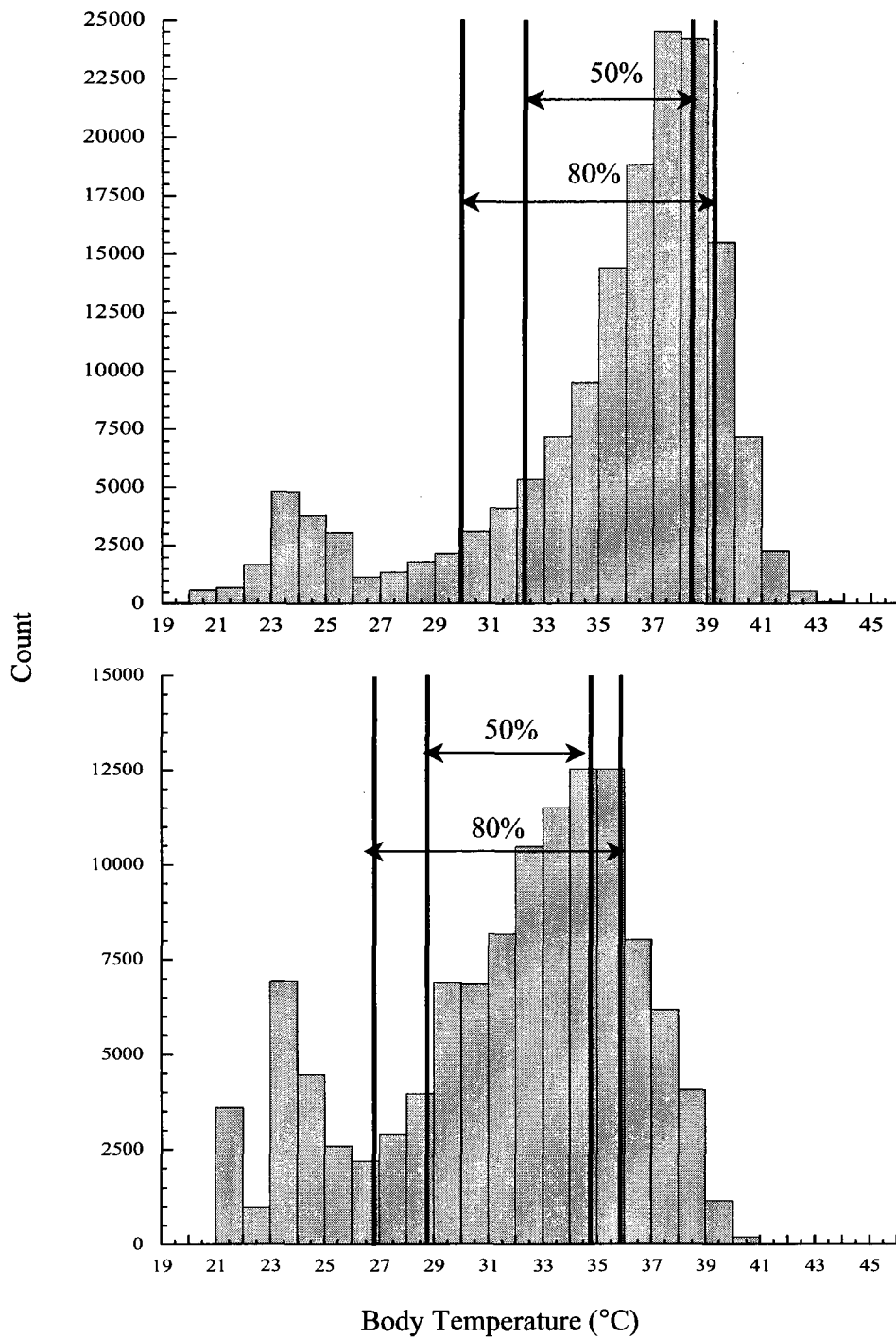
Figure 2-2: Body temperature distributions from thermal gradient for (A) fed (n = 12) and (B) fasted (n = 10) P. vitticeps . Vertical lines delineate the T set s given by the central 50% and 80% T b distributions.
