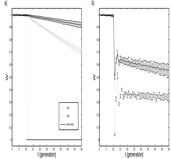
FIG. 6. Effect of network topology and fitness threshold on reproductive fitness ( W ). W for each of the DA, FFL, and FFL+PFL populations over 50 generations. Drug treatment is initiated at the tenth generation. (a) Population simulations using a step fitness function. (b) Population simulations performed using a Hill type fitness function. Parameters were set to: x = 1 , \alpha_y = 10 , \alpha_z = 100 , K = 1 , and n = 2 . In (a) z_c = 35 and in (b) K_w = 35 , and n_w = 2 . 10 realizations of 1000 cells were performed. Error bars show standard deviation.
