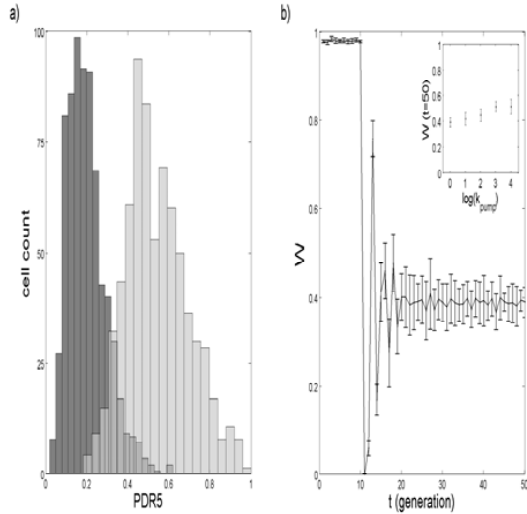
FIG. 7. Adaptation and fitness ( W ) facilitated by the PDR5 transcriptional network. (a) Number of cells in the population has the corresponding PDR5 expression level. Distributions are shown for the generation prior (dark gray) to drug application and 40 generations after (light gray) drug application. (b) W over 50 generations. Inset shows W at generation 50 for different rates of PDR5 mediated drug efflux ( k_{pump} ). Drug treatment is initiated at the tenth generation. Unless otherwise indicated, parameters were set to: \alpha_0 = 1 , \alpha_1 = 10 , K_1 = 1 , n_1 = 1 , \alpha_3 = 10 , K_3 = 1 , n_3 = 2 , \alpha_5 = 100 , K_5 = 20 , n_5 = 2 , k_{diff} = 100 , k_{pump} = 1 , and drug_{ext} = 100 . 10 realizations of 1000 cells were performed.
