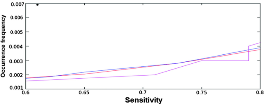
Figure 7 Comparison of PWM (mono-nucleotide and di-nucleotide) with the program Match. The OF i and sensitivity comparison for different PWM and Match. Occurrence frequencies are at Y-axis. X-axis denotes the sensitivities. The average OF i of the Match tool is denoted as filled circle (upper left corner). The sensitivity and specificity curve for the PWM obtained from GATA-3 binding sites from Jaspar is represented by blue, red and magenta are of the new mono-nucleotide PWM and di-nucleotide PWM respectively.
