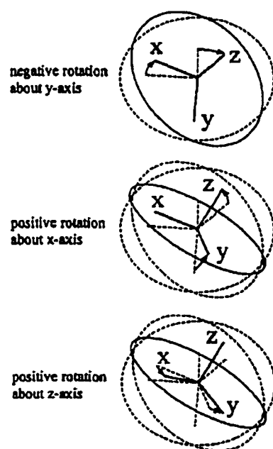
Figure C- 4: Angular descriptions as employed by Segment Analysis
