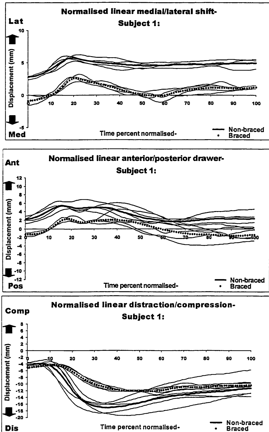
Figure 6 (a): Linear patterns of tibiofemoral joint translations derived from skeletal (femur, tibia) markers. The averages of the trials are displayed in bold. The bold solid line represent the unbraced kinematics, the bold dashed line represent braced kinematics. (a) Subject 1; (b) Subject 3; (c) Subject 4; (d) Subject 6.
