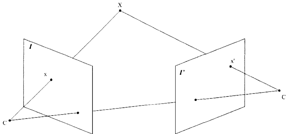
Figure E.1: 3D reconstruction by linear triangulation
