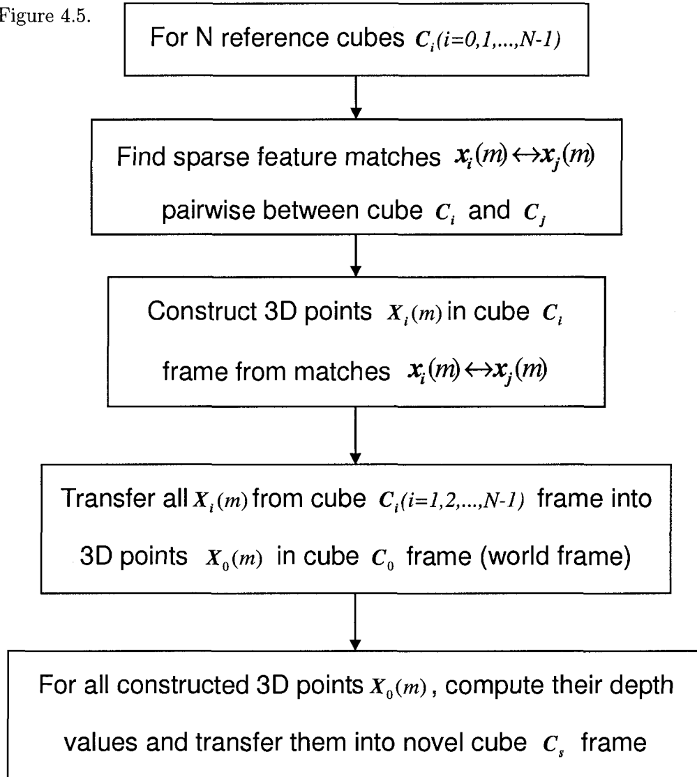
Figure 4.5: Guided depth searching with sparse 3D reconstruction
