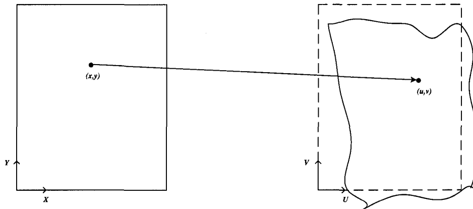
Figure 3.1: Image warping
