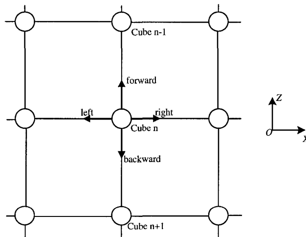
Figure 3.3: Cube navigating
