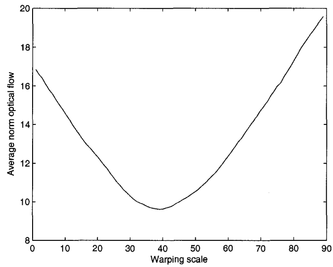
Figure 3.13: The average norm optical flow of different warping scales
