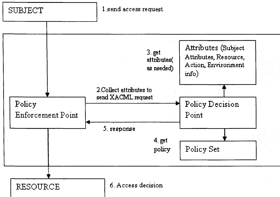
Figure 3: XACML process [42]
