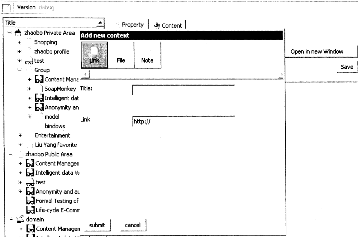
Figure 18 : New Command
