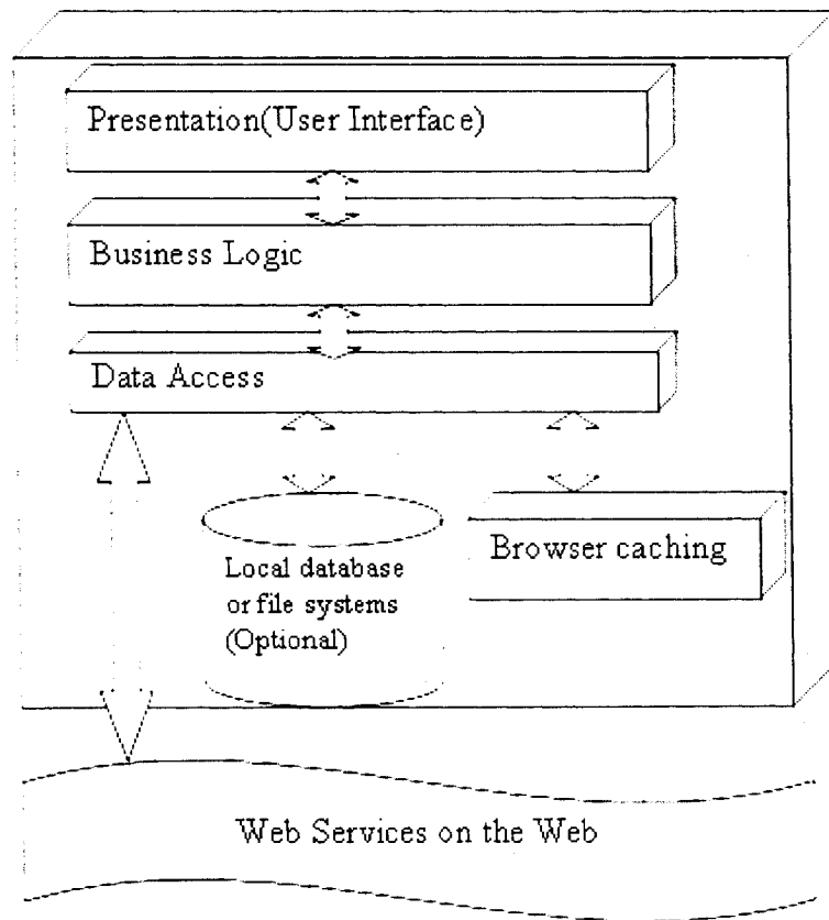
Figure 7: Enriched Web Services Architecture
