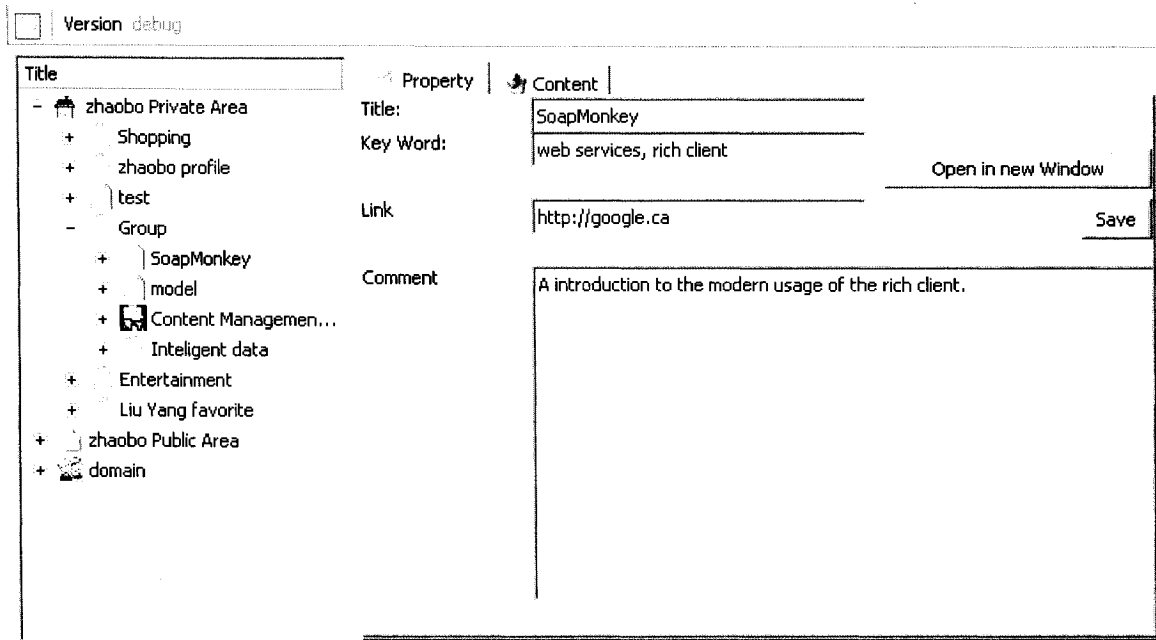
Figure 19 : Property Window
