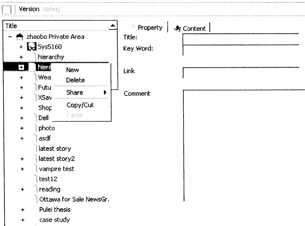
Figure 17 : Popup menu
