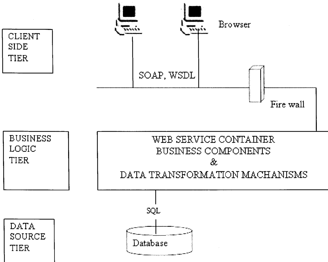
Figure 16: MSC System Architecture.
