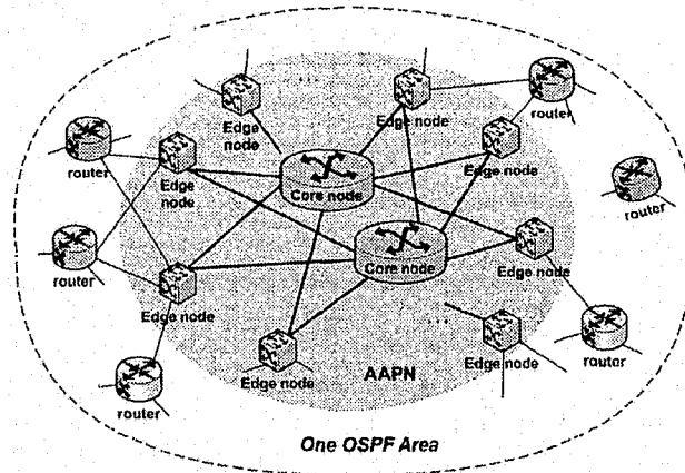
Figure 3.1: Deploying an AAPN in a single OSPF/OSPF-TE area network
