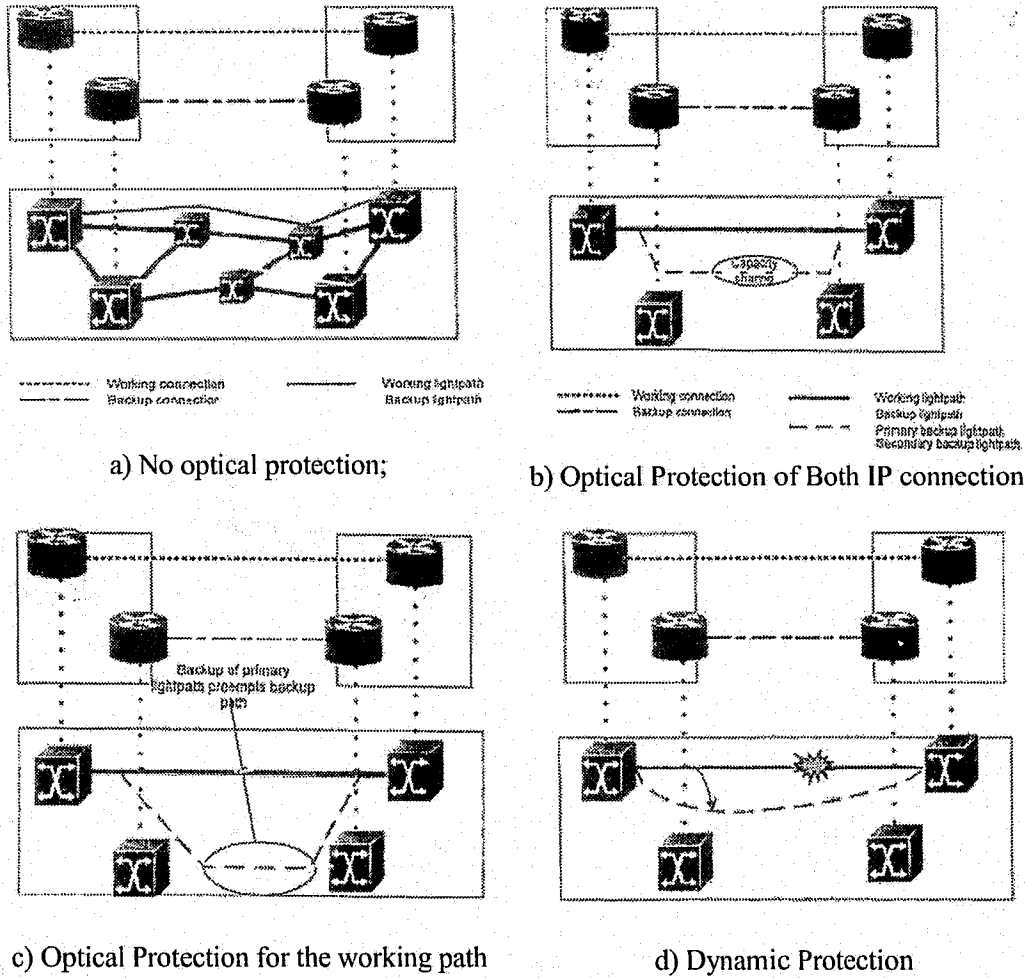
Figure 2.10: Several generic end-to-end recovery techniques in [Staessens2006]
