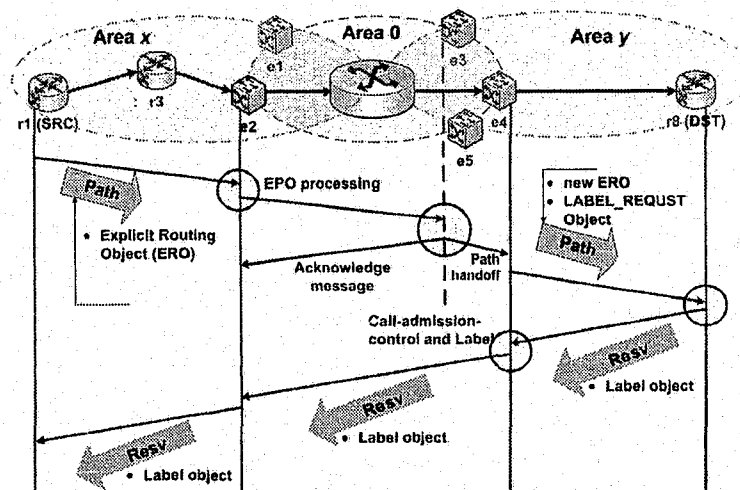
Figure 3.7: Inter-Area LSP Signaling Process that follows RFC 3209
