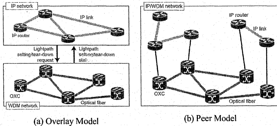
Figure 2.2: Models of IP/MPLS over Optical Networks [Koizumi2006]
