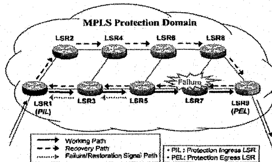
Figure 2.5: Path recovery: Haskin's scheme [Ahn2002].
