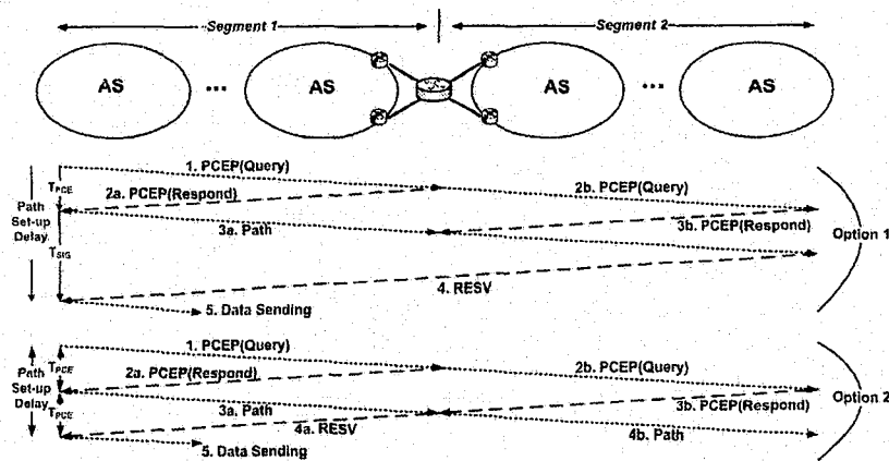
Figure 5.4: Segmented PCE-based architecture
