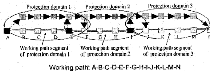
Figure 2.6: Illustration of SLSP [Ho2004a].
