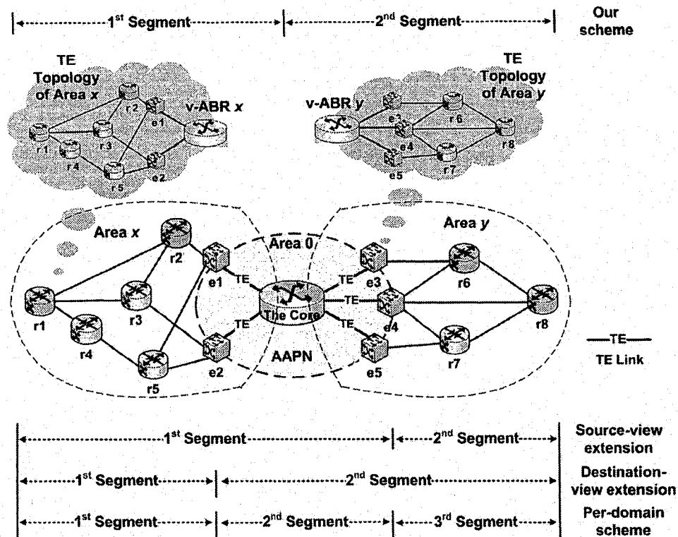
Figure. 3.6: The inter-area optimal routing framework we proposed deploys AAPN as backbone. We also illustrate the per-domain approach and its two extensions.
