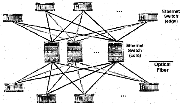
Figure 5.1: Ethernet version of OSN
