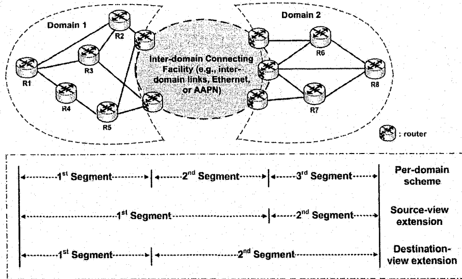
Figure 2.3: Per-domain approach and two partially-extending-TE-visibility approaches.
