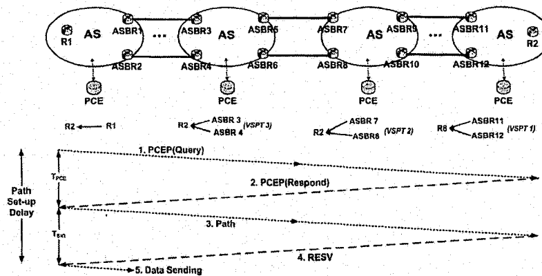
Figure 5.3: BRPC inter-domain path computation technique proposed by IETF
