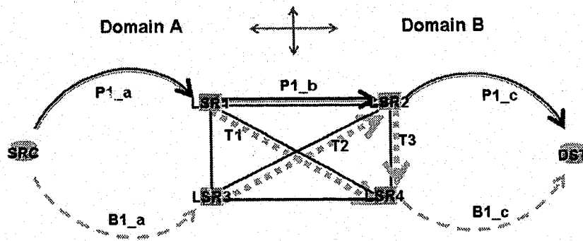
Figure 2.9: Inter-domain MPLS Protection [Huang04]
