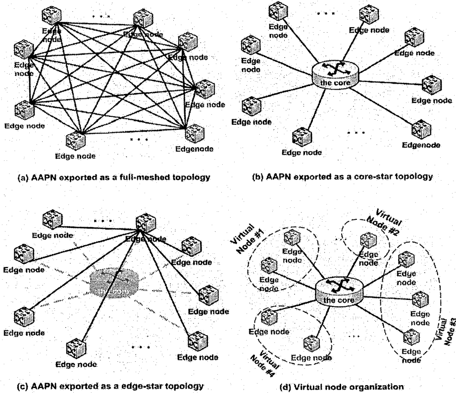
Figure 3.3: Exported Topologies of Agile All-Photonic Network
