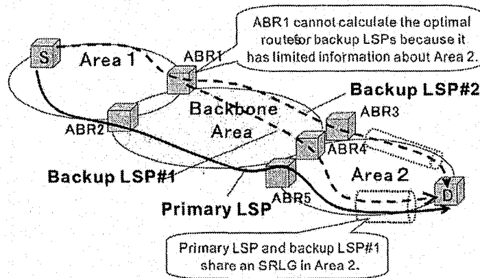
Figure 2.8: Inter-area SRLG-disjoint and multi-segment protection Scheme [Miyamura03]
