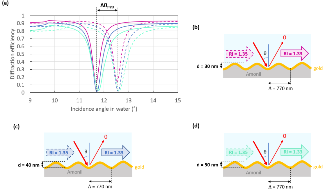
Figure 2.24: (a) Shift in the resonance angle due to a change of sensing medium with different RI (solid curve for initial water and dashed curve for a mix of water and glycerol with a RI of 1.35) for a (b) 30 nm (pink curves), (c) 40 nm (dark blue curves) and (d) 50 nm (bright blue curves) depth grating.
