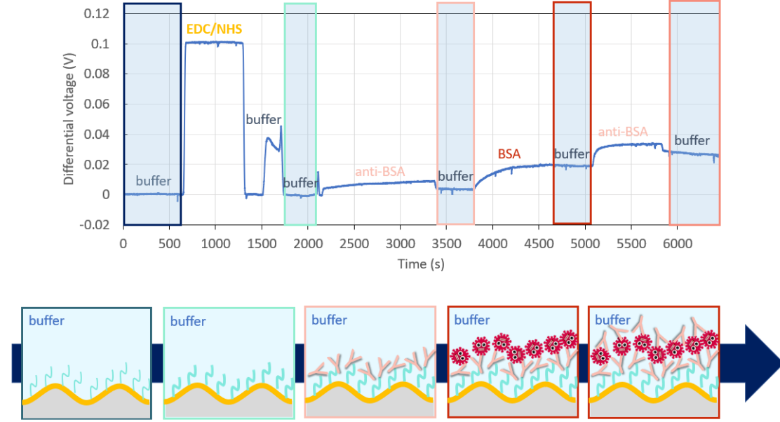
Figure 7.4: Complete cycle for the sandwich detection of BSA ( 40 \mu\text{g/mL} ) by anti-BSA ( 40 \mu\text{g/mL} ) immobilized on a gold-coated sinusoidal grating of period 770 nm and depth 228 nm. The grating was interrogated by a laser diode emitting at the free-space wavelength of \lambda_0 = 850 nm. The vertical axis plots the differential voltage measured from two amplified photodiodes capturing the 0^{\text{th}} and the -1^{\text{st}} diffracted orders. The sketches given at the bottom are not to scale.
