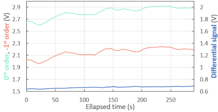
Figure 4.9: Time traces of the 0^{th} (green) and -1^{st} (orange curve) orders and the differential output signal (dark blue curve) obtained during injection of the solution s_1 with artificial noise affecting the system. The colours of the traces were modified. This Figure is adapted from [149]. Adapted with permission from https://doi.org/10.3390/s23031188 . Copyright © 2023 by the authors. Licensee MDPI, Basel, Switzerland. The Authors, licensed under a Creative Commons Attribution (CC BY) license.
