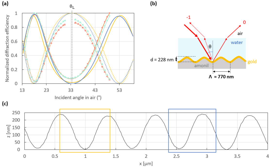
Figure 3.18: (a) Theoretical (dark blue and yellow curves) and experimental (bright blue and orange curves) normalized switch patterns resulting from the interaction of a p-polarized beam at a free-space wavelength \lambda_0=850 nm with the structure sketched in (b). The dotted lines represent the -1^{st} order, while the solid lines represent the 0^{th} order. The theoretical normalized switch patterns were simulated considering the period highlighted with boxes of the same colour in (c) which gives the AFM profile of the 121 nm thick gold-coated grating used to obtain the normalized experimental switch patterns in (a). The experimental switch patterns were normalized by dividing the respective measurements (photodiode output voltage of the transimpedance circuit) by the maximum value. The theoretical switch patterns were normalized in the same way as the experimental ones (using the computed diffracted waves) to be directly compared.
