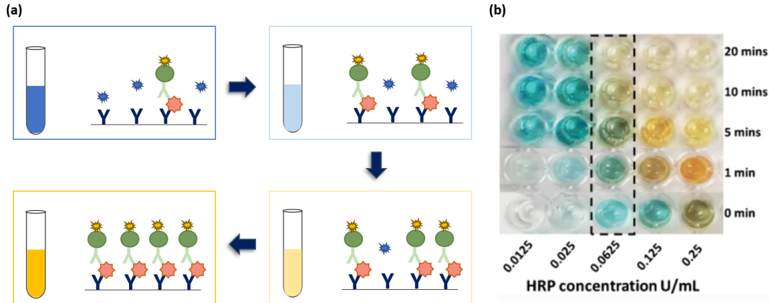
Figure 1.2: (a) Four sketches showing the correlation between the concentration of targeted analytes immobilized on the well walls and the change of coloration of the solution in the microwells. These sketches are not to scale. (b) Picture of an ELISA assay extracted from [22] showing the change of coloration observed at different reaction times depending on the concentration of the targeted analytes immobilized on the well walls. Reproduced with permission from Springer Nature, https://doi.org/10.1007/s00216-021-03359-8 . Copyright © 2021, Springer-Verlag GmbH Germany, part of Springer Nature.
