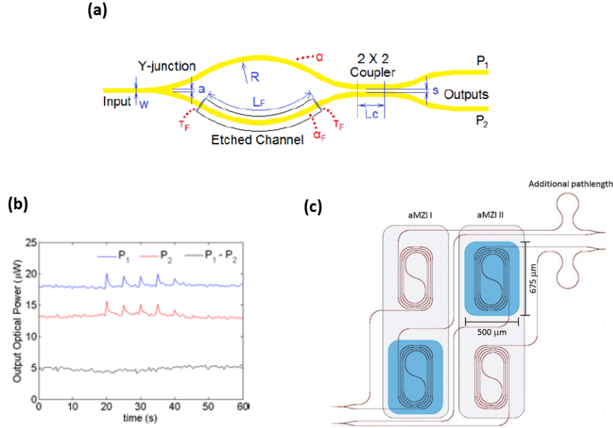
Figure 2.20: (a) Sketch of a dual output MZI. The dimensions labeled on the parts are: w = 5 \mu m , R = 5.5 mm , a = 2 \mu m , L_c = 100.25 \mu m , s = 3 \mu m , and L_F = 1.1985 mm . (b) Time traces of every single output ( P_1 , P_2 ) and their differential measurement ( P_1 - P_2 ) with the introduction of artificial noise. These figures are extracted from the article [110]. Reprinted with permission from IEEE, https://doi.org/10.1109/JLT.2016.2543138 . Copyright © 2016, IEEE. (c) Sketch of two asymmetric MZI with an additional path length in each reference arm on the left of the sketch. The blue areas show the sensing arms over which the fluids circulate. This sketch is extracted from [128]. Reprinted with permission from Elsevier, https://doi.org/10.1016/j.snb.2019.126758 . Copyright © 2019 Elsevier B.V.
