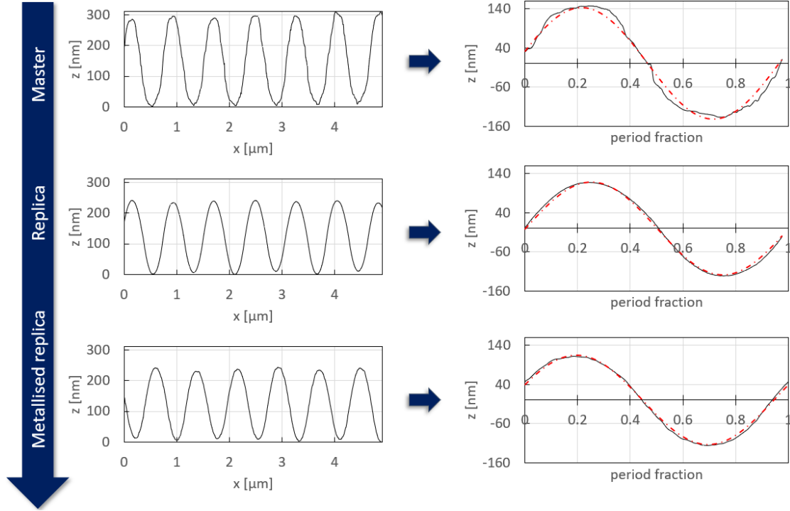
Figure 3.12: Evolution of the grating profile from the initial master to the metallised grating replica as measured by AFM scans (left panels). The right panels show a period extracted from each AFM profile with a perfect sinusoidal fit (red dashed-dotted curve)
