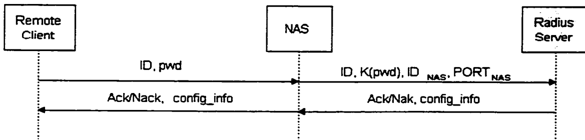
Figure 3B: RADIUS-PAP message exchanges.
