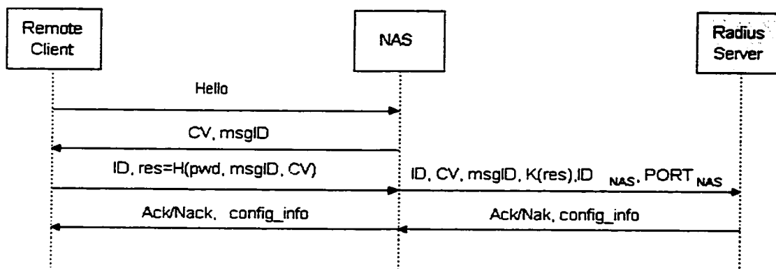
Figure 3C: RADIUS-CHAP message exchanges.
