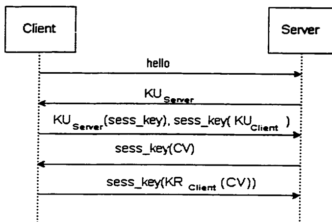
Figure 3E: SSH message exchanges.
