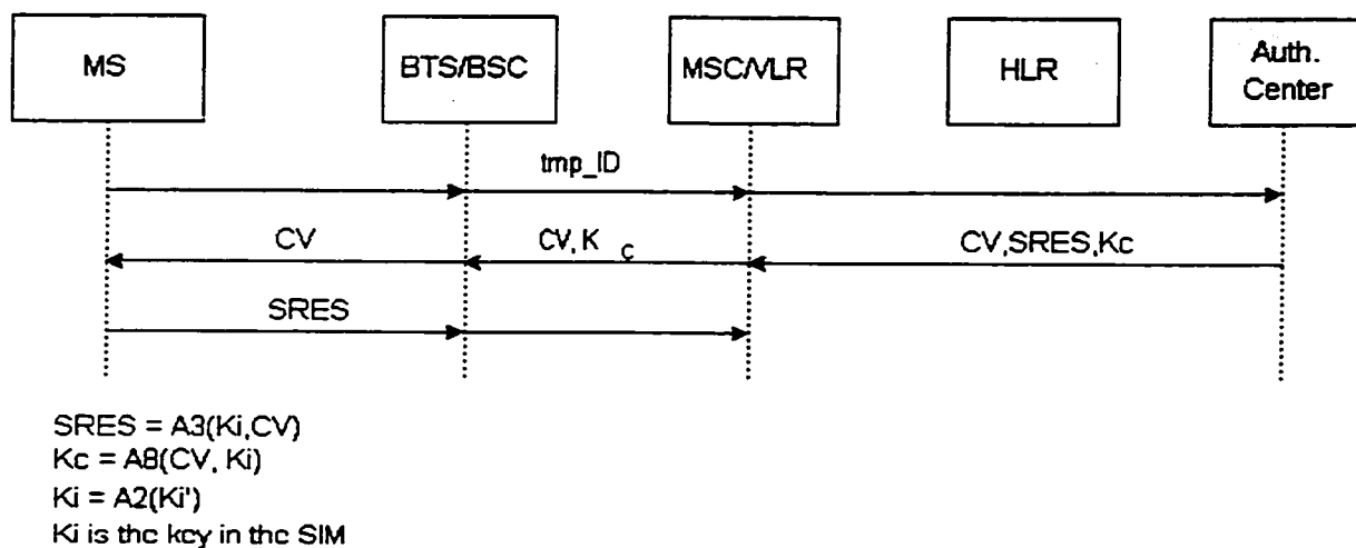
Figure 4C: authentication message exchange in GSM.
