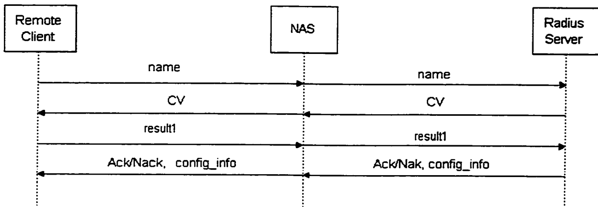
Figure 3D: RADIUS-OTP message exchanges.
