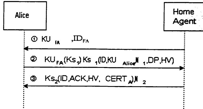
Figure 7F: Home domain message exchanges - Ack.
