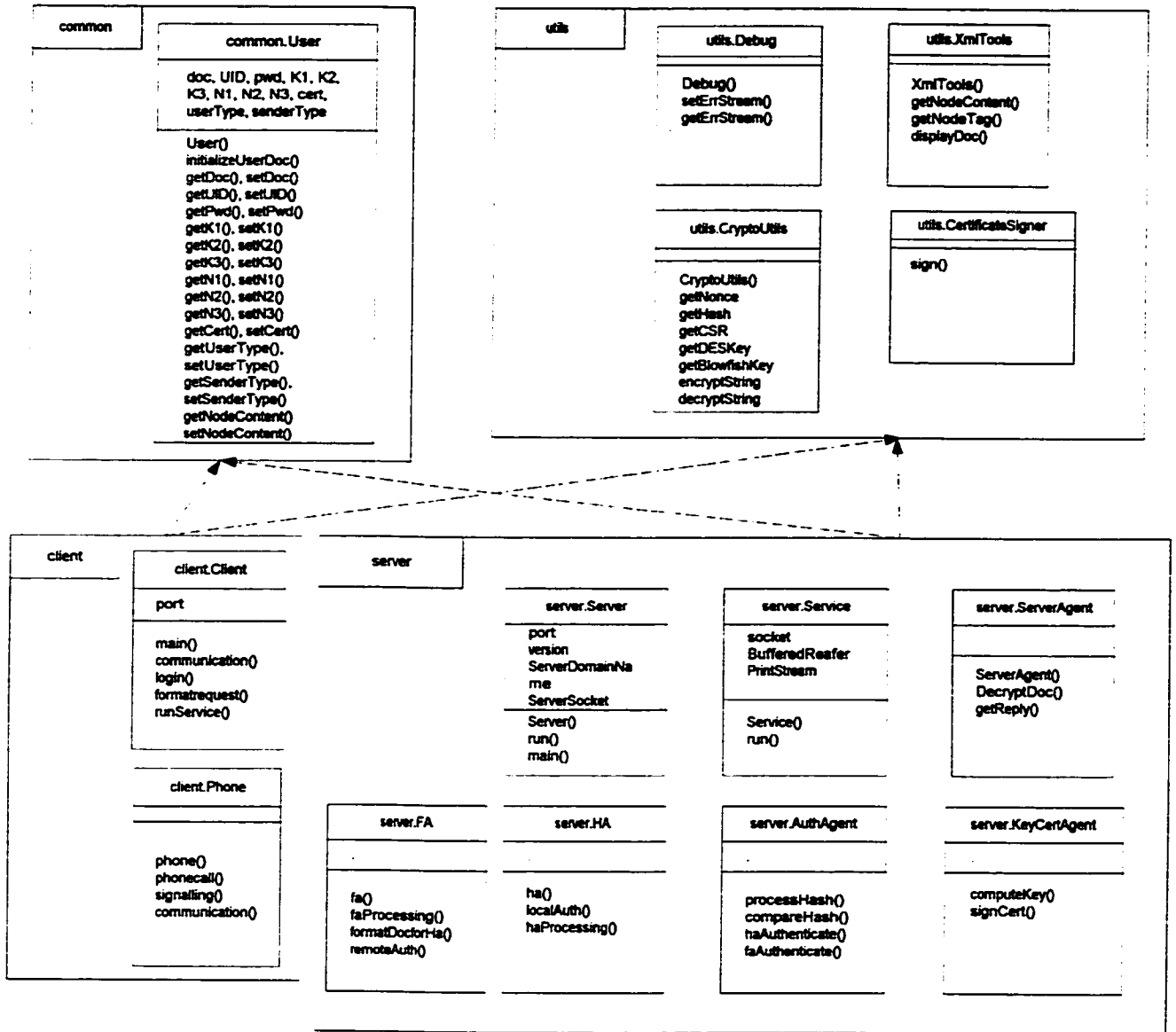
Figure 8C: Class diagram with package dependence.
