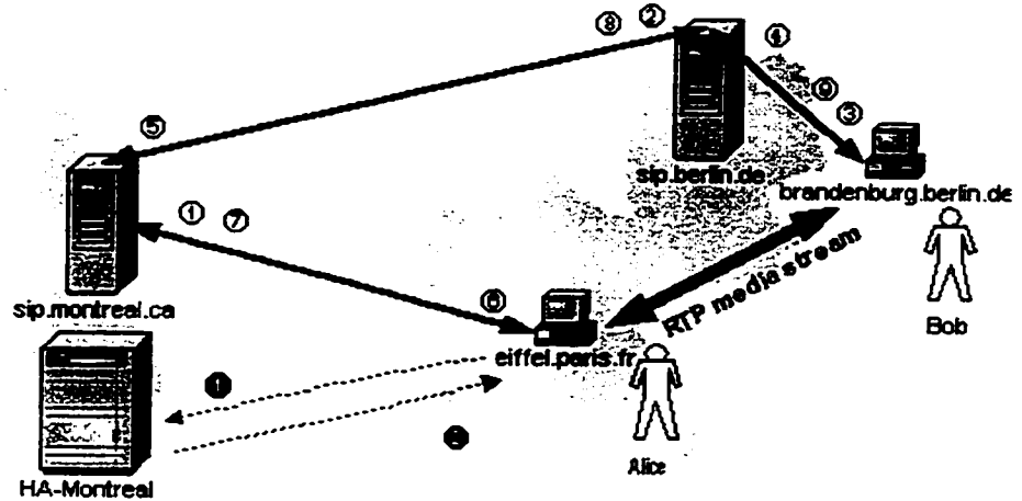
Figure 7K: Phone call protocol overview.
