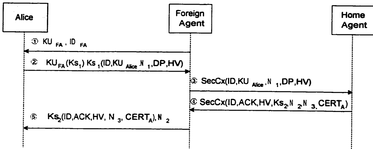
Figure 7C: Authentication message exchanges - Ack.
