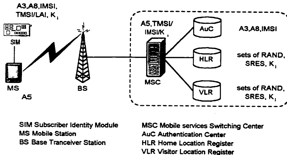
Figure 4B – Security architecture in GSM
