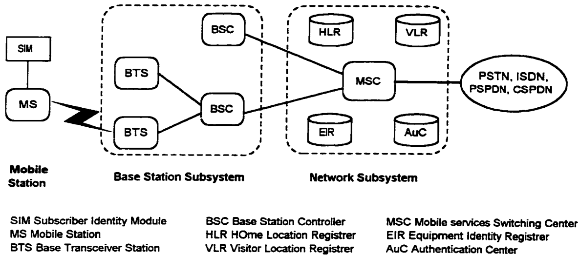
Figure 4A - Schematic presentation of the GSM network
