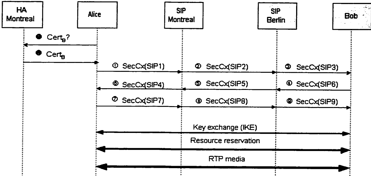
Figure 7L: Phone call message exchanges.
