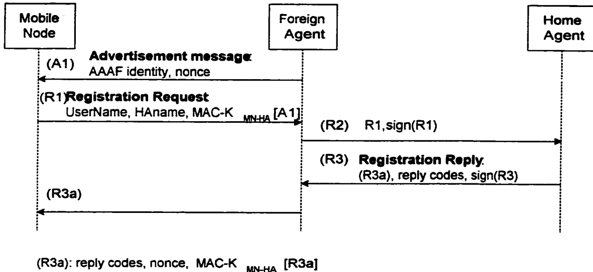
Figure 5D: session-based mobility protocol.
