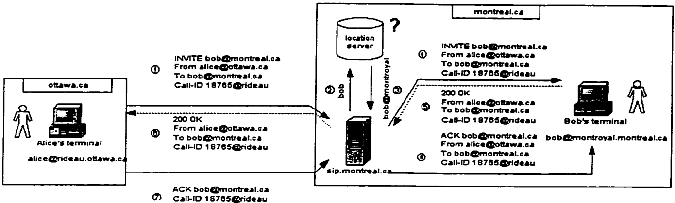
Figure 4E: SIP message exchanges.
