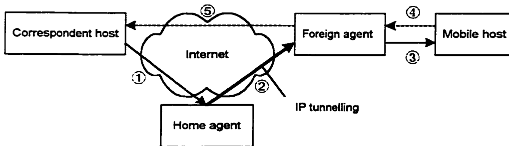
Figure 5A: Mobile IP architecture.
