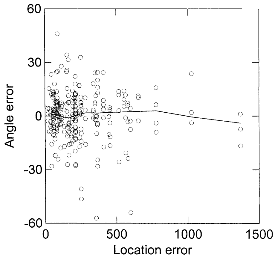
Figure 3.5. The relationship between angle error ( ^{\circ} ) and location error (m) for test data A ( n = 276 ). Locations were calculated using the MLE.
