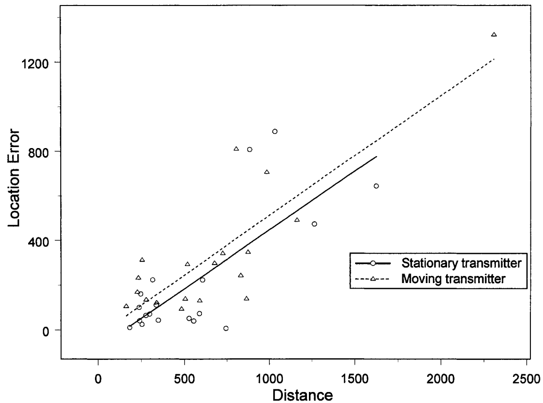
Figure 3.14. The effect of distance (m) between the transmitter and receiver on location error (m) for both moving and stationary transmitters. Locations were calculated using the geometric mean of bearing intersections ( n = 19 ).
