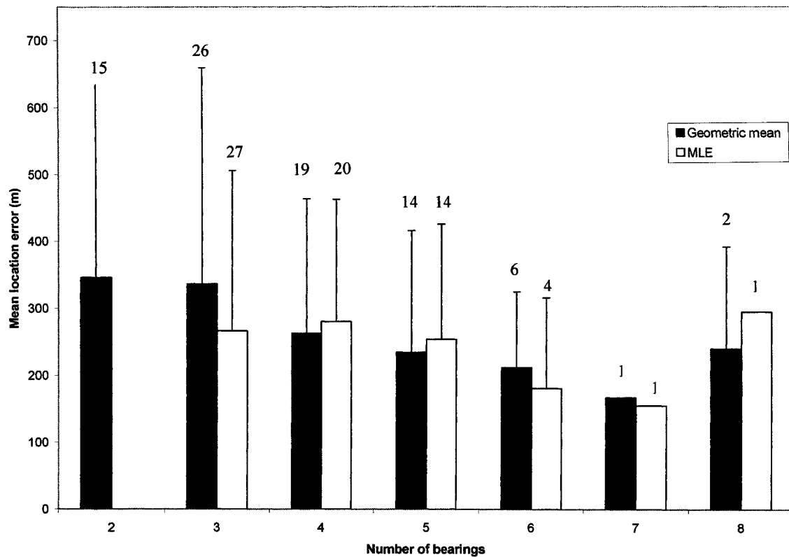
Figure 3.8. Mean location error (+ SD) as a function of the number of bearings used to make up the point location. Locations were derived from the geometric mean of bearing intersections or the maximum likelihood estimate (MLE) for test data A. Numbers above the error bars indicate sample size.
