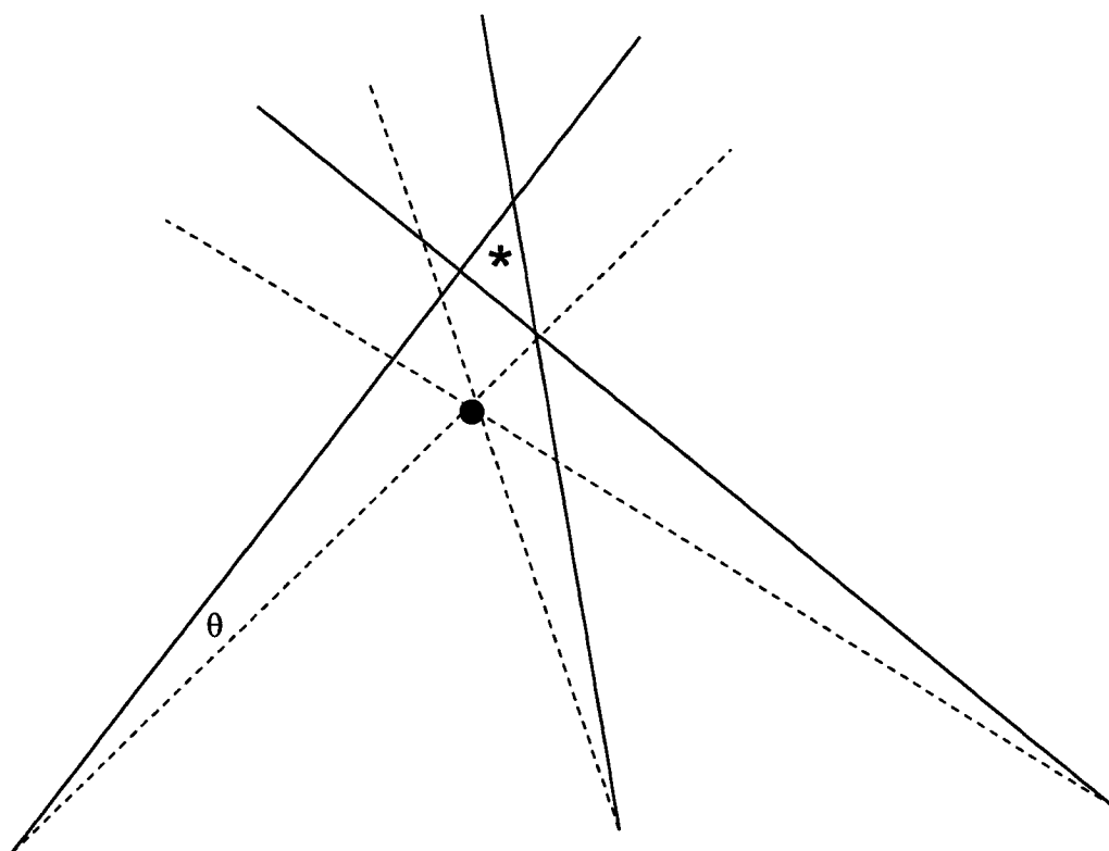
Figure 3.1. Triangulation error for a stationary transmitter. The dot represents the true location of the transmitter. The dashed lines are the actual bearings while the solid lines are the estimated bearings. The star represents the estimated location. The distance between the star and the dot is the triangulation, or location error. \theta is the angle error.
