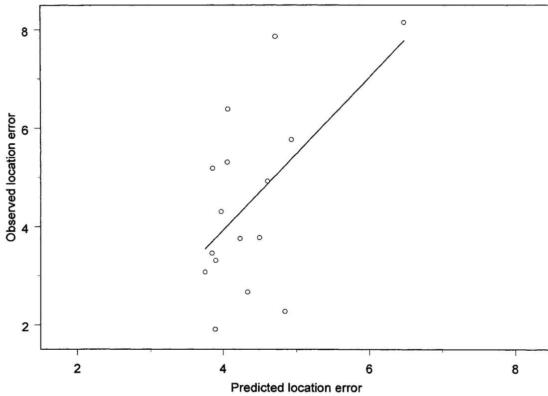
Figure 3.10. Predicted and observed MLE location error (m) (cube root transformed) for test data B ( n = 16 ). Predicted error is derived from the regression of location error and distance between transmitter and receiver for test data A.
