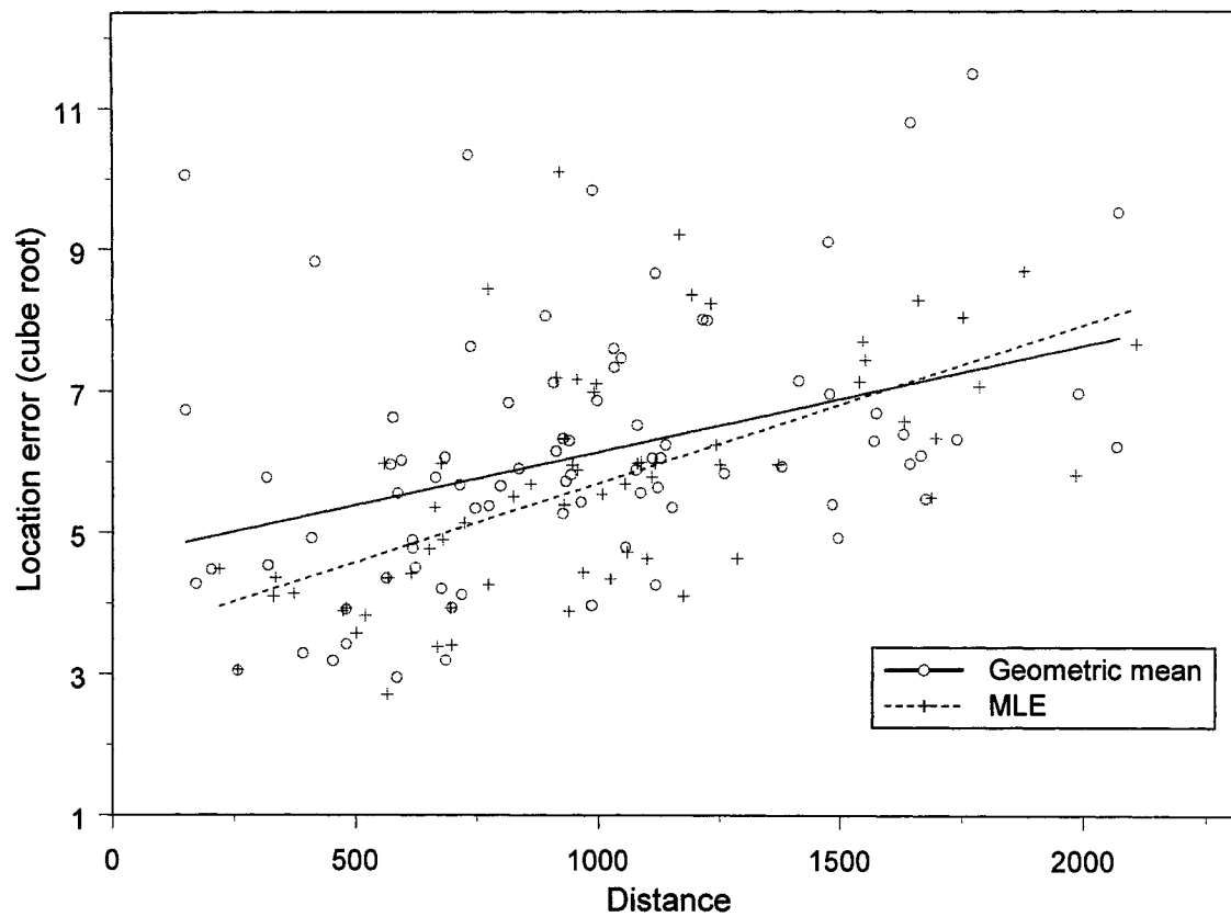
Figure 3.7. The cube root of location error (m) vs. the distance between the receiver and estimated transmitter location (m) for points derived from the geometric mean of bearing intersections ( n = 83 ) and the maximum likelihood estimate (MLE, n = 66 ) for test data A.
