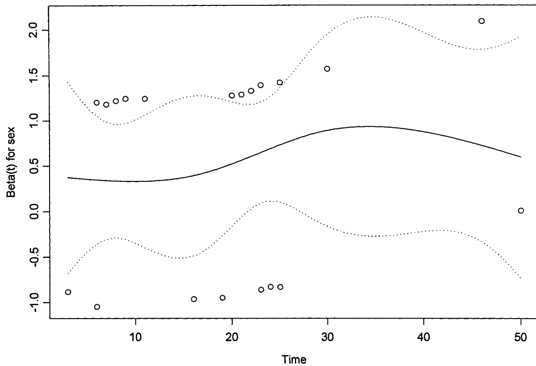
Figure 4.5. Scaled Schoenfeld residuals for the Cox proportional hazards model of fisher survival (over 2 years), with sex as a covariate. The solid line is a smoothing spline and the dotted lines are \pm 2 standard error. Departures from a horizontal line are indicative of non-proportional hazards.
