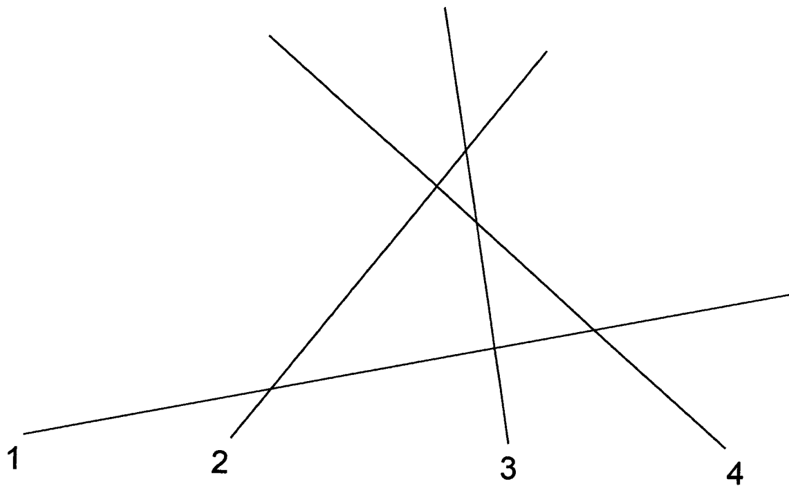
Figure 3.2. Demonstration of a potentially erroneous bearing when assessing triangulation error. The intersections of bearing 1 with bearings 2, 3 and 4 are far from the intersections of all other bearings. Thus, bearing 1 is omitted from the triangulation.
