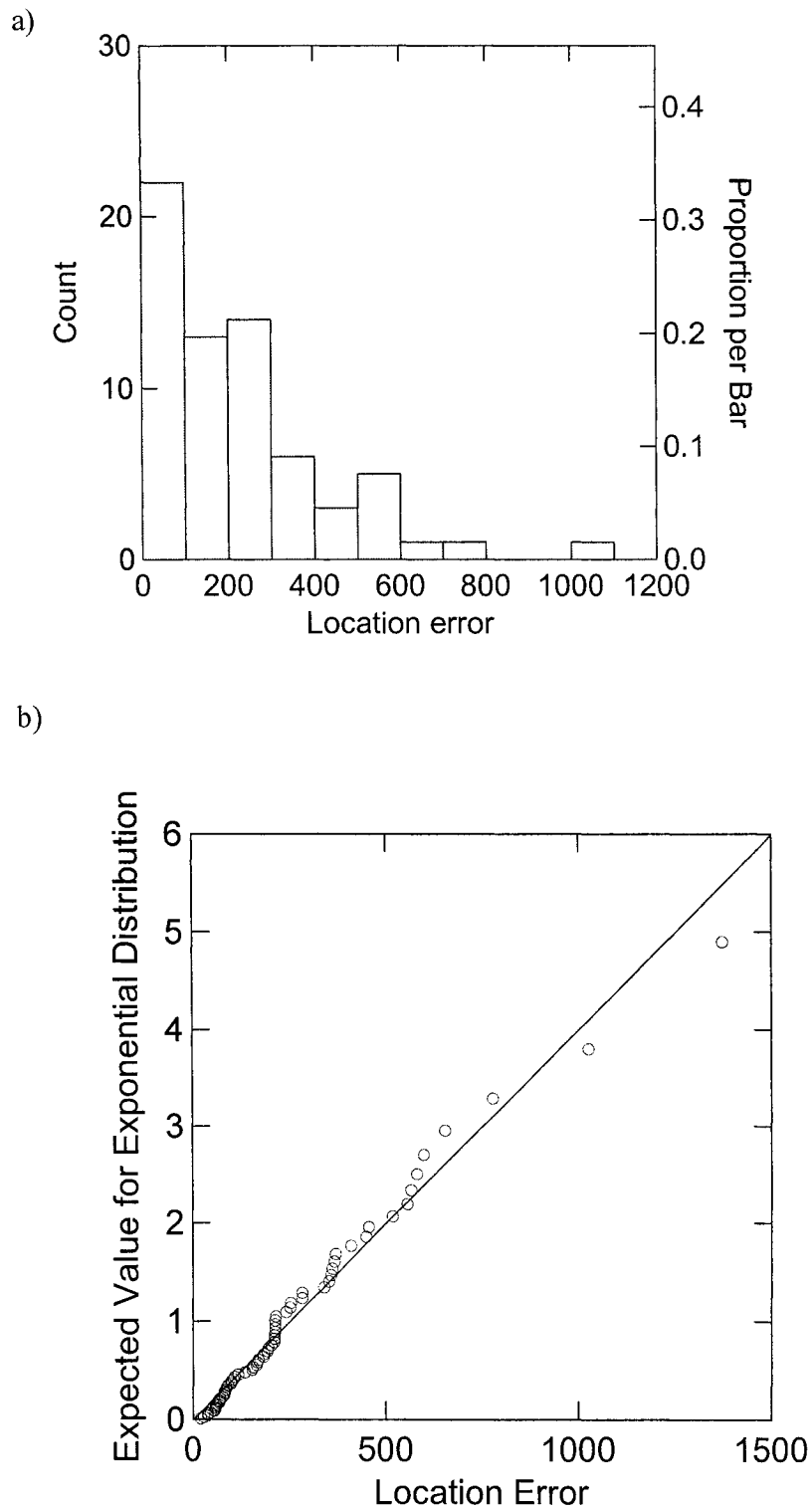
Figure 3.11. a) Distribution of location error (m). b) Probability plot of location error (m) vs. the expected value if the distribution is exponentially distributed.
