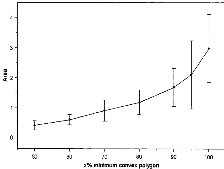
Figure 1.6. Mean ( \pm 1 SD) estimated area (km 2 ) of minimum convex polygon home ranges with 5 to 50% of the locations furthest from the arithmetic mean of x,y coordinates excluded. Home ranges are for a) male (n = 10) and b) female (n = 16) fishers in eastern Ontario between June 2003 and February 2004.
