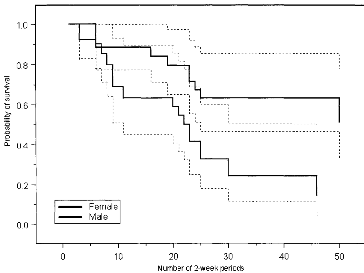
Figure 4.4. Two-year Kaplan-Meier survivorship and 95% confidence intervals (dotted lines) for male and female fishers from February 2003 until December 2004 (n = 59).
