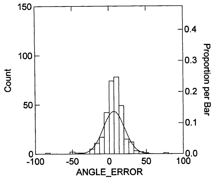
Figure 3.6. The distribution of angle error (°) for test data A with a normal curve superimposed (n = 315).
