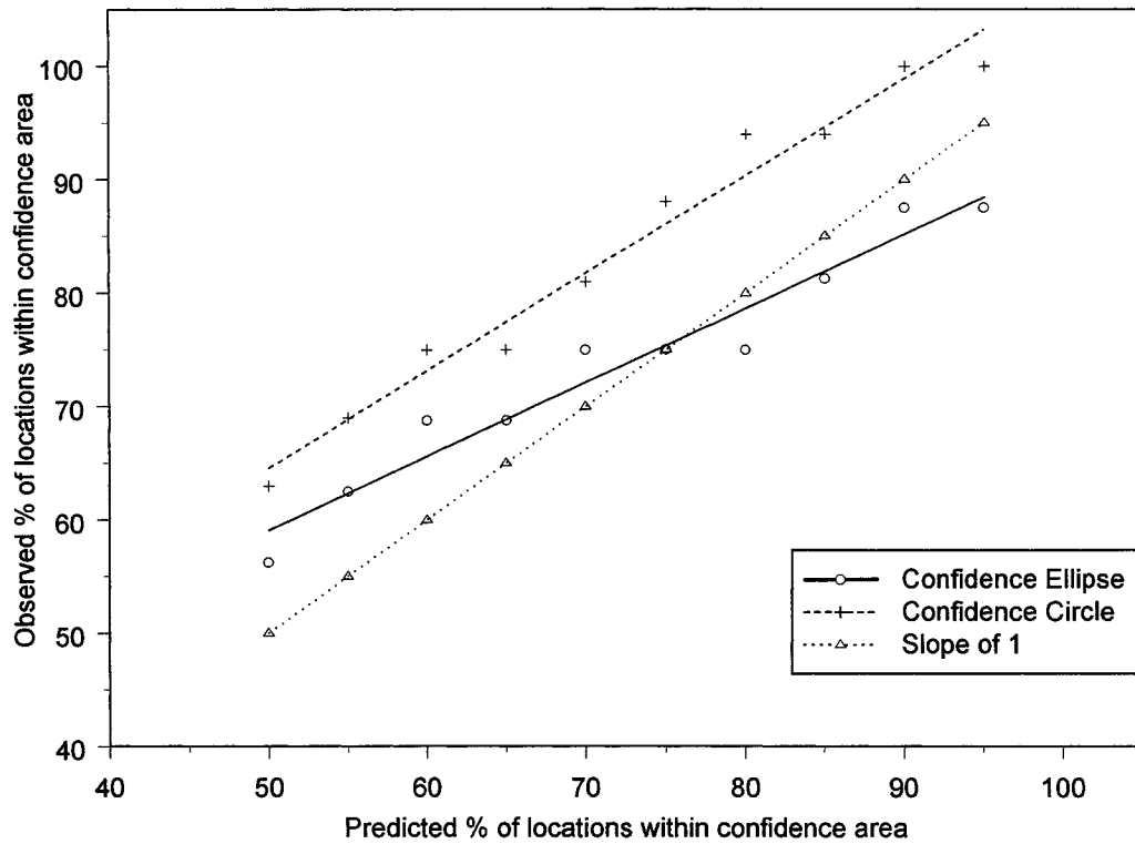
Figure 3.12. Observed percentage of test data B locations falling within x% confidence areas ( n = 16 ), including a line passing through the origin with a slope of 1 for comparison.
