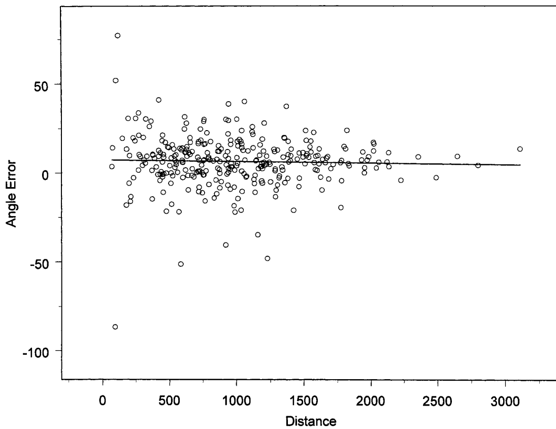
Figure 3.4. The relationship between angle error ( ^{\circ} ) and the distance between the receiver and the estimated transmitter location (m) for test data A ( n = 315 ).
