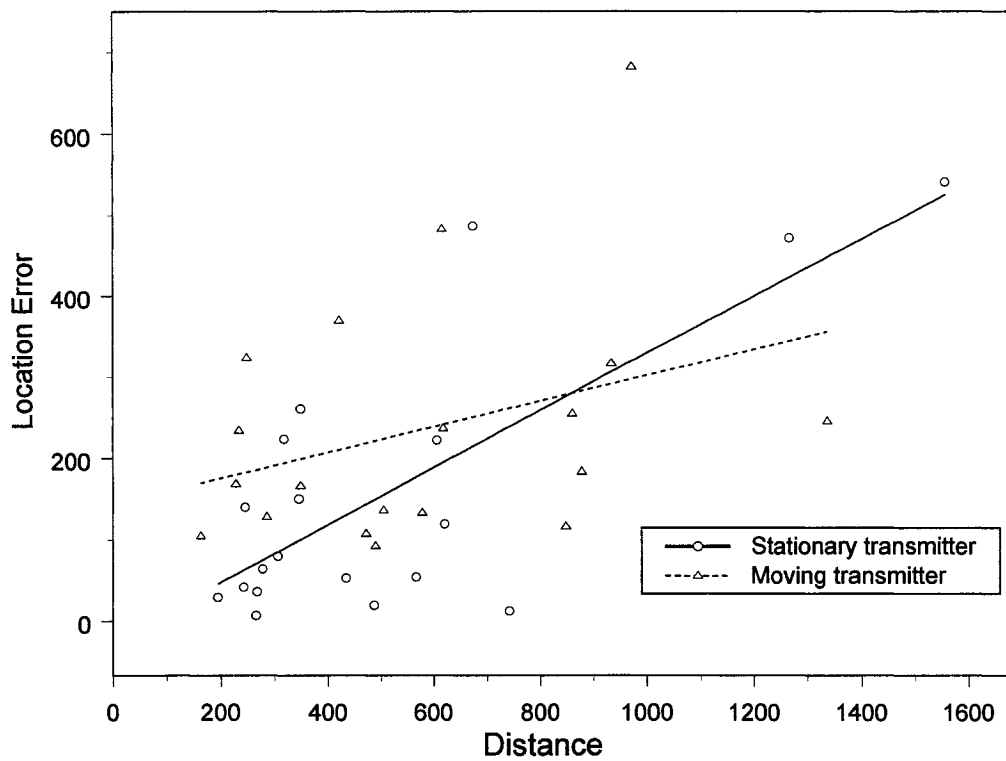
Figure 3.13. The effect of distance (m) between the transmitter and receiver on location error (m) for both moving and stationary transmitters. Locations were calculated using the maximum likelihood estimate ( n = 19 ).
