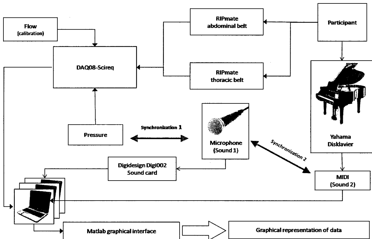
Figure 4.1: Experimental set-up illustrating the double synchronization method.
