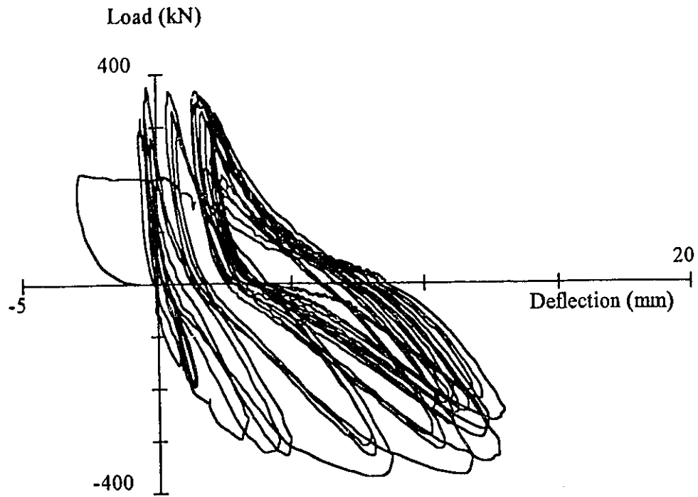
Figure 3.34 Load-West Top Vertical Deflection for Wall 7
