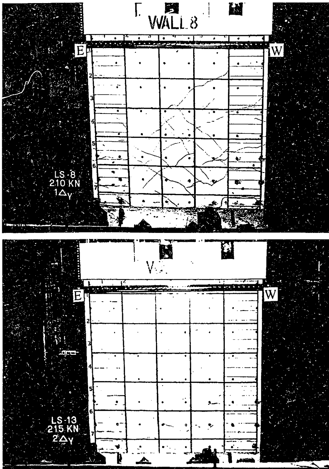
Figure 3.49 Wall 8 Crack Pattern, Cycle 1 (pulling) at 1\Delta_y (above) and Cycle 1 (pushing) at 2\Delta_y (below)
