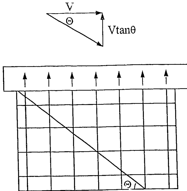
Figure 5.11 Vertical Component of Shear Load in Reinforcement
