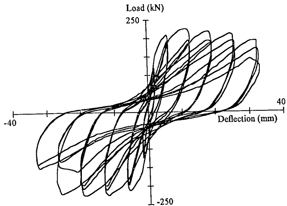
Figure 4.16 Hysteretic Load Top Horizontal Deflection for Wall 8 at the Center of the Top Beam
