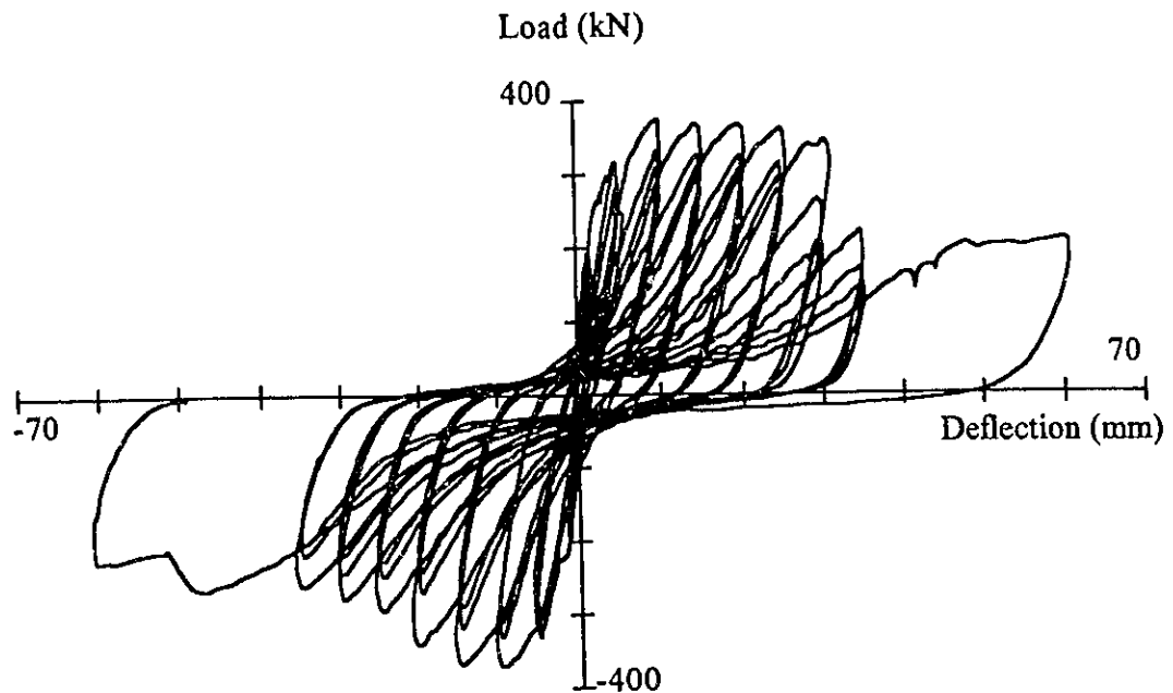
Figure 3.31 Load-West Top Horizontal Deflection for Wall 7 at the Level of Potentiometer
