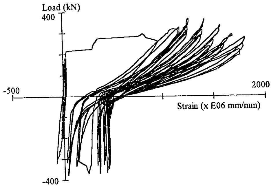
Figure 3.47 Load-Strain Relationship for Horizontal Bars, average of H741 and H742 Wall 7
