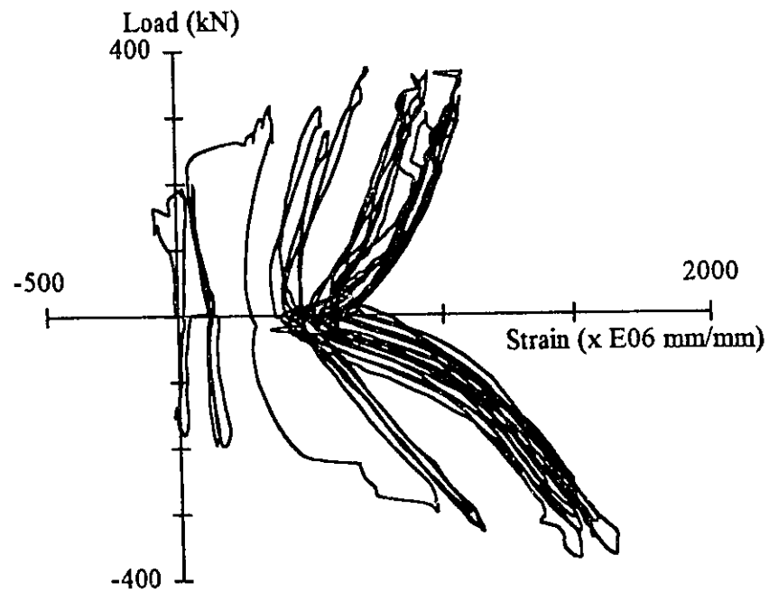
Figure 3.46 Load-Strain Relationship for Horizontal bar, H724, Wall 7
