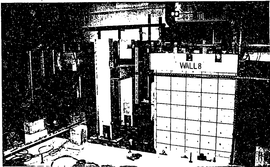
Figure 3.13 Overall View of the Test Set-Up
