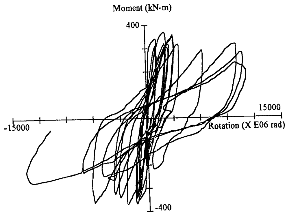
Figure 4.17 Hysteretic Moment Anchorage Slip Rotation for Wall 8
