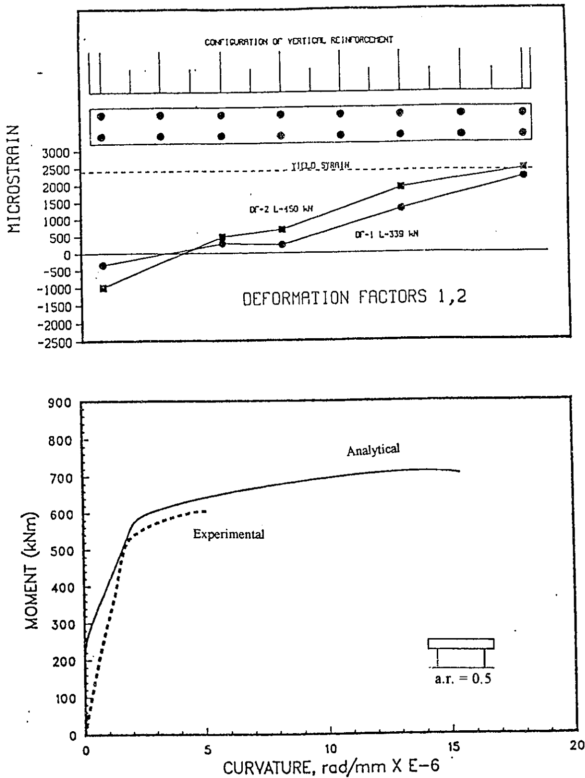
Figure 5.4 Strain Profiles in Flexural Reinforcement (above) and Moment Curvature Relationship for Wall 6 (adopted from Wasiewicz, 1988)
