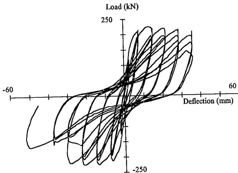
Figure 3.54 Load-West Top Horizontal Deflection for Wall 8 at the Level of Potentiometer
