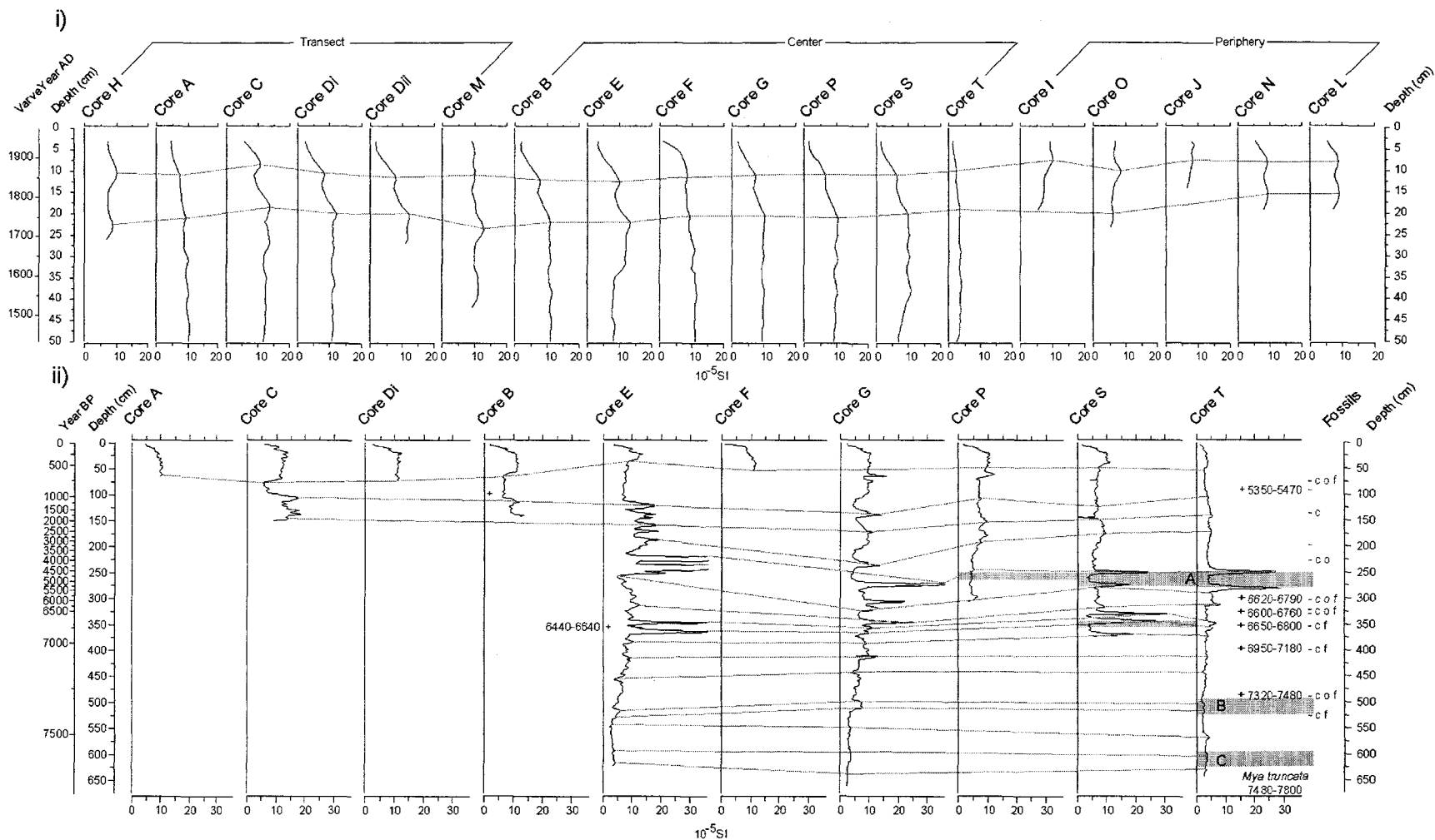
Fig 3.1: i) Magnetic susceptibility profiles of all cores, truncated at 50cm, and ii) "Wiggle-matched" magnetic susceptibility profiles (gray lines) of cores longer than 50cm. 2-sigma calibrated radiocarbon dates (+), subfossil presence at sampling sites (-), where c is chronomid head capsules, o is ostracode valves, and f is forams. Grey zones are A) a thick homogenous bed, B) a transition zone between deeper grey sediments and orange-tan sediments above, and C) a portion containing dark grey pebbles.
