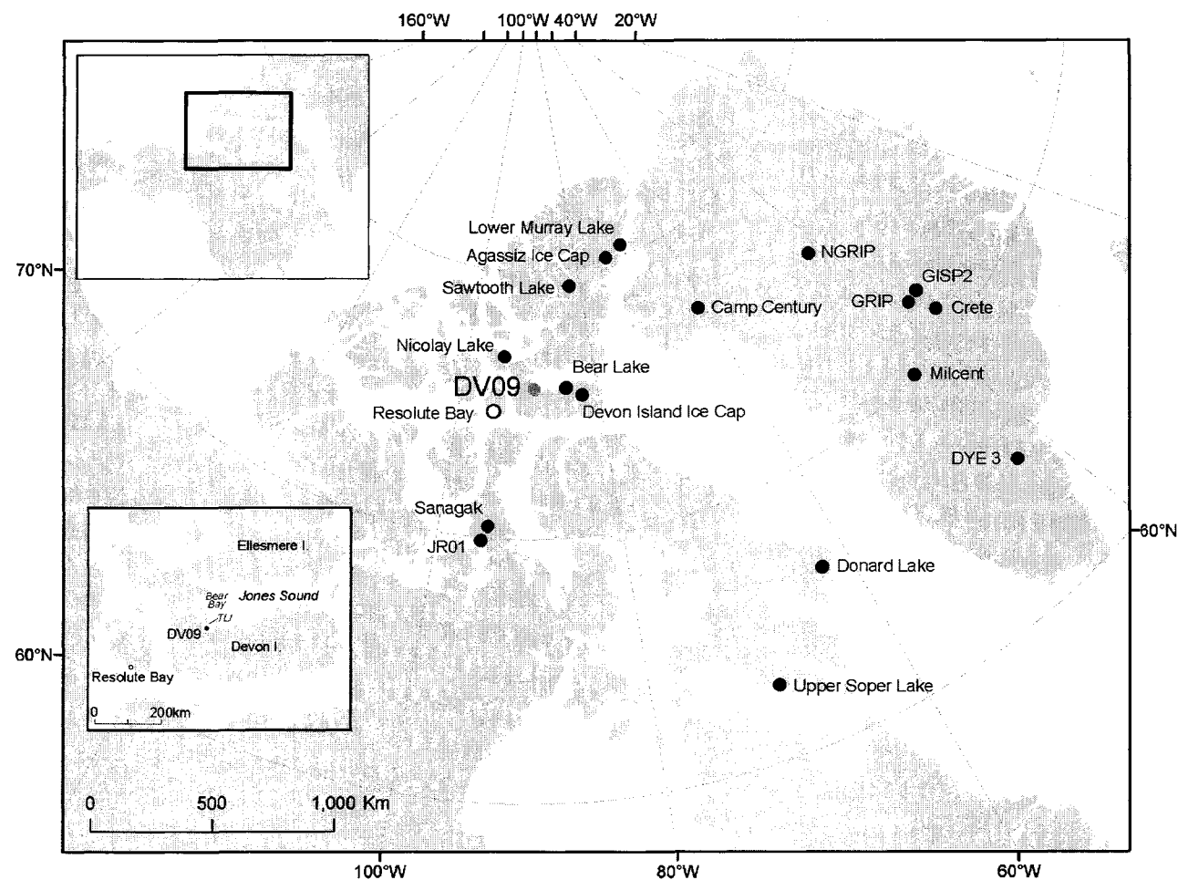
Fig 1.1: Arctic North America, grey dot shows the the study site, white dot shows the meteorological site, and black dots indicate other paleoclimate records discussed in the text. Inset Map: Devon Island region. TLI = Thomas Lee Inlet.
