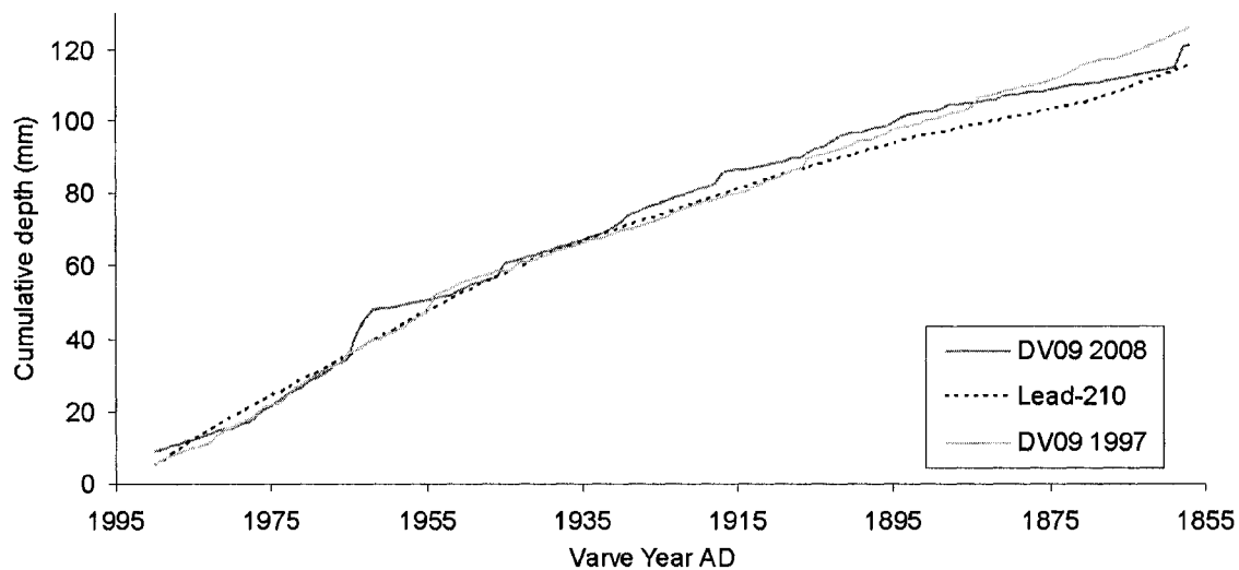
Fig 4.4: The varve record from this paper, and the lead-210 dates from a previously dated short core (Turner, 1995; Gajewski et al , 1997). Data was truncated to the CRS modeled dates (AD1990-1857).
