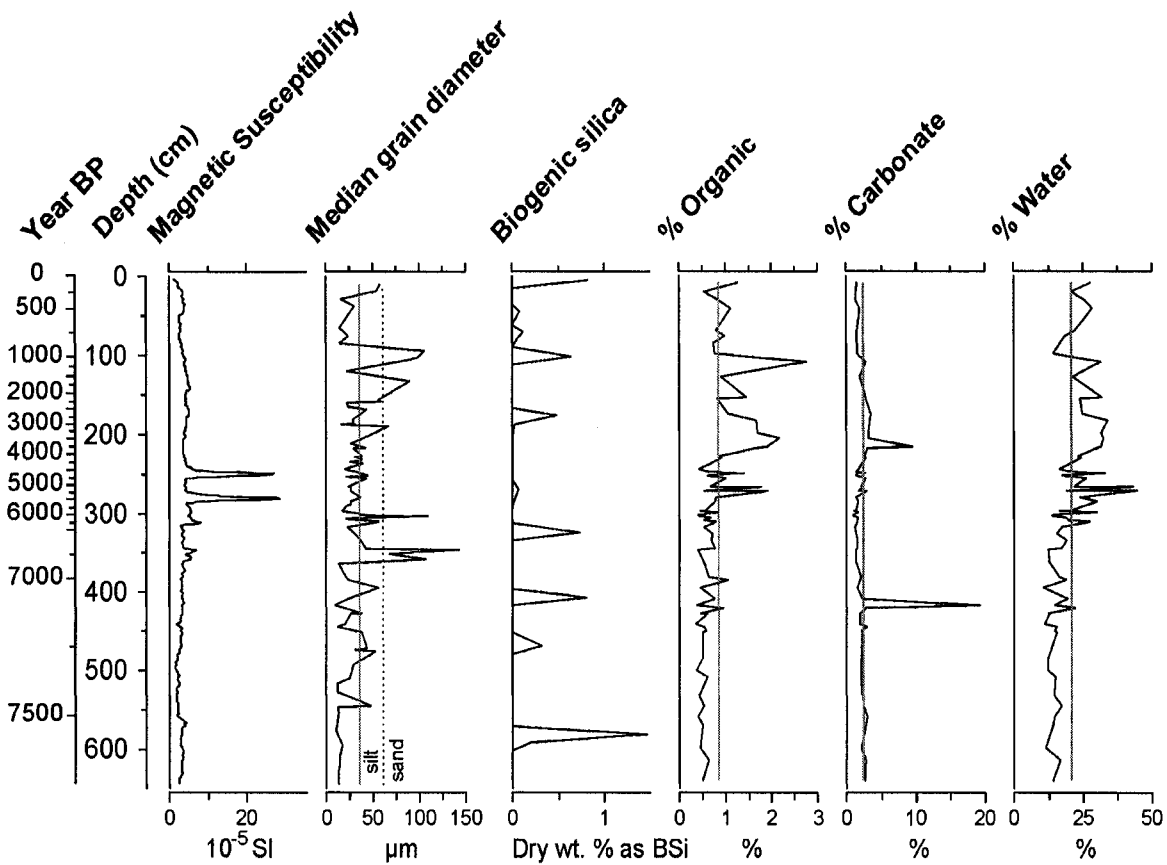
Fig 3.2: Core T sedimentologic measurements. The vertical grey line shows the respective series mean, equal to 35.11 \mu\text{m} for the median grain size diameter, 0.844% for organic matter, 2.54% for carbonate content, and 20.88% for water content.
