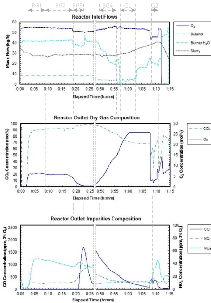
Figure 5.4 – Reactant flows and product gas compositions
