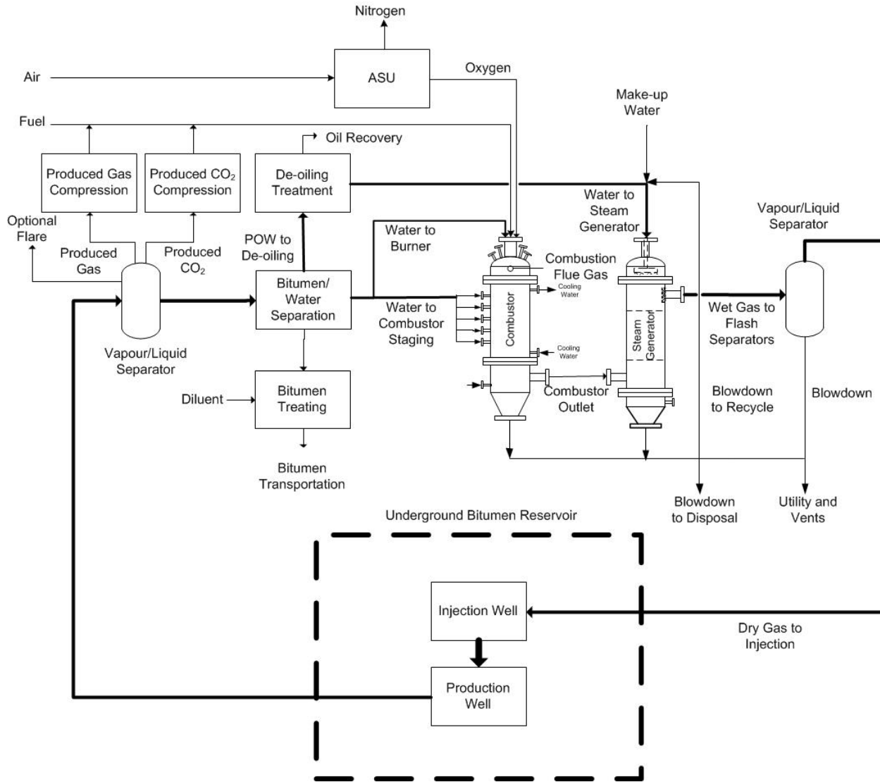
Figure 2.2 – Oxy-fired Direct Contact Steam Generation Block Flow Diagram
