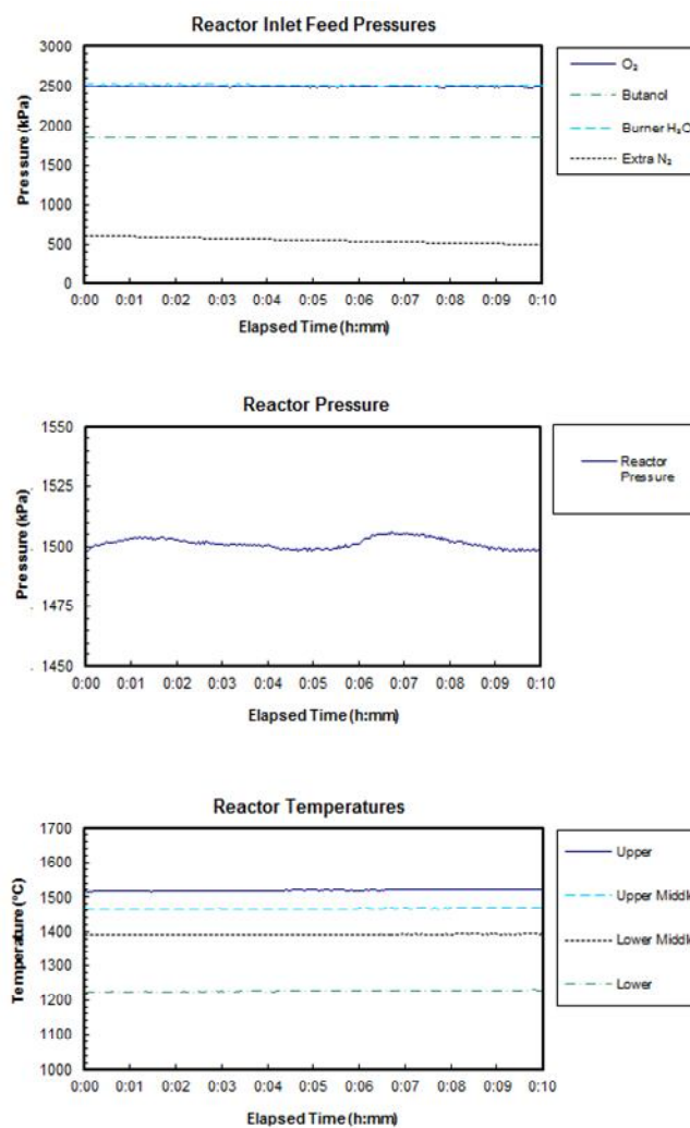
Figure 4.5 – Process pressures and temperatures for the test run that contained test period B1
