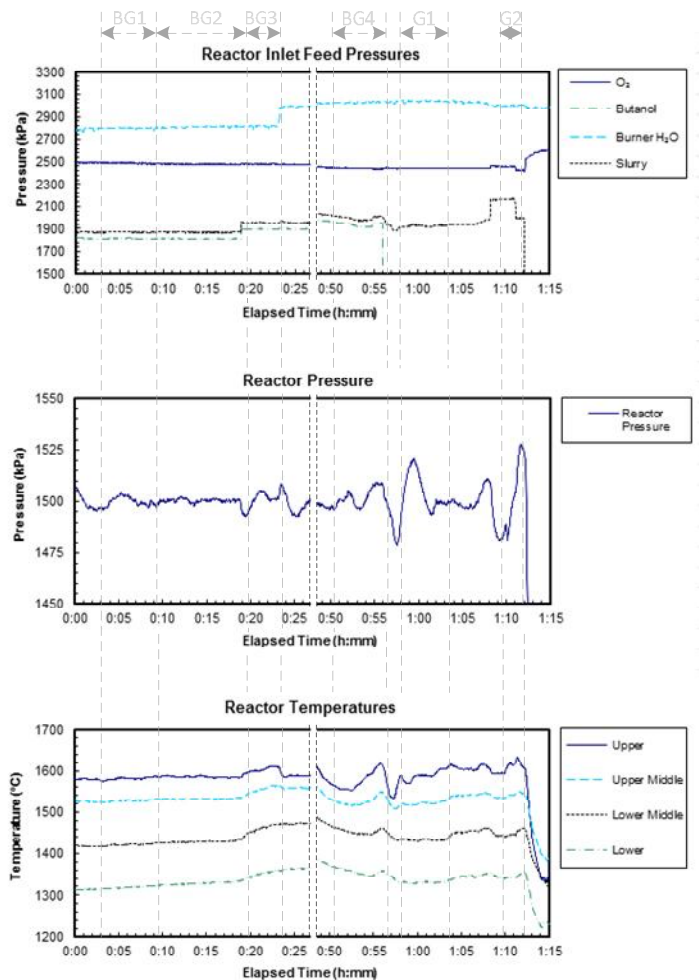
Figure 5.5 – Process pressures and temperatures
