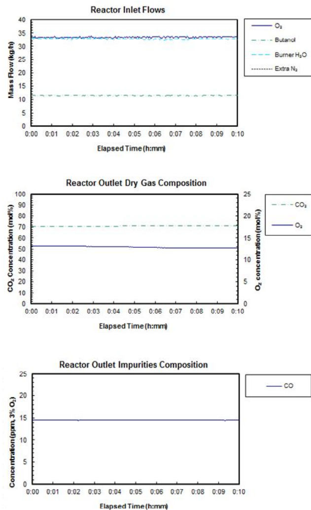
Figure 4.4 – Reactant flows and product gas compositions for the test run that contained test period B1
