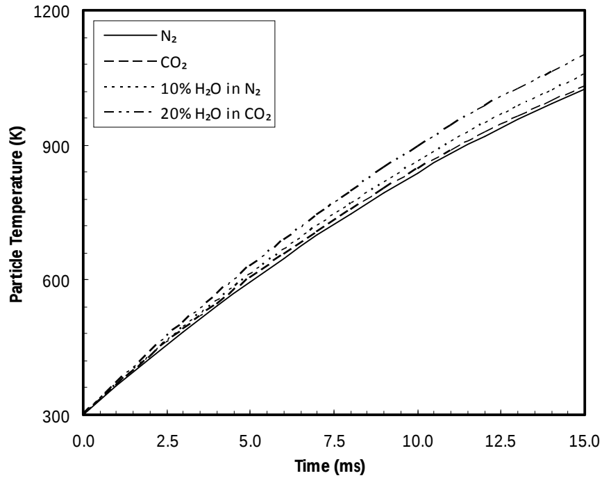
Figure 3.2 – Calculated particle temperature of a spherical 100 \mu\text{m} coal particle in selected gas environments at 1227 ^\circ\text{C} , with radiative boundary at 1000 ^\circ\text{C} and a Nusselt number of 2.0. Gas thermal conductivities are those indicated in Figure 3.3 , with gas mixture conductivity estimated according to simple molar mixing ratios, adapted from [17]
