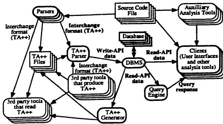
FIGURE 2.7 Architecture of the Program Comprehension Tool
