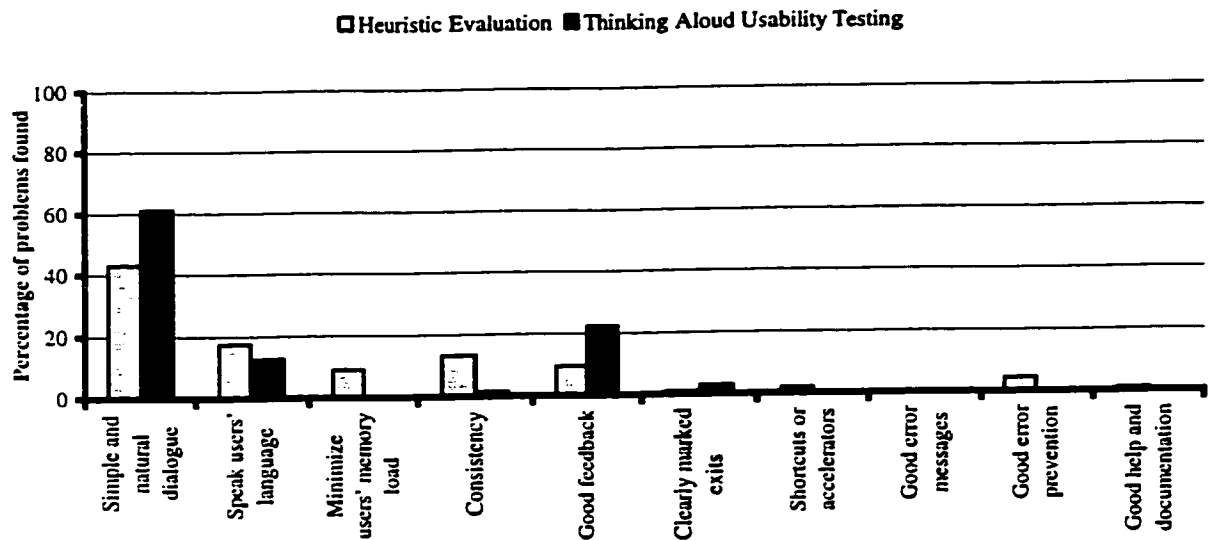
FIGURE 4.1 Problems according to the usability guidelines
