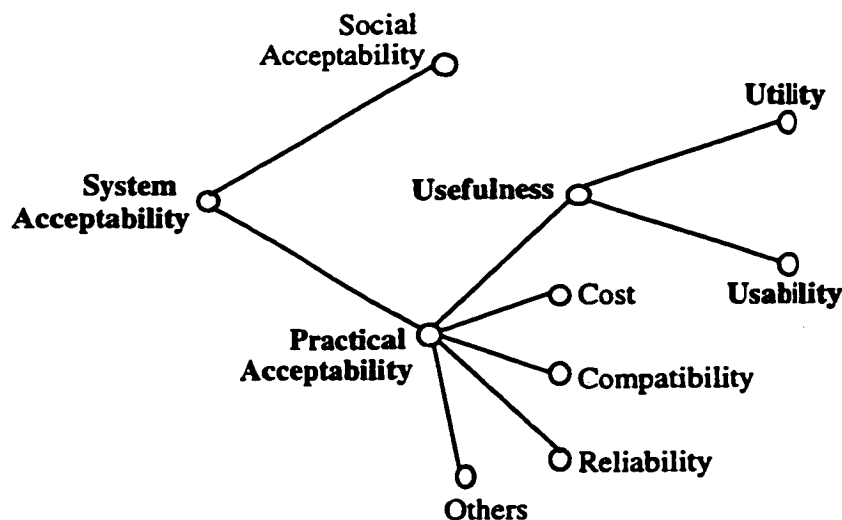
FIGURE 2.3 System acceptability and usability
