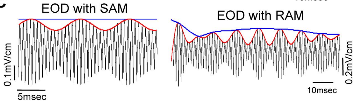
Figure 1. Electric organ discharge (EOD) from weakly electric fish in different situations. (A) Experimental recordings of two isolated individual fish. (B) An example compound EOD recording from two fish in close proximity. The interference of electric fields generated by each fish evokes a time-varying beating amplitude modulation (AM) which is a first order envelope E1 (red trace), as well as a second order envelope E2 (here a flat line, blue trace). (C) The EOD signal with a sinusoidal amplitude modulation (SAM, red trace) or a narrowband random amplitude modulation (RAM, red trace) are common ways to experimentally mimic or computationally simulate electrosensory signals arising from social interactions. doi:10.1371/journal.pcbi.1002564.g001
