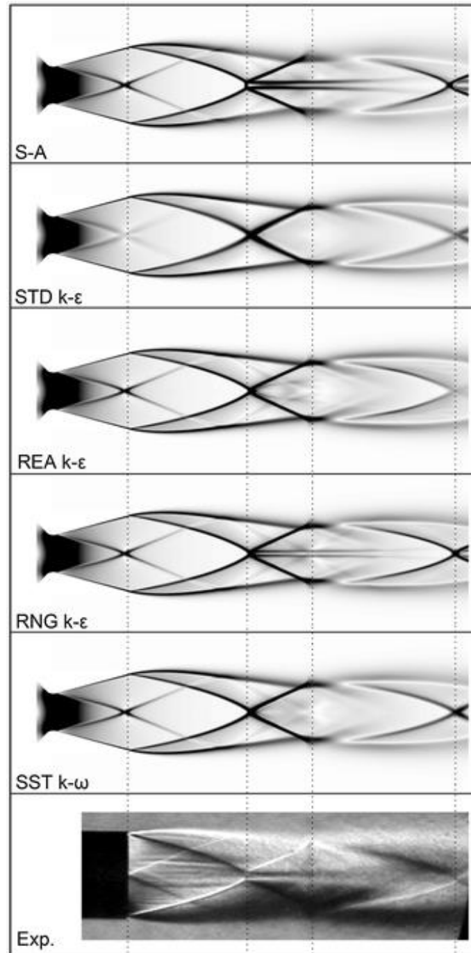
Figure 2.18: Gas flow pattern at the nozzle exit obtained using different turbulence models in CFD simulations. An experimental Schlieren image is provided for comparison purposes(Ref 27). (Reproduced with permission of Springer Nature)
