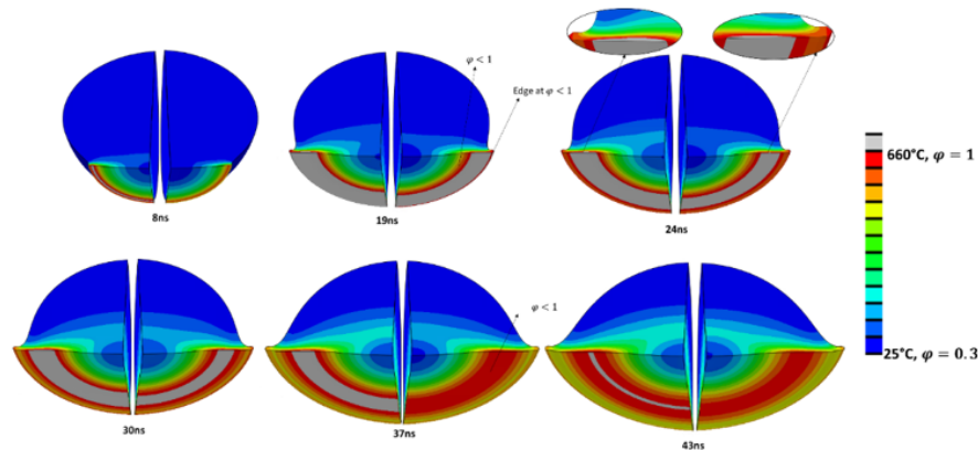
Figure 7: Numerical temporal evolution of particle temperature (left) and particle pressure-dependent melting temperature factor \phi (right) are provided at the interface of LPIT powder set 3 impact. Inserts show the effect of pressure through particle thickness.
