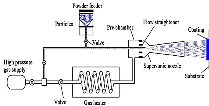
Figure 2.2: High pressure CGDS system layout with powder injection occurring upstream in the stagnating gas of the converging nozzle section (Ref 89). (Reproduced with permission of Elsevier)
