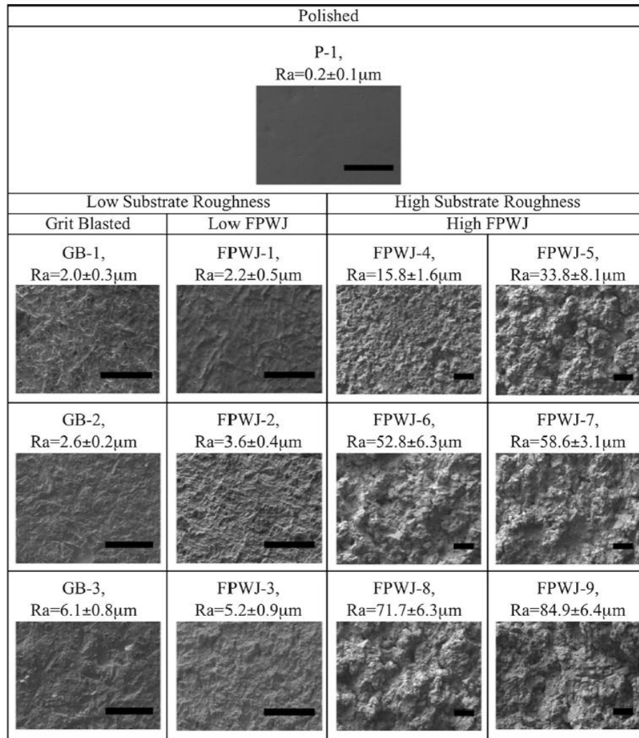
Fig. 3 SEM images of substrates top surface topography and resulting roughness (Scale = 200 \mu m )
