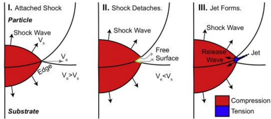
Figure 2.23: Jetting process related to pressure release in CGDS (Ref 172). (Reproduced with permission of Elsevier)
