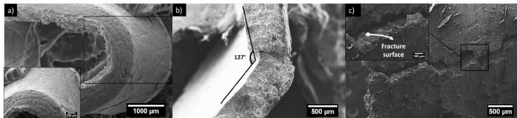
Fig. 12. SE SEM images of coatings during the bend-to-break process using feedstock powder set 2 with a) LPIT deposits showing no sign of cracking during the first phase of the bend-to-break test and b–c) HPIT deposits. A fracture surface from the HPIT coating is highlighted in image c).
