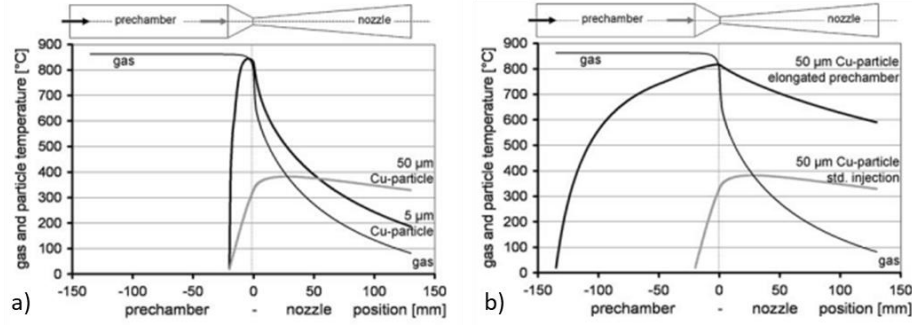
Figure 2.20: Particle in-flight temperature variation as it travels within a CGDS nozzle with an upstream injection (Ref 114). (Reproduced with permission of Springer Nature)
