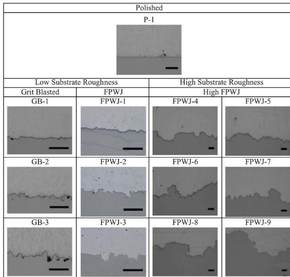
Fig. 4 Optical microscope cross-sectional images of the deposition interface for all produced surfaces (Scale = 100 \mu\text{m} )
