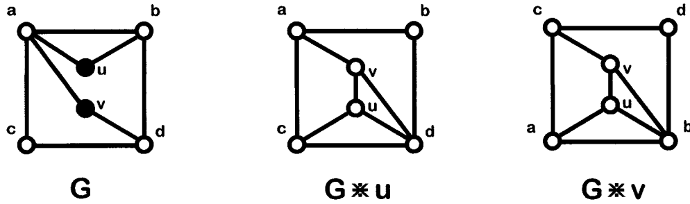
Figure 1.4: A graph with two vertex-switch pseudosimilar vertices
