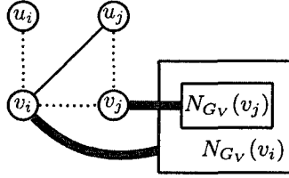
Figure 5.2: Across Edge Rule
