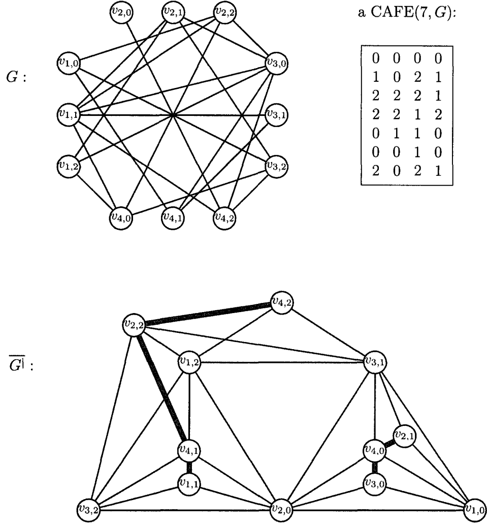
Figure 4.2: A graph G \in \mathcal{G}_{4,3} such that \text{CAFEN}(G) > \theta'(\overline{G}) .
