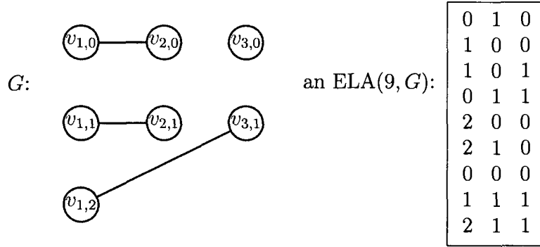
Figure 2.8: An error-encoding graph G \in \mathcal{G}_{(3,2,2)} and an \text{ELA}(9, G) .
