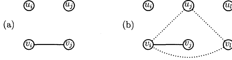
Figure 5.4: Theorem 5.2.11: Case 2: \{v_i, v_j\} \in E(G_{UV})
