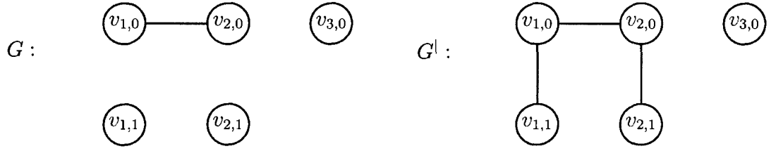
Figure 2.1: A forbidden edges graph G and the graph G^l
