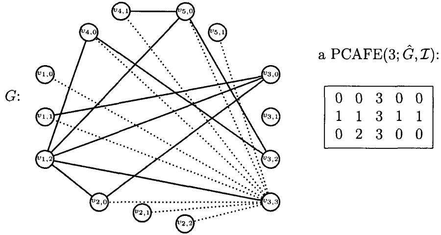
Figure 4.3: The forbidden edges graph G \in \mathcal{G}_{(3,3,4,2,2)} of the augmented mobile phone product line testing problem, with the dotted edges corresponding to \mathcal{I} , and a PCAFE(3; G, \mathcal{I} )
