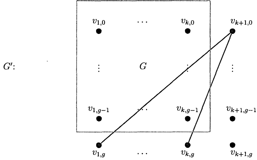
Figure 5.1: The graph G' of Proposition 5.1.5
