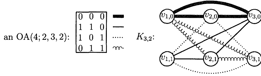
Figure 4.1: Equivalence of an \text{OA}(4; 2, 3, 2) and an edge-disjoint 3-ECC of K_{3,2} . The vertices of K_{3,2} are labeled as described in the proof of Proposition 4.1.1 and the edge-disjoint k -ECC of K_{3,2} is pictured by the different types of edges. Each edge type shows the three edges covered by a given 3-clique.
