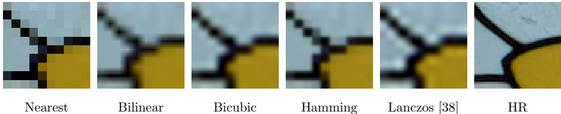
Figure 1.1: Various image interpolation methods.
