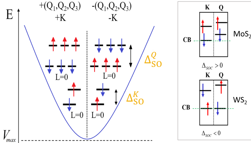
Figure 6.16: Demonstration of possible spin arrangement in different TMDC materials. (left) Spin levels for an MoS 2 QD. (right) Two possible spin band arrangements for bulk MoS 2 and WS 2 at K and at Q . Spins are aligned (anti-aligned) for MoS 2 (WS 2 ).
