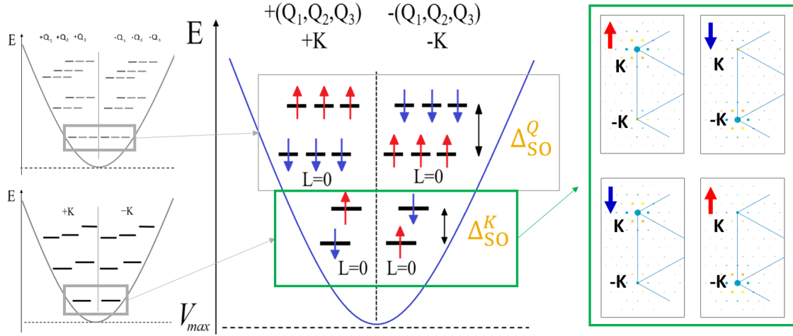
Figure 6.15: The effect of \Delta_{SO} on SP energy levels of an MoS 2 QD. The SO splitting of lowest shell (left) is shown in the middle (not to scale). Spin up and down are denoted with red and blue arrows respectively. \Delta_{SO}^K and \Delta_{SO}^Q are opposite in opposite valleys. and the same within a valley. (right) Fourier distribution of the K -derived L=0 shell (marked with green box). Each level is clearly linked to valley and spin, which allows for distinction.
