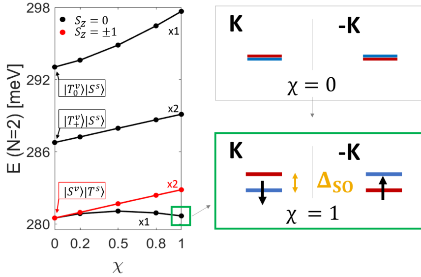
Figure 6.26: (left) Solutions of N = 2 interacting electrons in the first I = 0 shell of an Mo 2 QD with varied SO strength \chi ( \Delta_{SO} \rightarrow \chi\Delta_{SO} ). The GS becomes a mix of spin triplet |T^s\rangle and spin singlet |S^s\rangle , shown with a green box. (right,top) Energy levels for \chi = 0 . (right,bottom) GS for \chi = 1 is spin and valley unpolarised.
