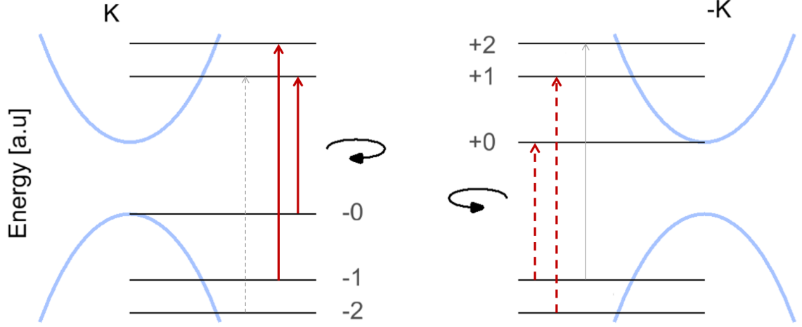
Figure 5.5: Schematic representation of the optical selection rules for mdF LLs. Thick red (thin grey) lines mark the dominant (weak) transitions allowed by Eq. 5.40. The dominant selection rules at \pm\mathbf{K} are \Delta n = \pm 1, \Delta m = 0 for \sigma^\mp (shown with solid and dashed lines respectively) and opposite polarisation for the weak transitions.
