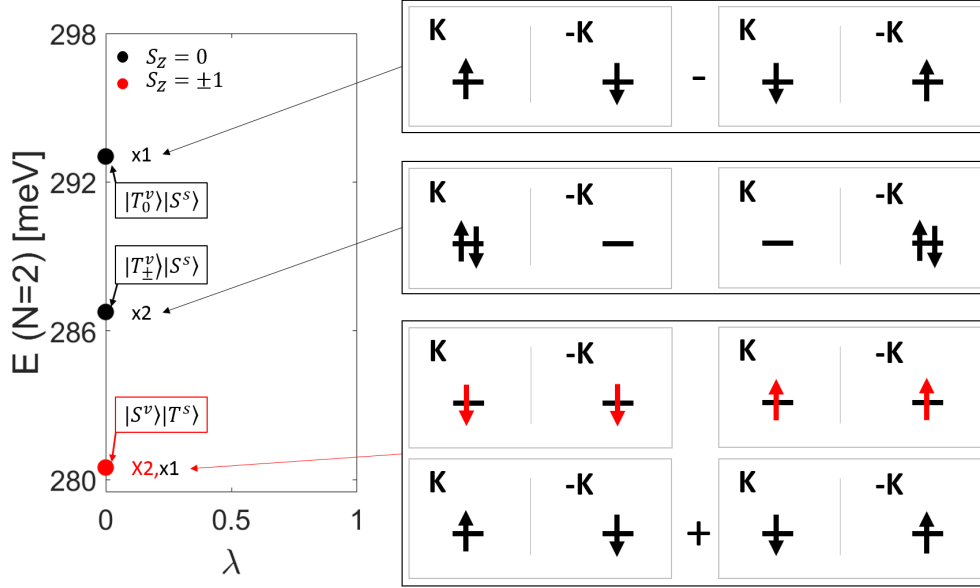
Figure 6.25: (left) Solutions of N = 2 interacting electrons in the first I = 0 shell of an Mo 2 QD with SO strength \chi = 0 ( \Delta_{SO} \rightarrow \chi \Delta_{SO} ). The GS is a spin triplet |T^s\rangle and valley singlet |S^v\rangle . Excited states are labelled analogously. (right) Eigenvectors building states in the left. Spins are shown with arrows, colors label S_z eigenstates.
