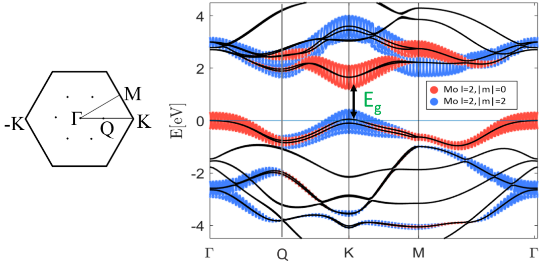
Figure 2.14: DFT band structure of MoS 2 . (left) Chosen path in the BZ. (right) Band energies for the path shown on the left. Energies are marked with black lines, while the colorful overlapping patterns depict the orbital content of bands. The thickness of the pattern encodes the amount of orbital content. Colors label Mo orbitals for m_d = 0 (red) and m_d = \pm 2 (blue). The energy band gap is shown at \mathbf{K} with a green symbol.
