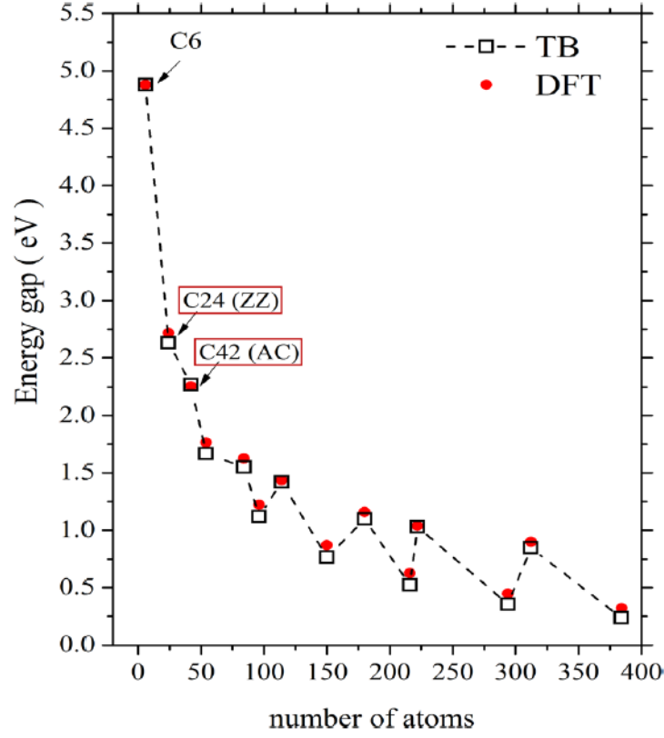
Figure 3.1: Comparison of the energy gap of GQDs obtained from NN TB model and DFT methods. The hopping element t has been fit for the first data point (benzene) and used to obtain remaining TB energy gaps.
