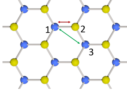
Figure 6.23: MoS 2 atomic sites included in the evaluation of Coulomb integrals. Numbers label atoms identified in integrals in Table 6.1. Red (green) arrows mark NN (NNN) integrals (rows 7,8 in the Table).
