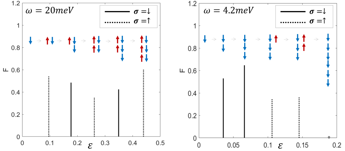
Figure 6.32: Values of F(\varepsilon) (Eq. 6.36) for two \omega regimes for N = 2 - 6 electrons. Spin up (down) shown with a dashed (solid) line and red (blue) arrows. As a consequence of the nature of the GS phase, both regimes differ by the spin sequence of peaks. Low \omega lacks the last peak (grey dot) due to spin and valley blockade.
