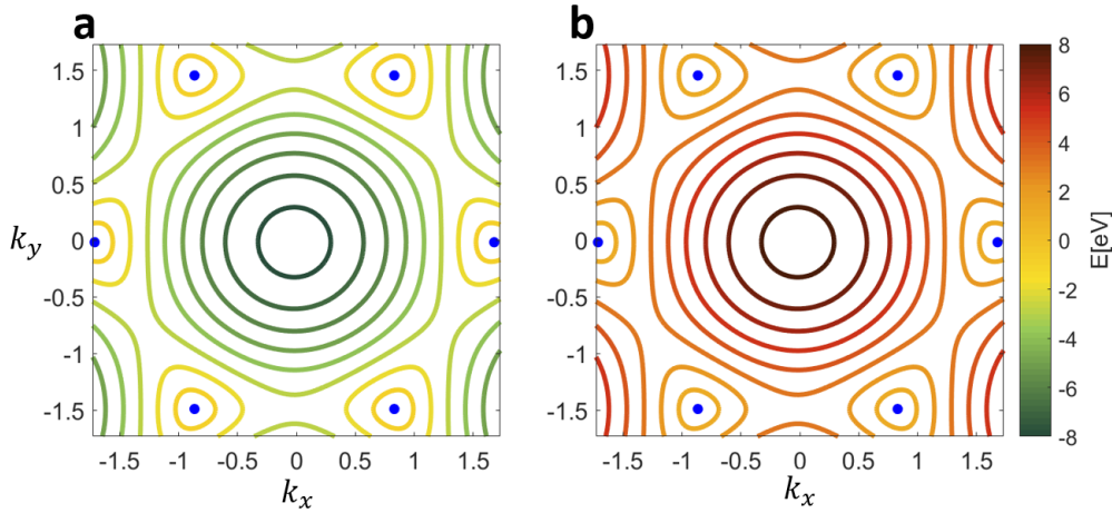
Figure 2.4: Energy dispersion of the \pi band for graphene in the NN approximation for a) VB and b) CB. Colors encode the energy. Blue dots mark the corners of the BZ \mathbf{K} & -\mathbf{K} . Mirror symmetry of both bands is apparent.
