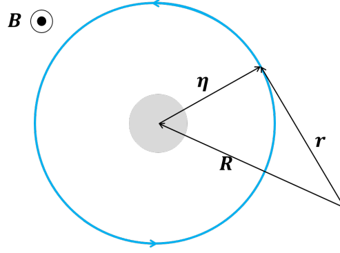
Figure 5.1: Relative cyclotron motion \boldsymbol{\eta} (blue circle) of an electron about the centre \mathbf{R} with uncertainty of the position (grey circle).
