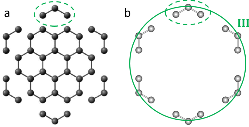
Figure 3.6: 1D Lieb lattice on the edge of an armchair-edged graphene quantum dot. a) Single cluster and b) ring of clusters.
