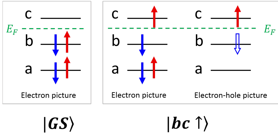
Figure 2.16: (left) GS configuration, with all levels filled with electrons (solid arrows) below the Fermi level E_F . (right) An excitation schematically drawn in the electron and electron-hole picture. In the electron picture, when an electron is promoted above the Fermi energy, an empty level is left behind. The electron-hole picture regards the empty level as a positive charge - a hole (empty arrow), which has an opposite spin to the missing electron.
