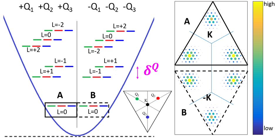
Figure 6.13: (left) QD energy levels associated with \mathbf{Q} -points (not to scale). For each valley there are three \mathbf{Q} -points (red, blue and green in inset and corresponding energy levels), which produce threefold degenerate spectrum for each valley. Topological splitting \delta^{\mathbf{Q}} is larger than \delta^{\mathbf{K}} . (right) \mathbf{k} -point distribution for lowest 6 states (groups A and B) shows localisation at \mathbf{Q} -points.
