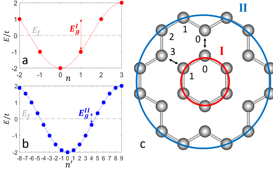
Figure 3.3: Energy spectrum (in the units of t ) of ring a) I and b) II. The size of the ring determines the number of states n, n' . Energy gap of each ring E_g^I, E_g^{II} is marked. Fermi level is marked with E_f . c) Coupling rule for both rings (see text for details).
