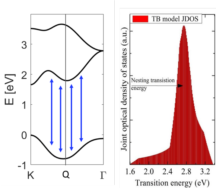
Figure 4.6: (left) The bands around the \mathbf{Q} -point are approximately parallel, which causes band nesting. The nesting transition energy (blue arrow) around \mathbf{Q} is the most common through BZ, which causes the joint optical density of states to peak in the right panel. (right) Joint optical density of states in \text{MoS}_2 . Peak at \approx 2.8 eV corresponds to the nesting transition energy in the left panel.
