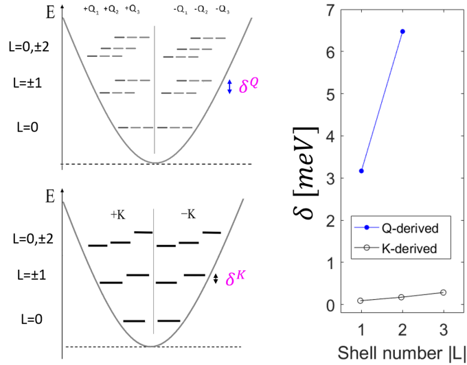
Figure 6.14: (left) Topological splitting \delta for \mathbf{K} -derived and \mathbf{Q} -derived states (identified on the bottom and top of left panel, not to scale). (right) Magnitude of \delta^{\mathbf{K}} and \delta^{\mathbf{Q}} shown for different shells with black empty and blue solid dots. \delta^{\mathbf{Q}} is an order of magnitude larger than \delta^{\mathbf{K}} and reaches up to 6.5 meV.
